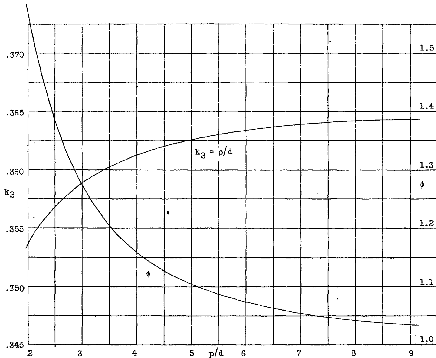
Figure A-1.-- Values of \phi and k_2 for corrugated sheet.
