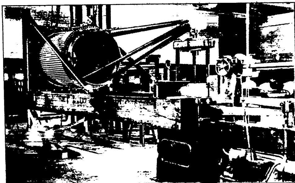
Figure 7.- Cylinder 1 in jig ready for test.
