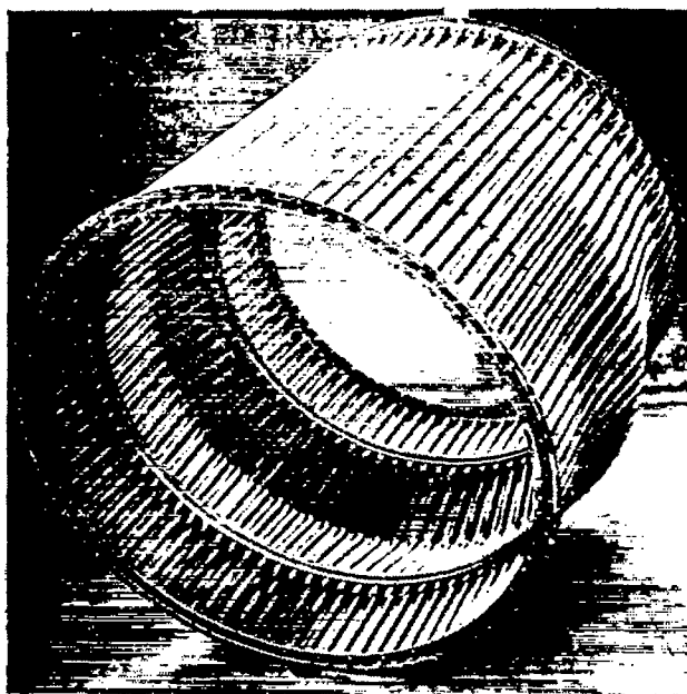
Figure 3.- Failure of cylinder 1.
