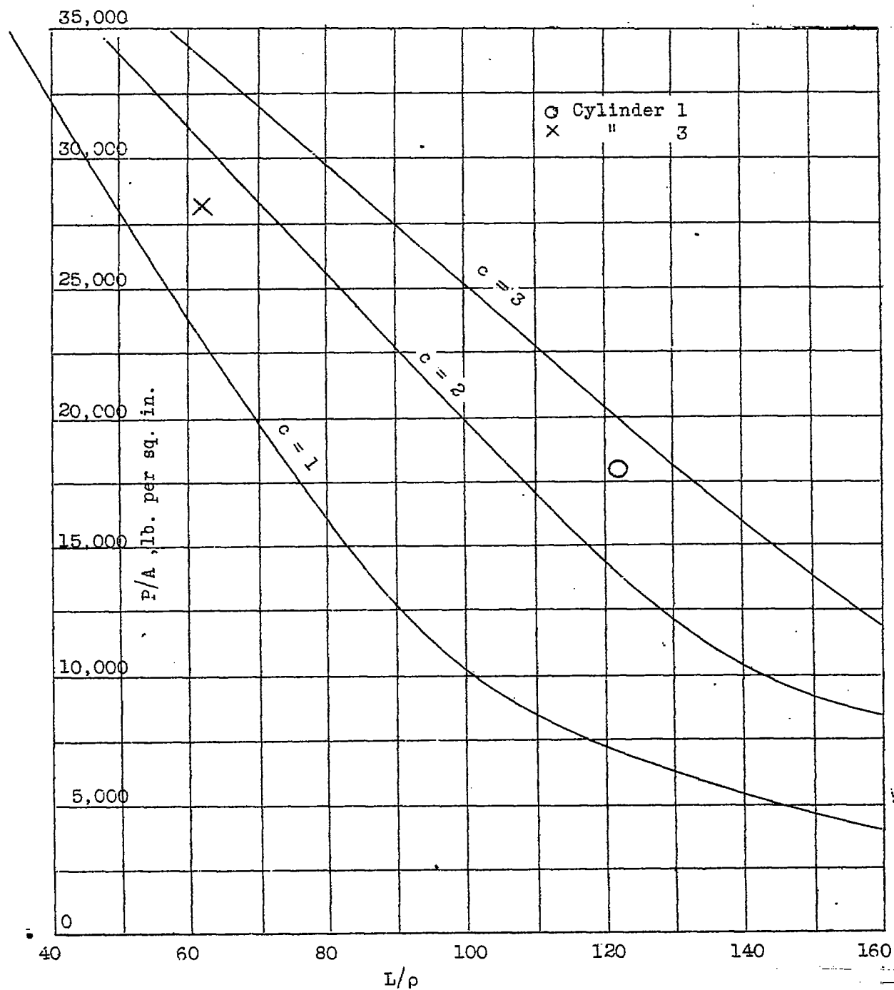
Figure 9.- Relation between column curve and observed stresses at failure.
