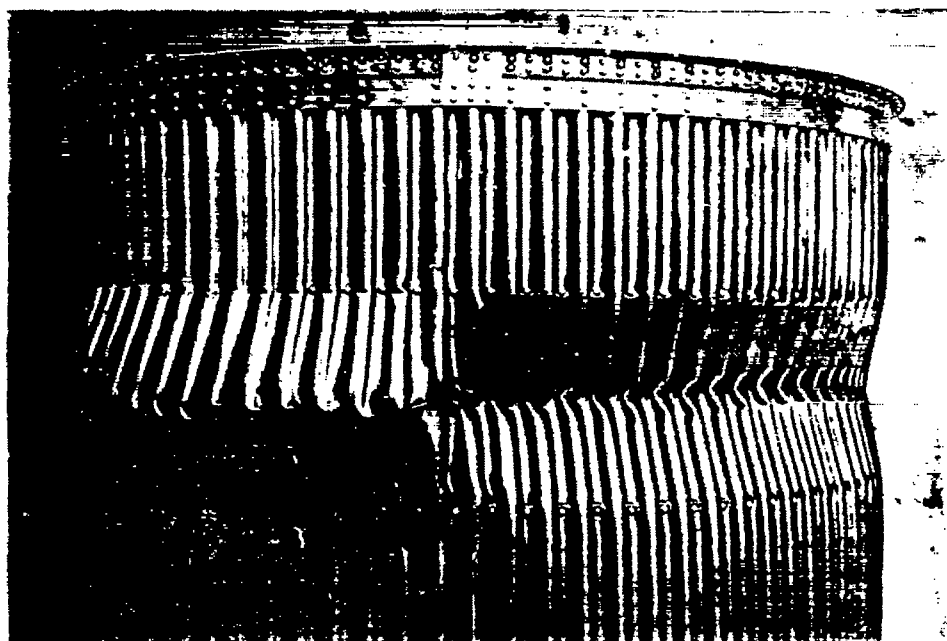
Figure 4.- Failure of cylinder 3.
