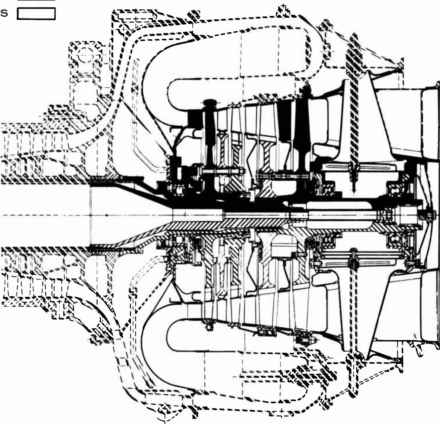
T53-L-13 ENGINE (DESIGN CHANGES AS COMPARED TO T53-L-11)
