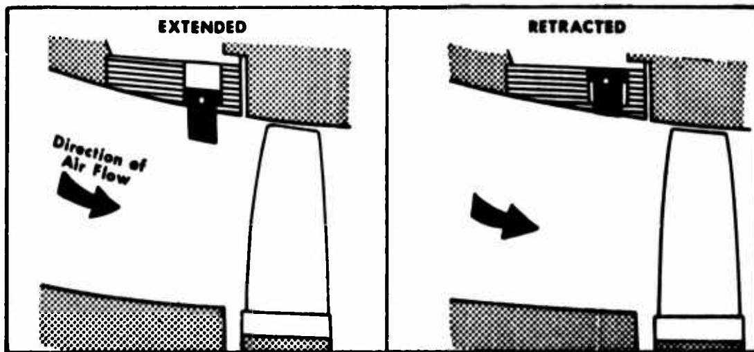
FIG. 3 , COMRESSOR INLET FLOW FENCE
