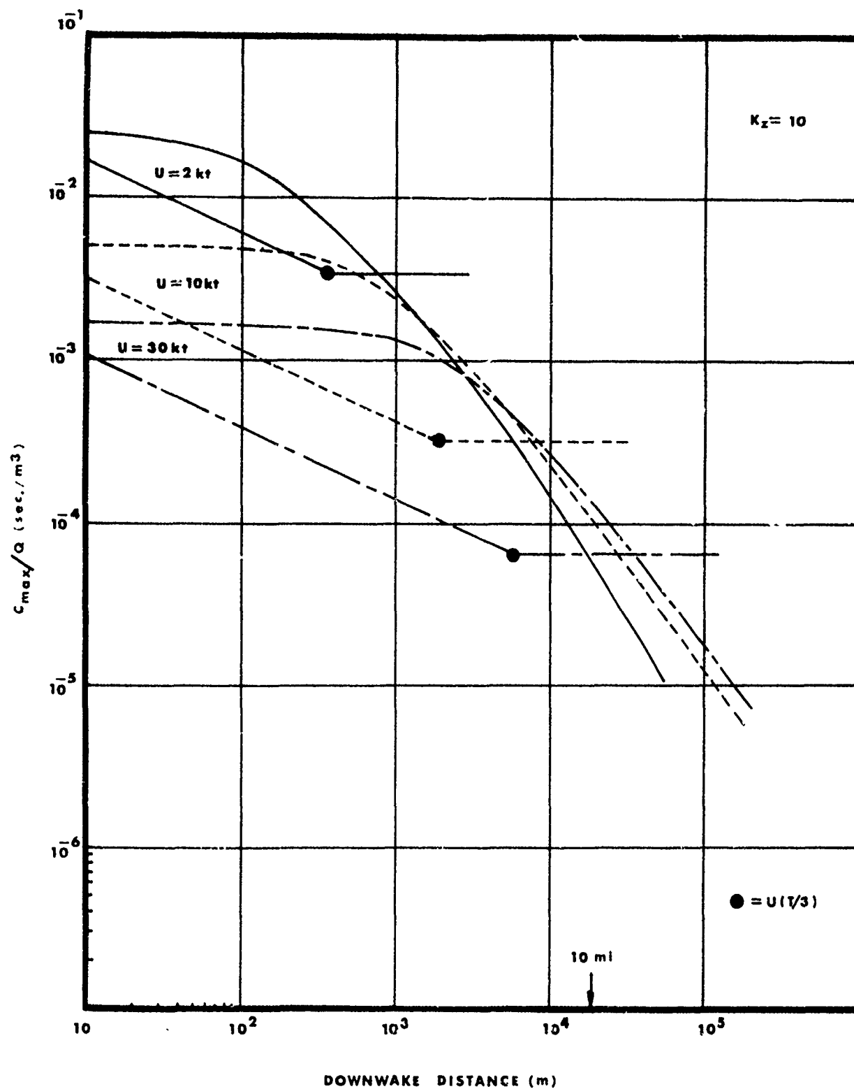
Figure 5. Maximum Contaminant Concentration vs. Downwake Distance for a Submarine Wake with T = 18 \text{ min} and for a Naturally Dispersing Volume Source with K_z = 10 \text{ cm}^2/\text{sec} at Three Speeds.
