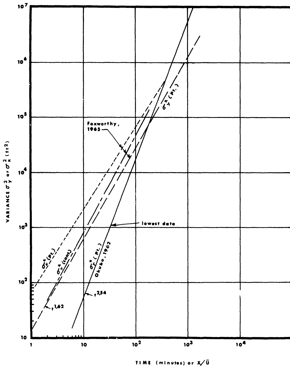
Figure 3. Size Variance of Naturally Dispersing Point Instantaneous and Continuous Dye Tracer Releases vs. Time or X/\bar{U} for Continuous Plume.
