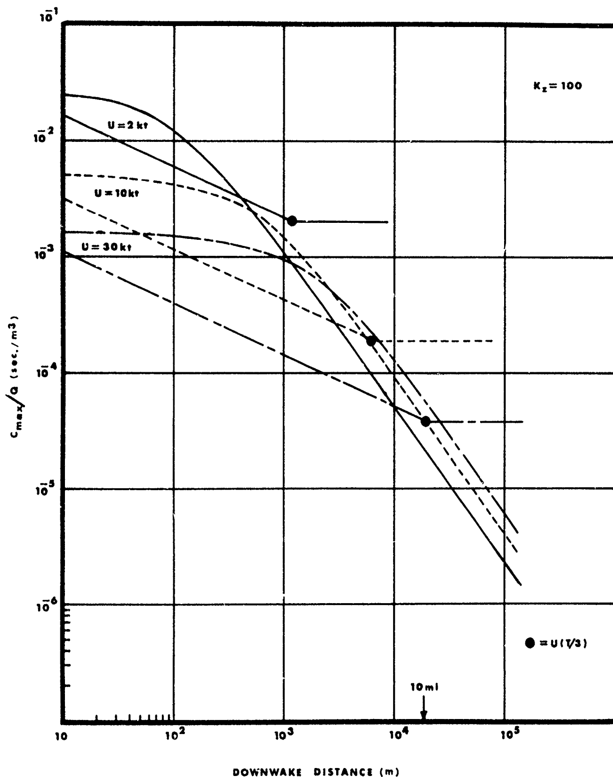
Figure 6. Maximum Contaminant Concentration vs. Downwake Distance for a Submarine Wake with T = 60 min and for a Naturally Dispersing Volume Source with K_z = 100 \text{ cm}^2/\text{sec} at Three Speeds.
