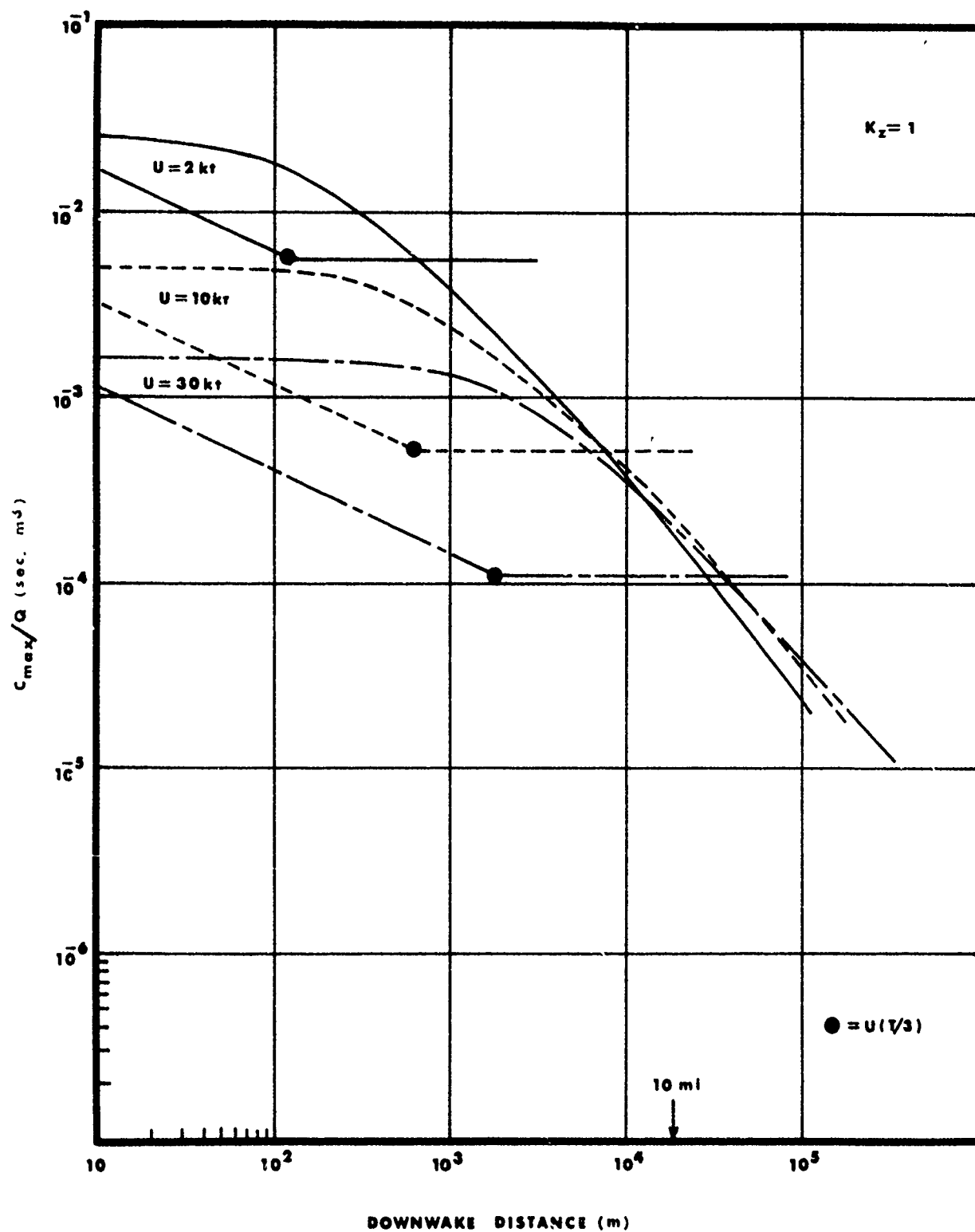
Figure 4. Maximum Contaminant Concentration vs. Downwake Distance for a Submarine Wake with T = 6 min and for a Naturally Dispersing Volume Source with K_z = 1 cm 2 /sec at Three Speeds.
