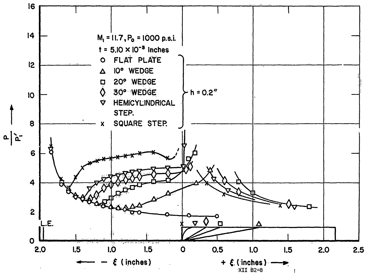
Figure 11c. Pressure distribution on a flat plate and afterbody at M = 11.7, t = 5.1 \times 10^{-3} \text{ inches}
