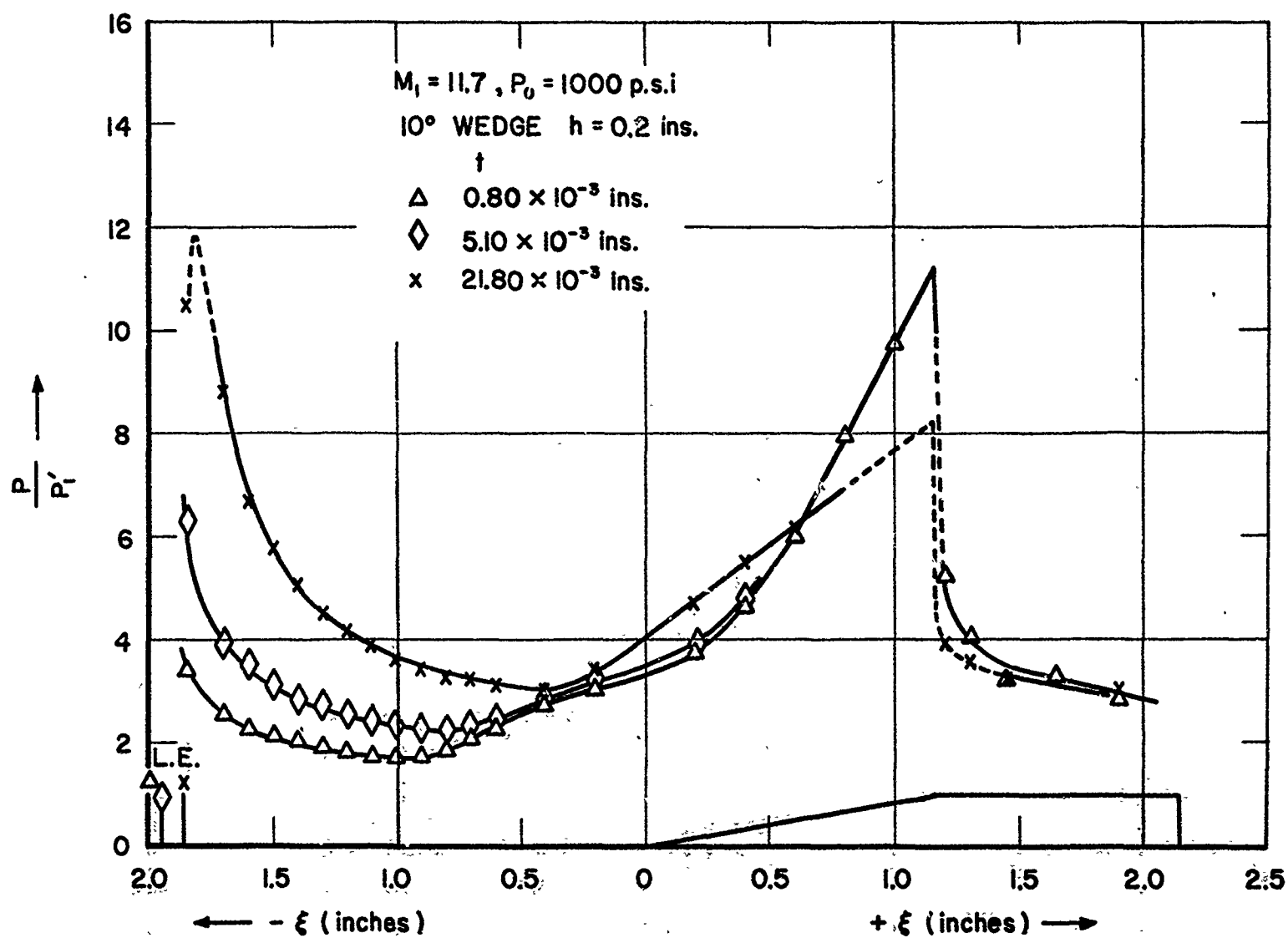
Figure 12a. Pressure-distribution on a flat plate and afterbody at M_1 = 11.7, 10^\circ \text{ wedge}
