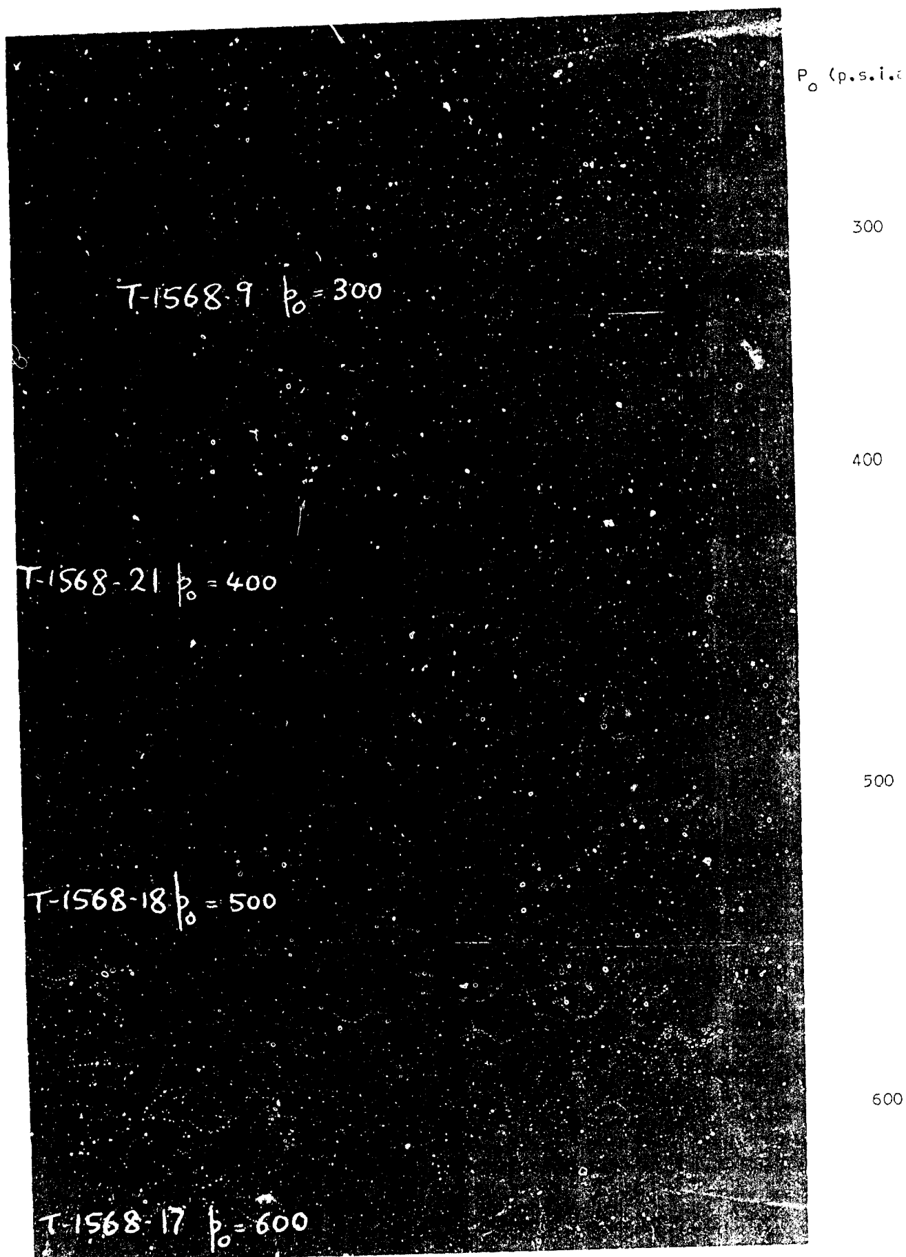
Schlieren photographs of 1\frac{1}{4}'' \times \frac{3}{32}'' cavity model at various stagnation pressures; T_0 = 535^\circ\text{R} .
