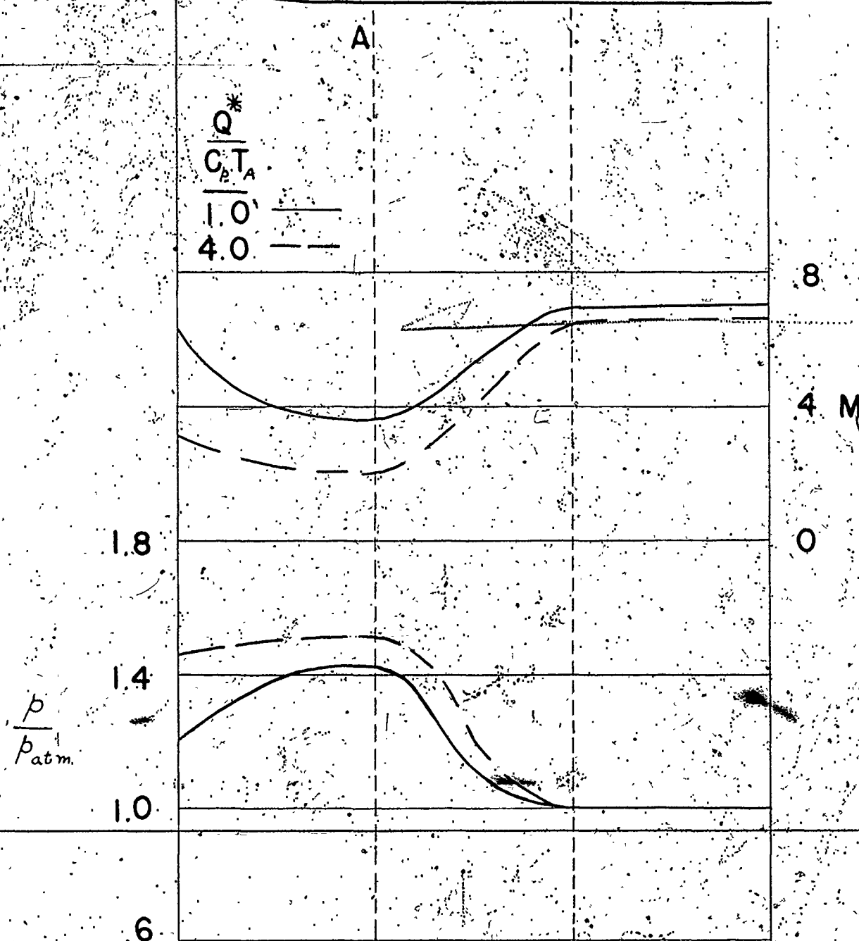
FIGURE 4 THE STEADY FLOW OBTAINED IN AN INITIALLY SUBSONIC FLOW FOR SEVERAL VALUES OF THE QUANTITY OF HEAT ADDED.
