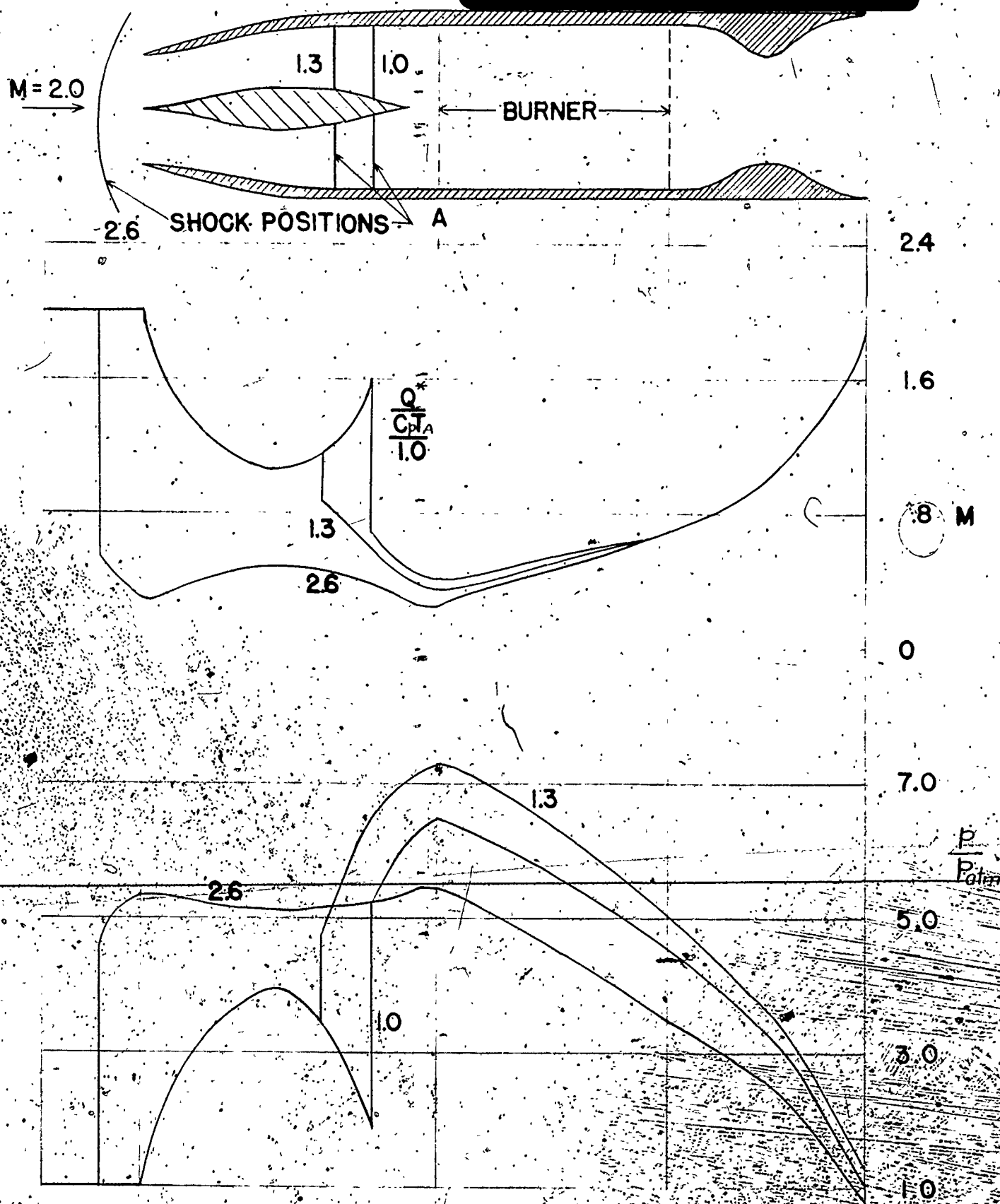
FIGURE 5 THE STEADY FLOW OBTAINED IN AN INITIALLY SUPERSONIC FLOW FOR SEVERAL VALUES OF QUANTITY OF HEAT ADDED.
