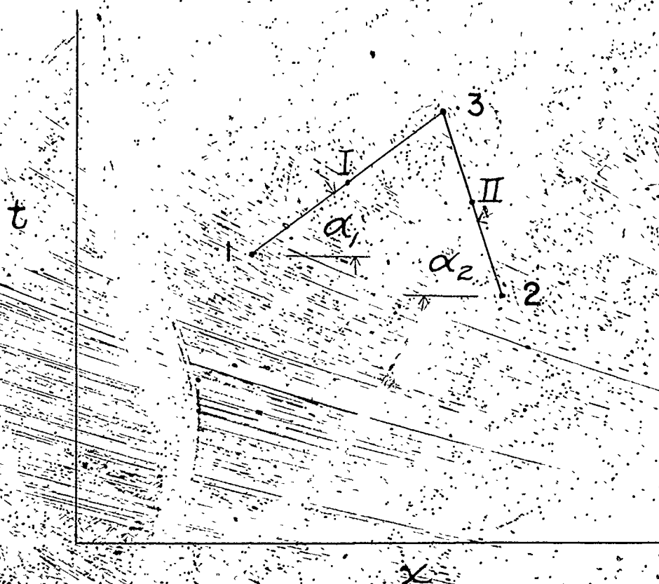
FIG. 6. GRAPHICAL METHOD OF CONSTRUCTING CHARACTERISTICS
