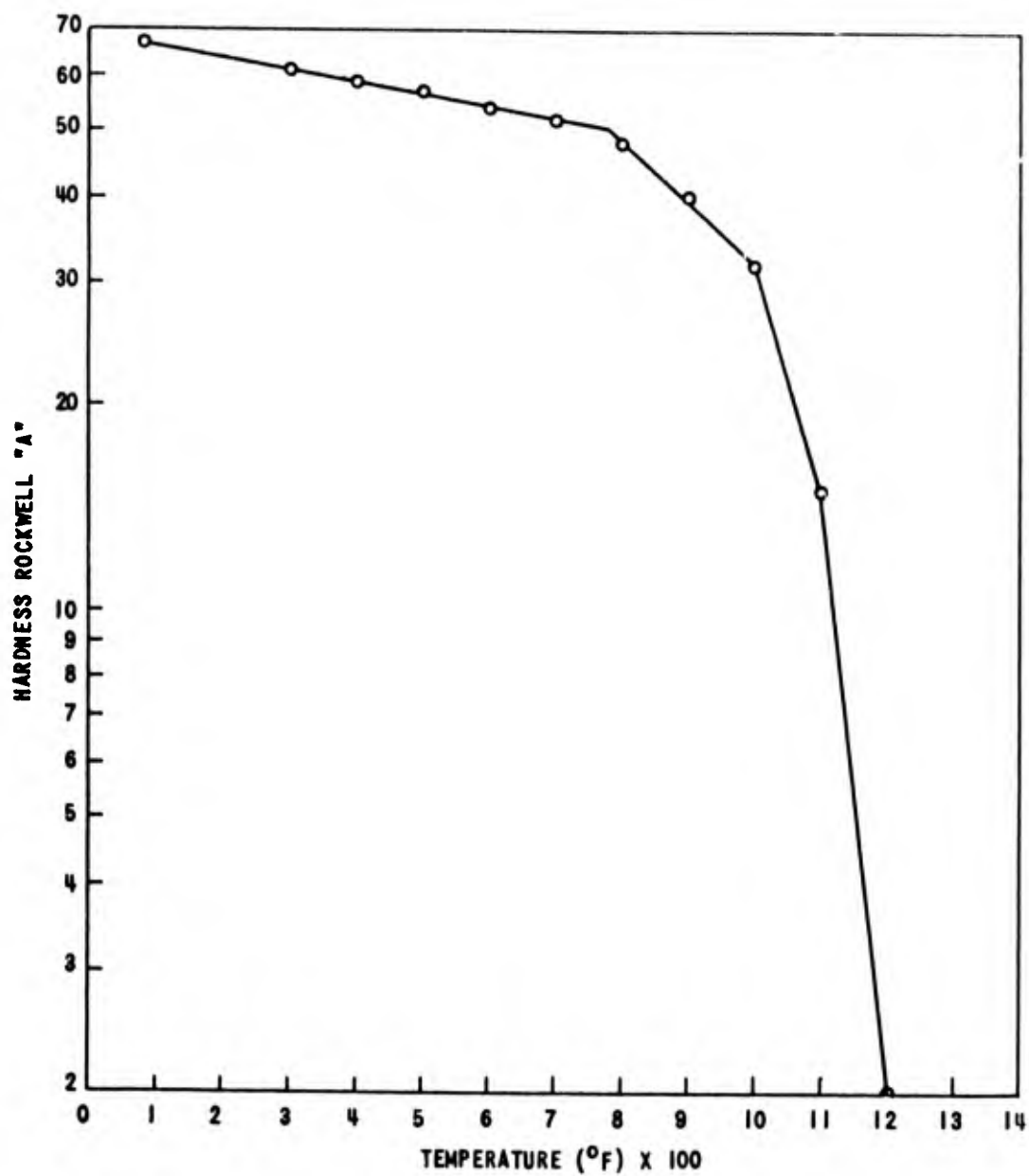
EFFECT OF TEMPERATURE ON THE HARDNESS OF Ti150A (TH1J2)
