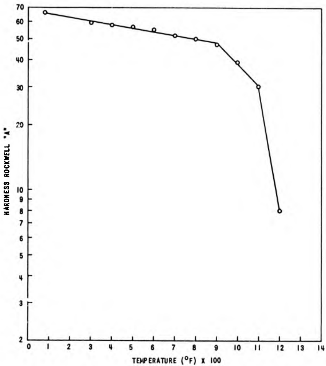
EFFECT OF TEMPERATURE ON THE HARDNESS OF C110M (RXG5)
