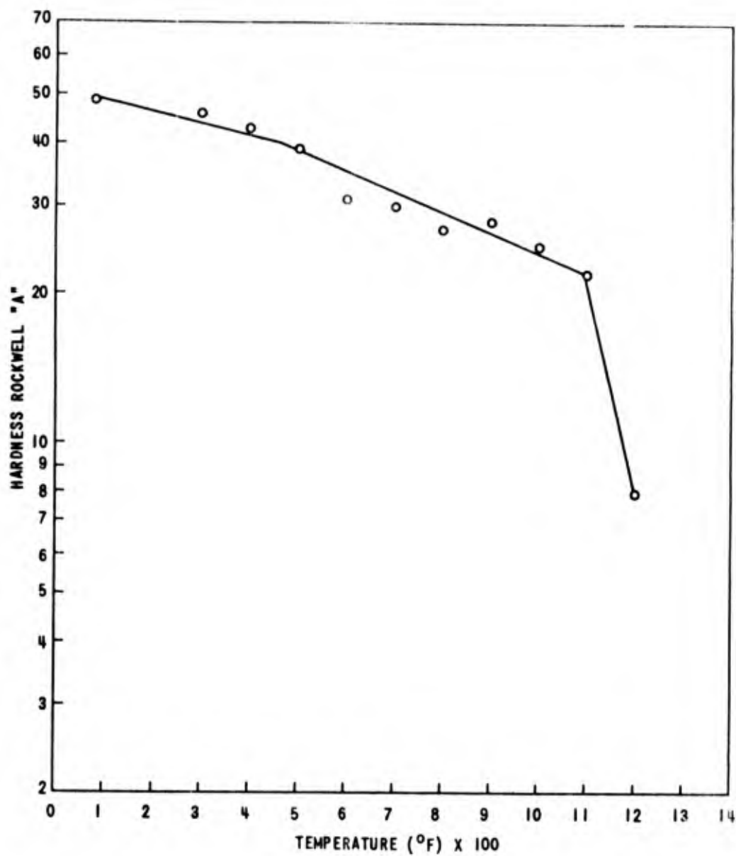
EFFECT OF TEMPERATURE ON THE HARDNESS OF Ti-0Zr (TZI)
