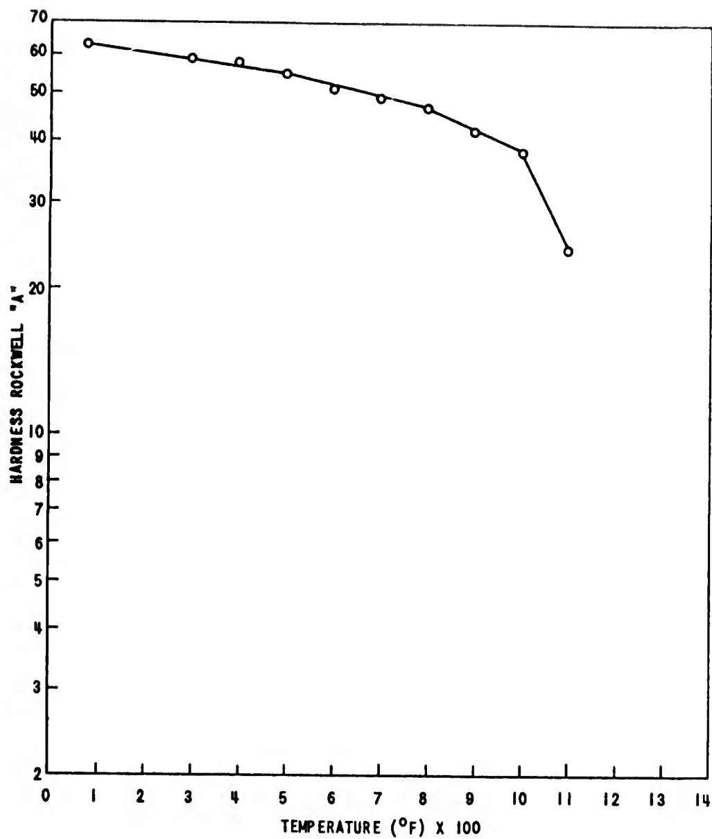
EFFECT OF TEMPERATURE ON THE HARDNESS OF Ti-3.8Cr-1.5Fe (RS14)
