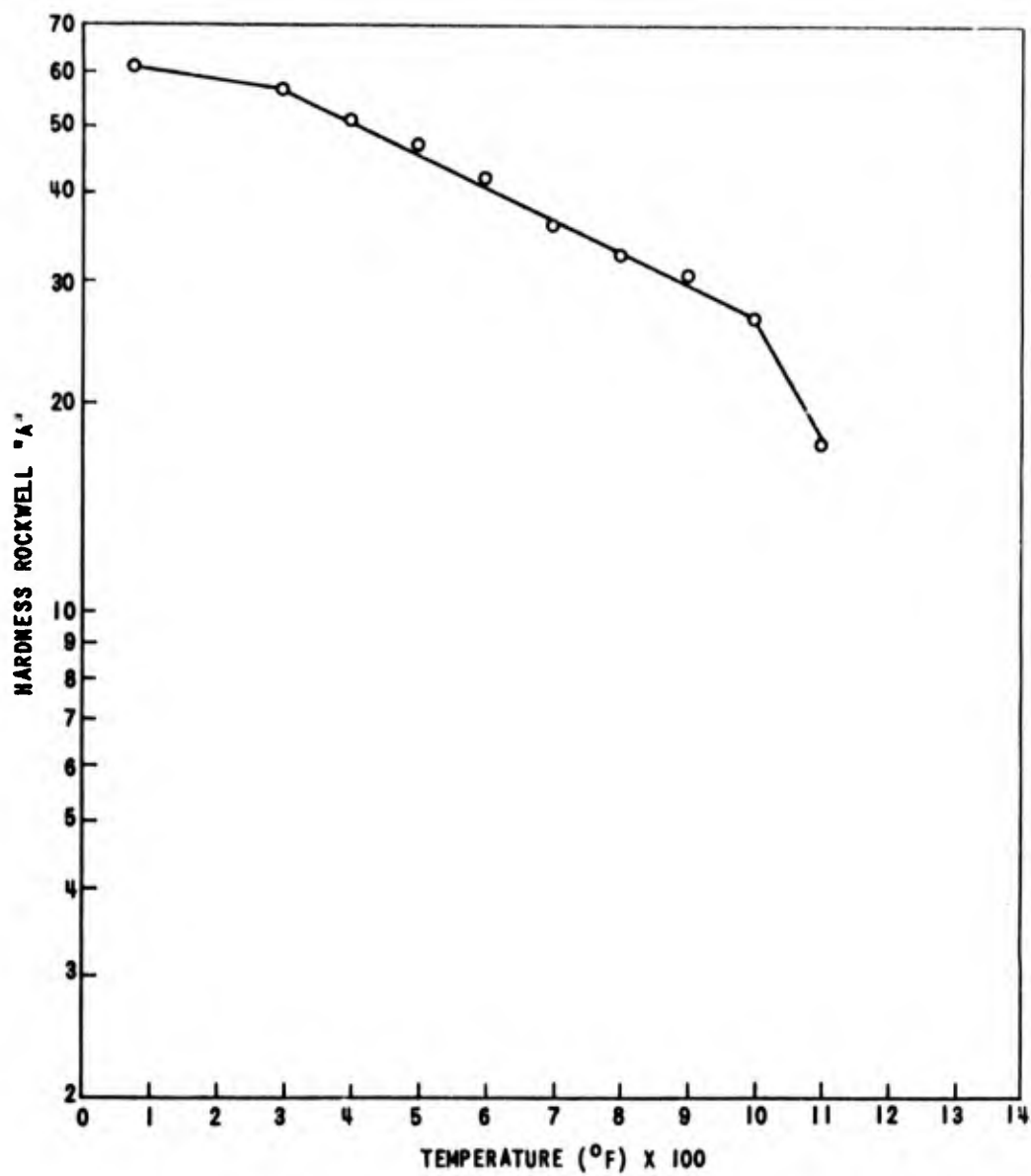
EFFECT OF TEMPERATURE ON THE HARDNESS OF RC70 (RHIDI)
