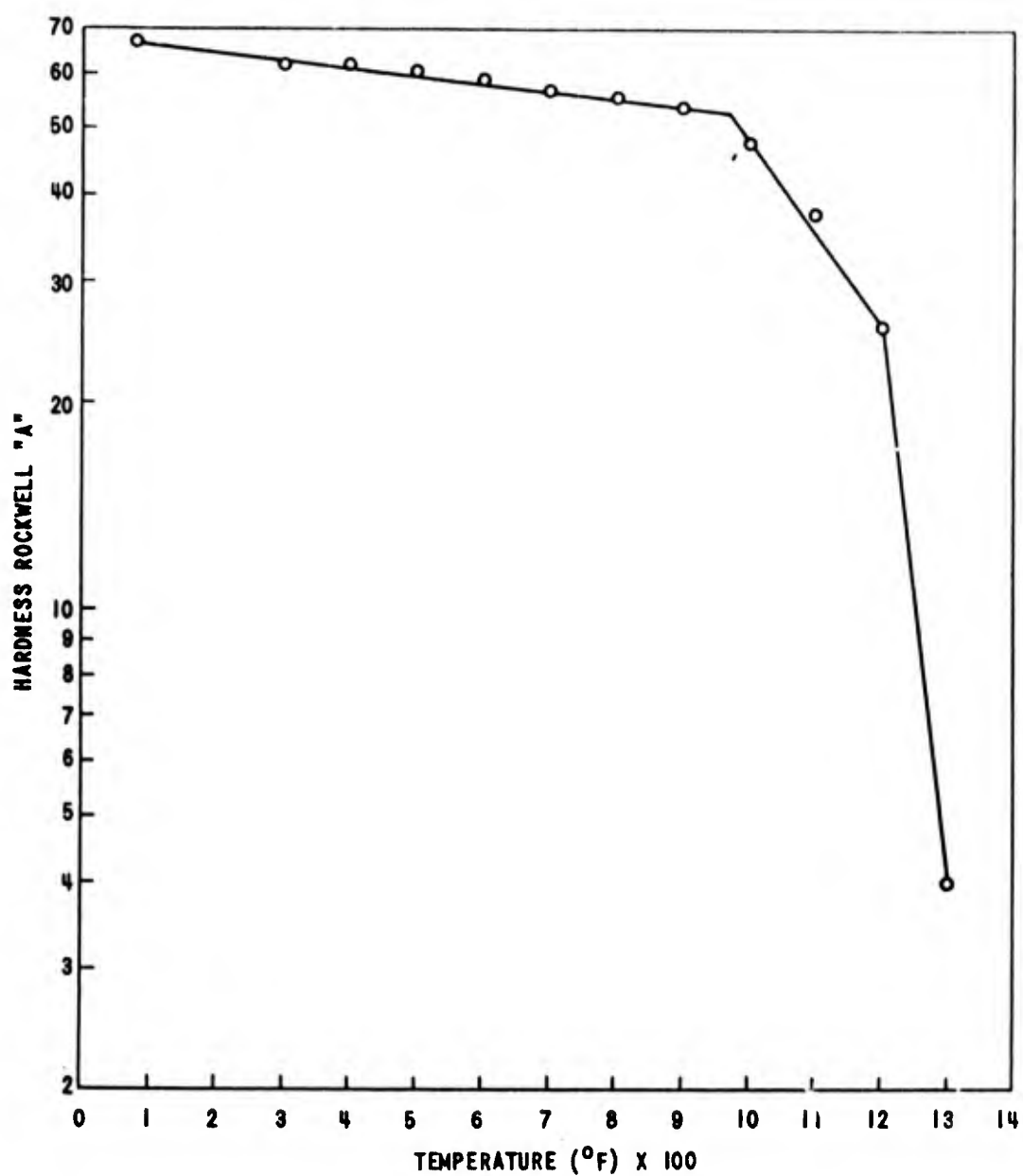
EFFECT OF TEMPERATURE ON THE HARDNESS OF C130AM (RH1B2)
