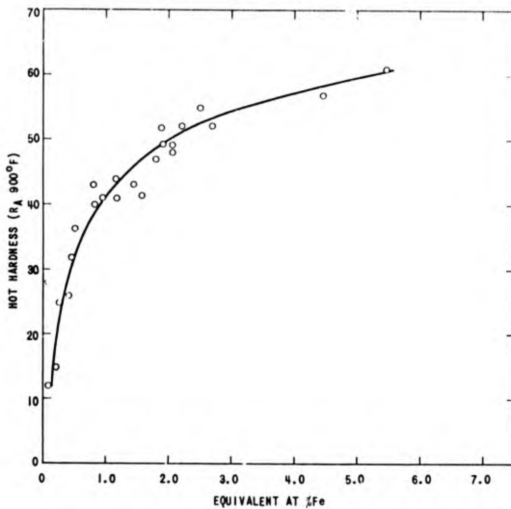
EFFECT OF CHEMICAL COMPOSITION ON THE HOT HARDNESS OF TITANIUM AT 900°F
