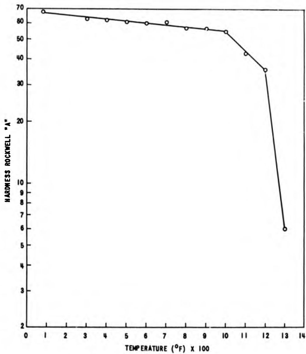
EFFECT OF TEMPERATURE ON THE HARDNESS OF Ti150B (TH15)
