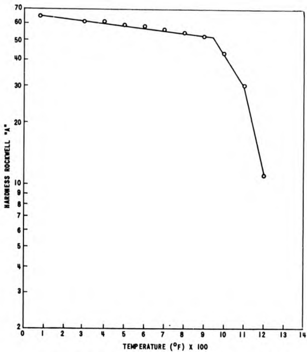
EFFECT OF TEMPERATURE ON THE HARDNESS OF CI10M (RJ1A2)
