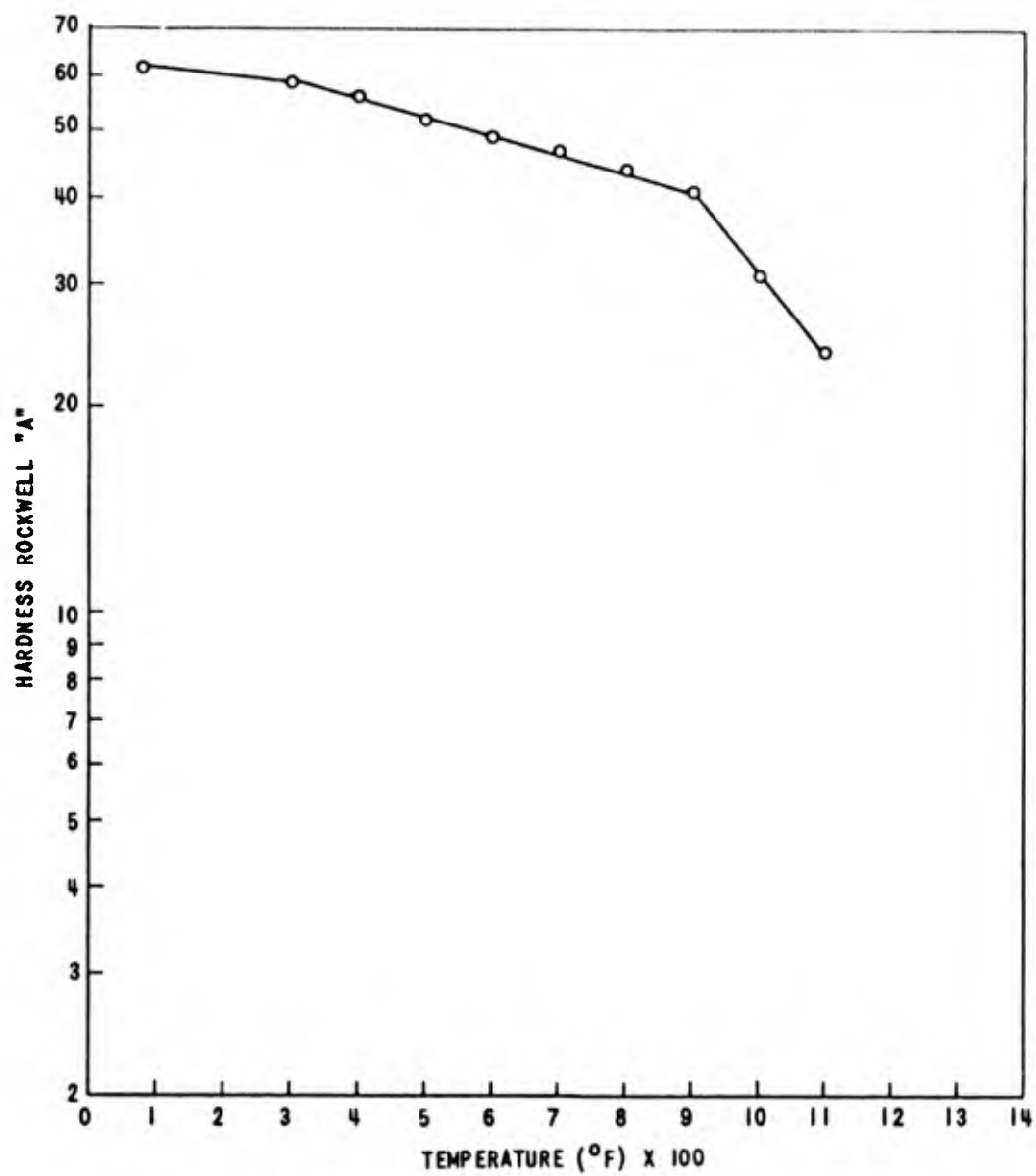
EFFECT OF TEMPERATURE ON THE HARDNESS OF Ti-3.4Al-1.5Sn (R26)
