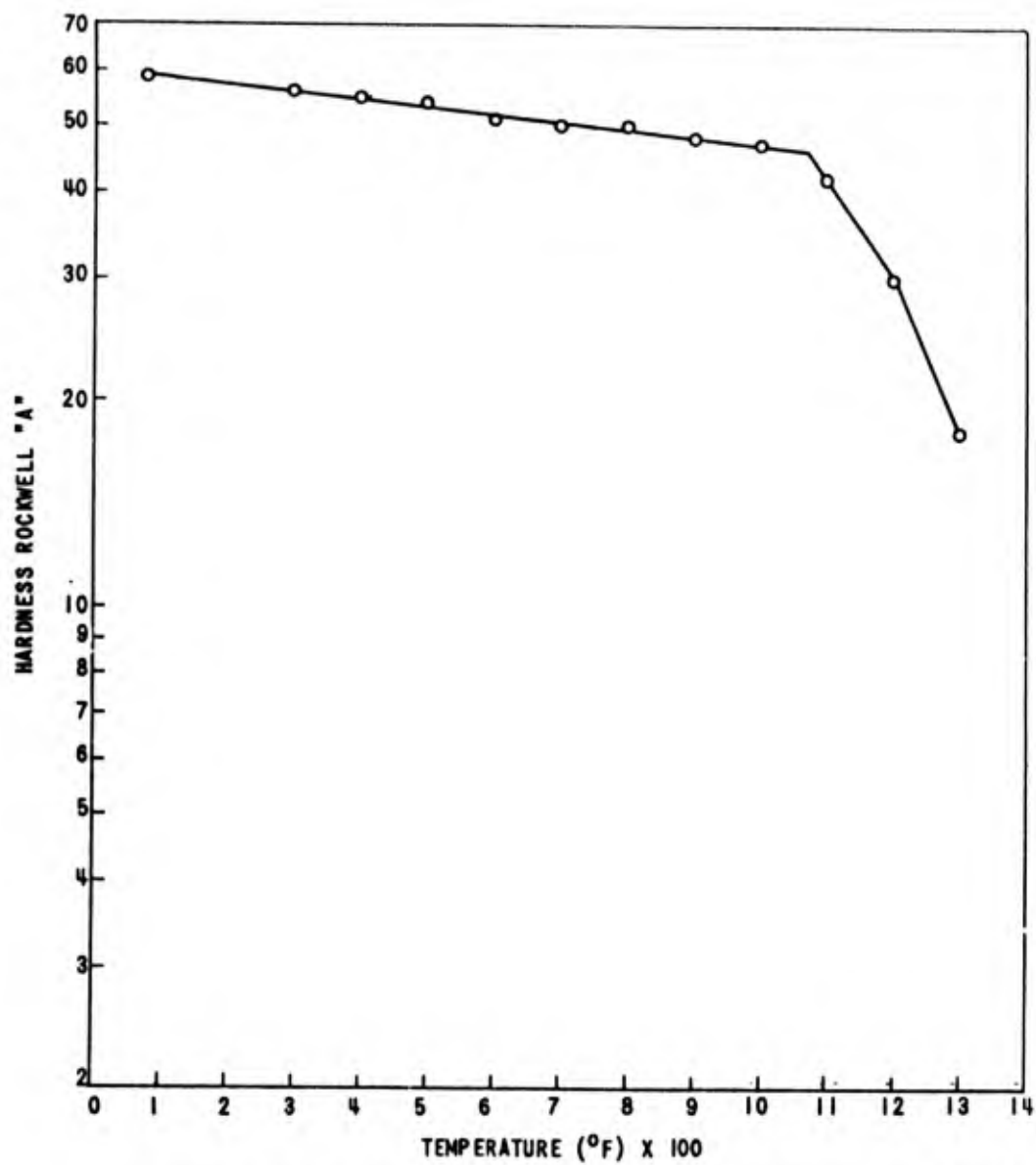
EFFECT OF TEMPERATURE ON THE HARDNESS OF Ti-24.9Zr (TZ5)
