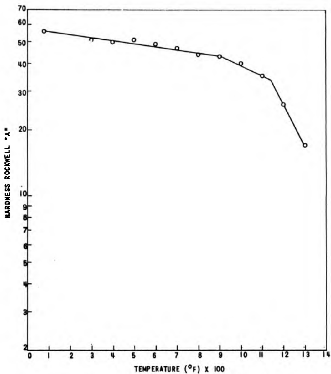
EFFECT OF TEMPERATURE ON THE HARDNESS OF Ti-5Zr (TZ2)
