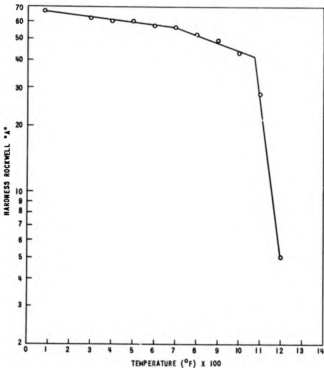
EFFECT OF TEMPERATURE ON THE HARDNESS OF C110M (RHIG5)
