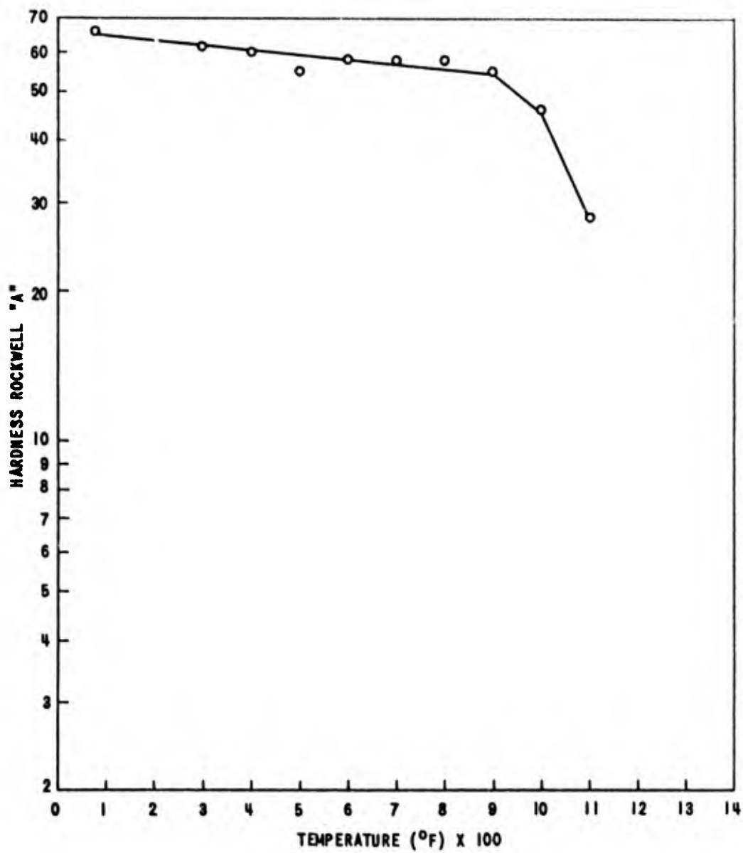
EFFECT OF TEMPERATURE ON THE HARDNESS OF Ti-6.8Mn-4.3Mo-3.9Cr (R110)
