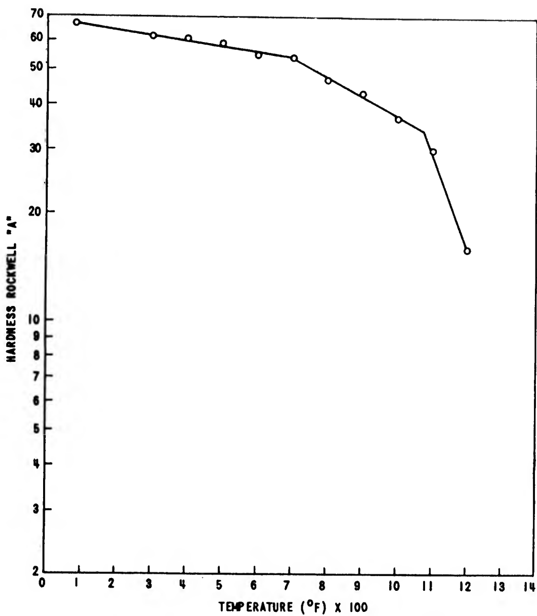
EFFECT OF TEMPERATURE ON THE HARDNESS OF Ti150A (TXF2)
