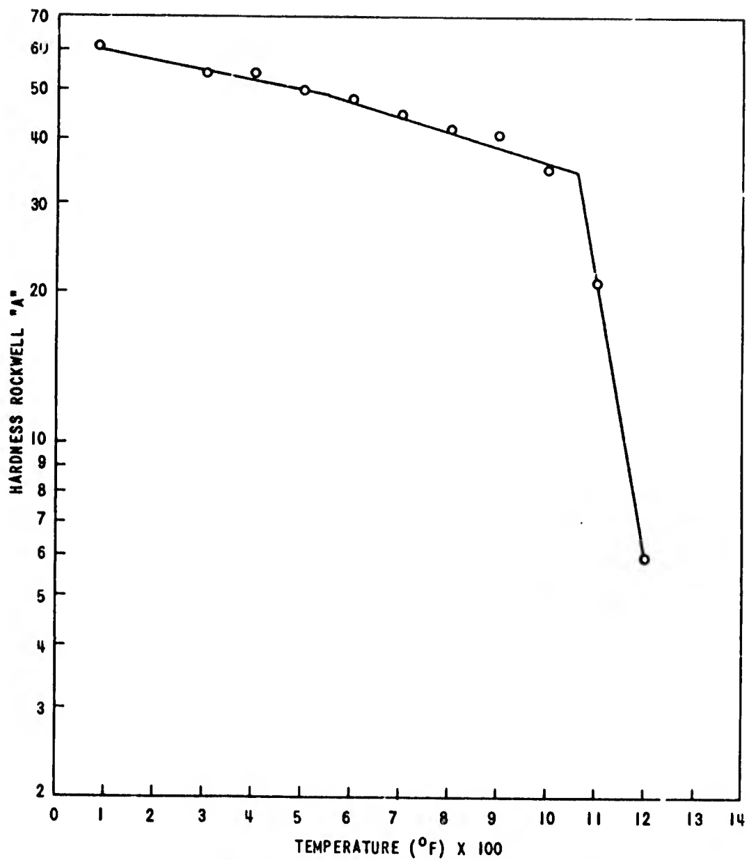
EFFECT OF TEMPERATURE ON THE HARDNESS OF Ti-4Mn (SXE4)
