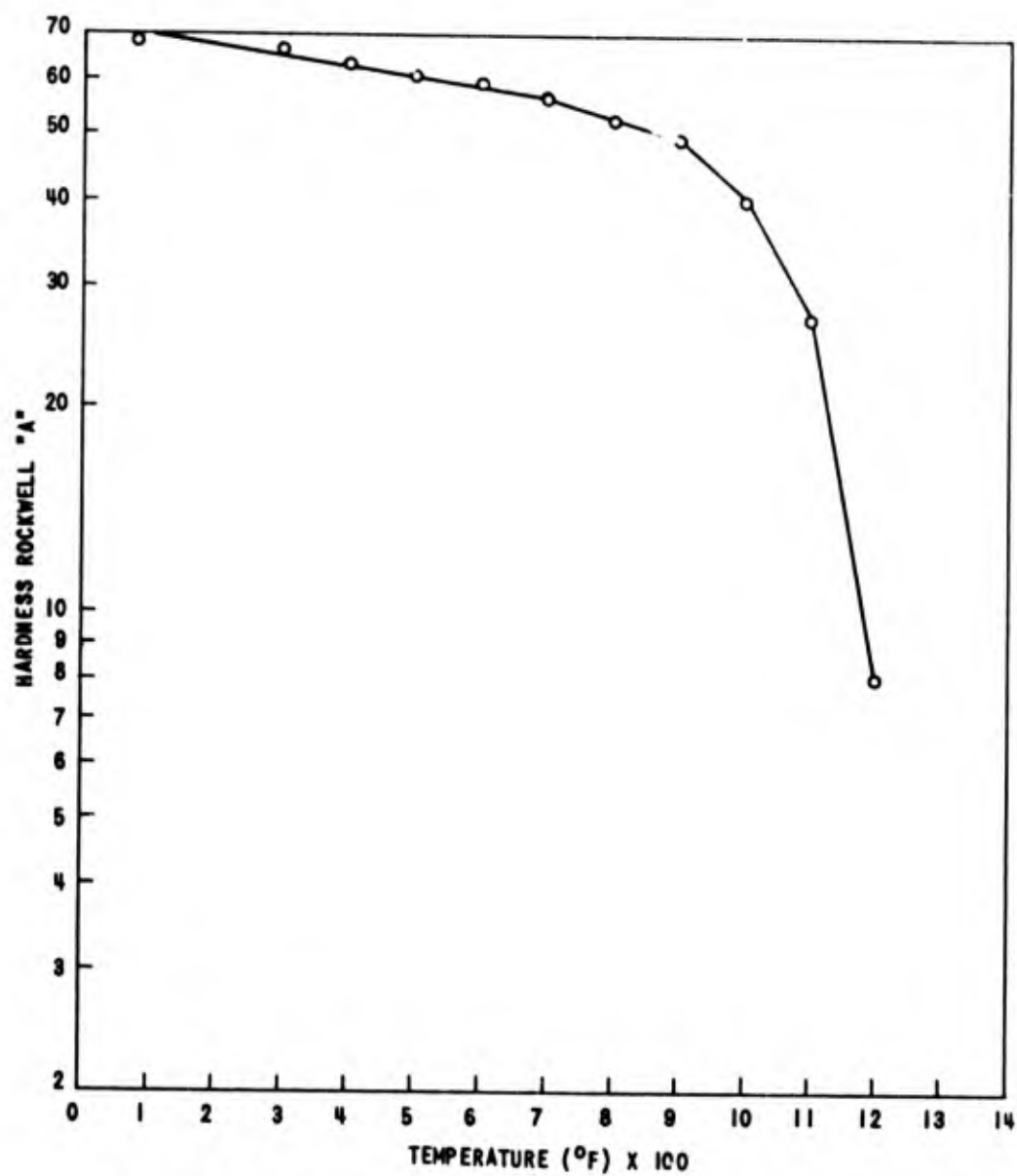
EFFECT OF TEMPERATURE ON THE HARDNESS OF C110M (RH1E2)
