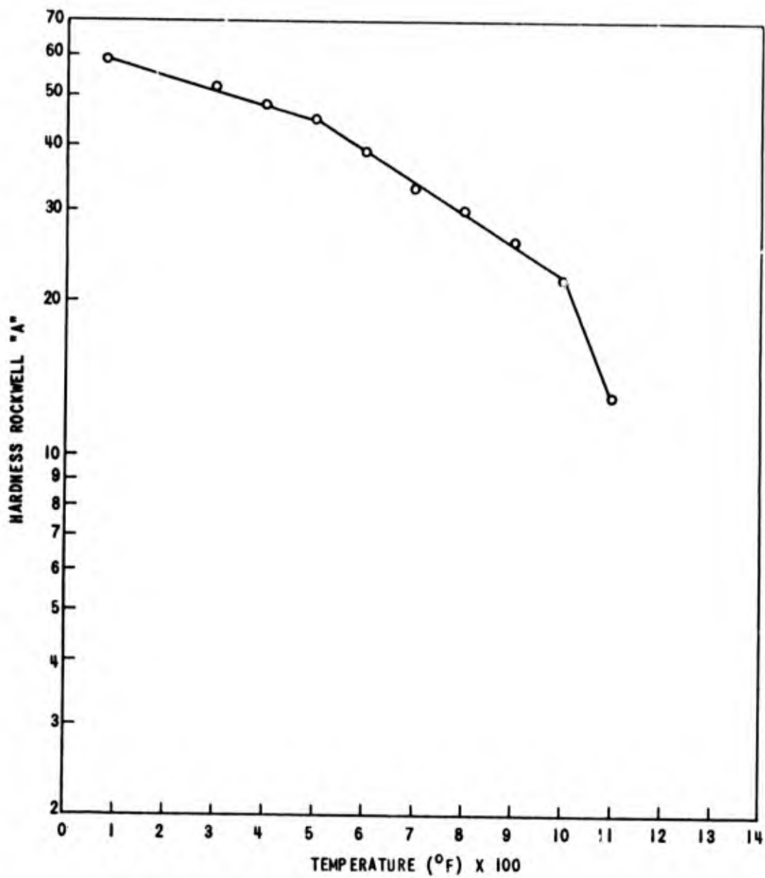
EFFECT OF TEMPERATURE ON THE HARDNESS OF Ti100A (THIG2)
