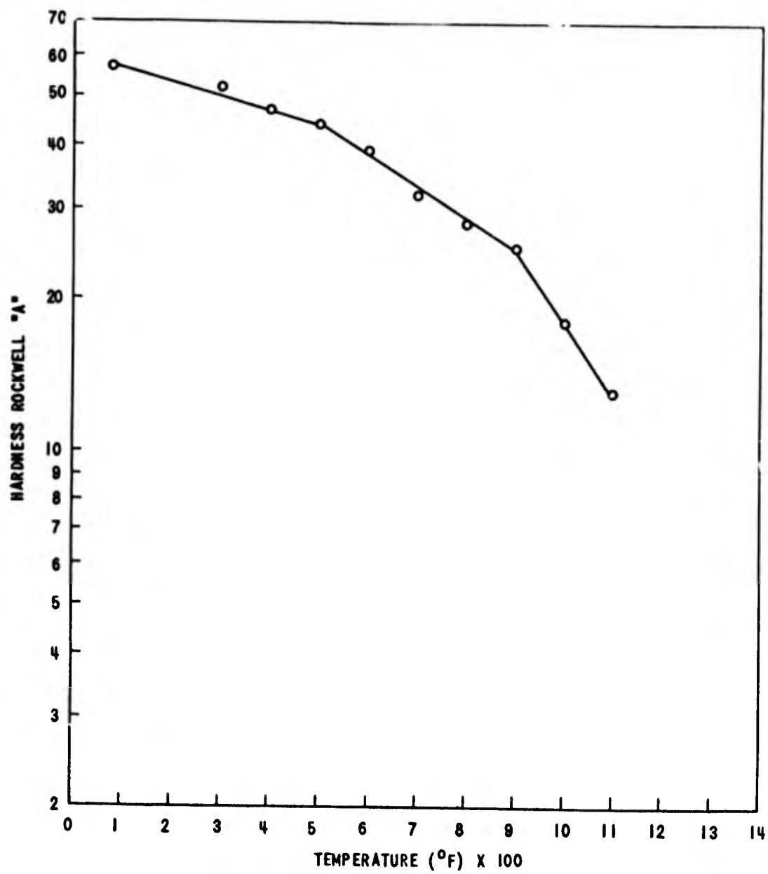
EFFECT OF TEMPERATURE ON THE HARDNESS OF A55 (TH1F2)
