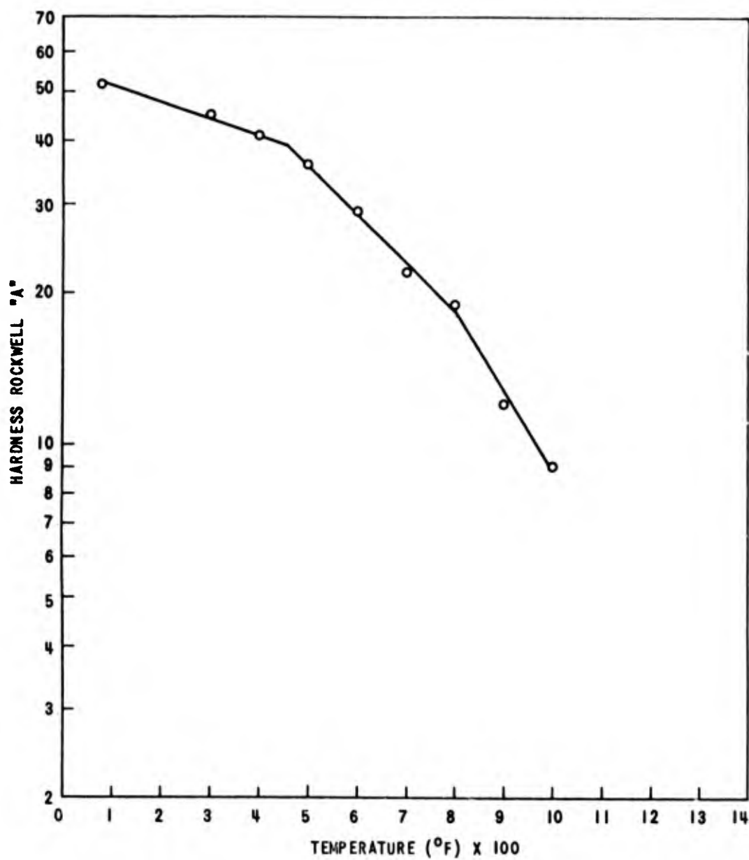
EFFECT OF TEMPERATURE ON THE HARDNESS OF RS55(SXA7)
