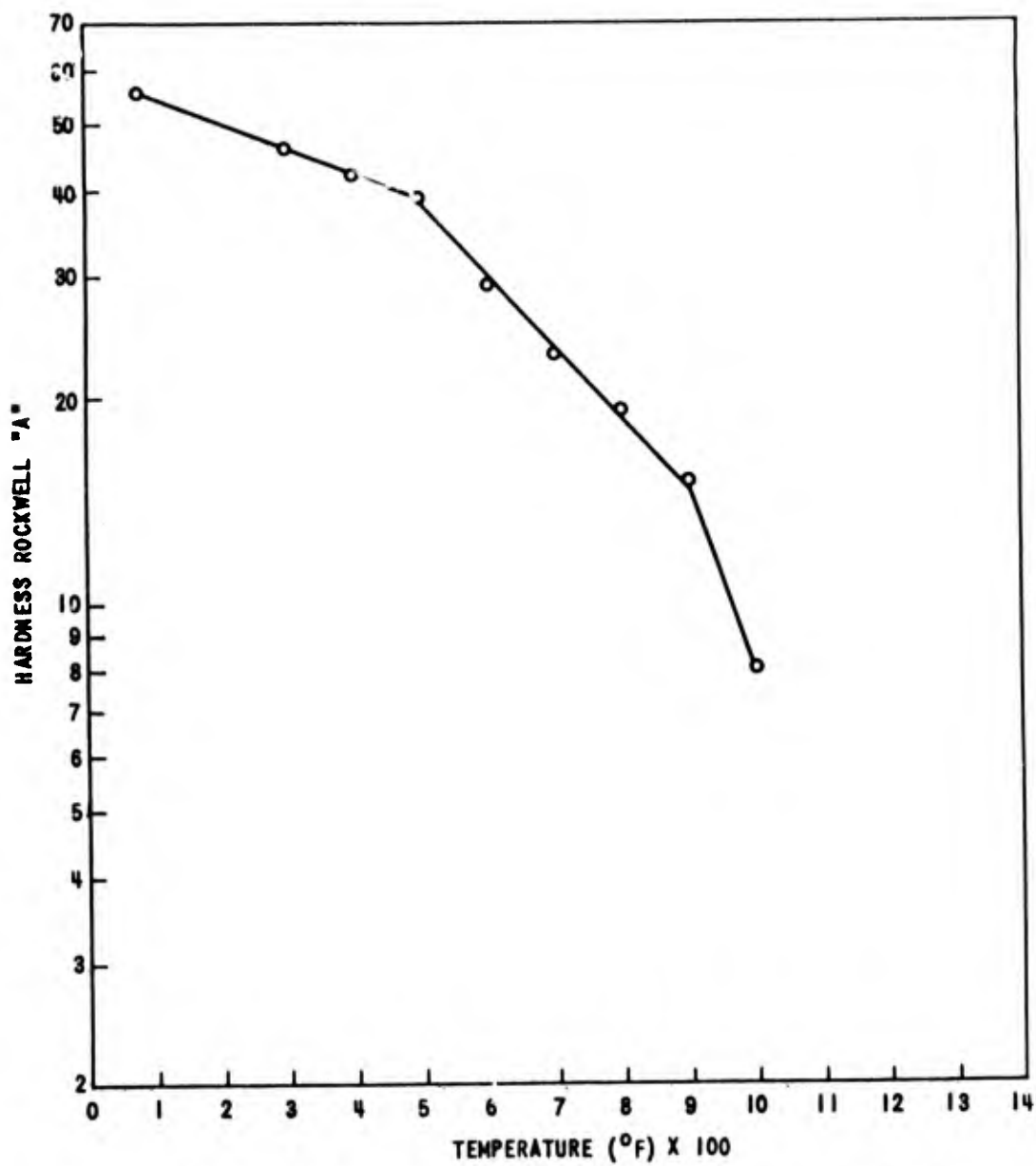
EFFECT OF TEMPERATURE ON THE HARDNESS OF A55 (RHIG4)
