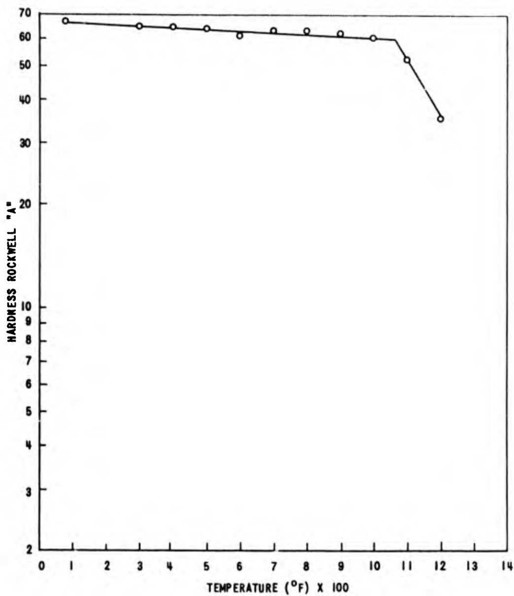
EFFECT OF TEMPERATURE ON THE HARDNESS OF Ti-5.4Fe-11.8Cr (K100)
