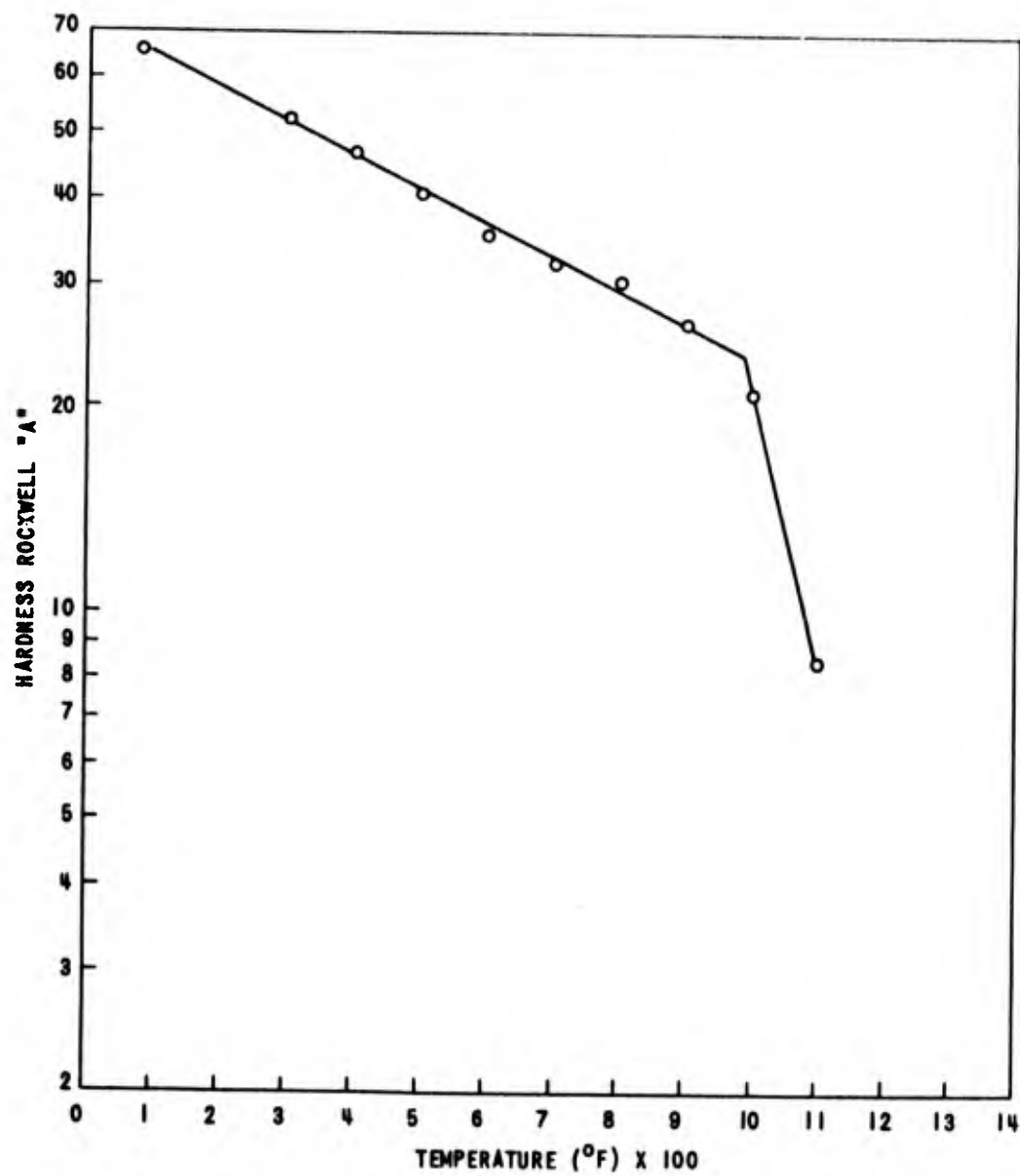
EFFECT OF TEMPERATURE ON THE HARDNESS OF A55 (RH1C1)
