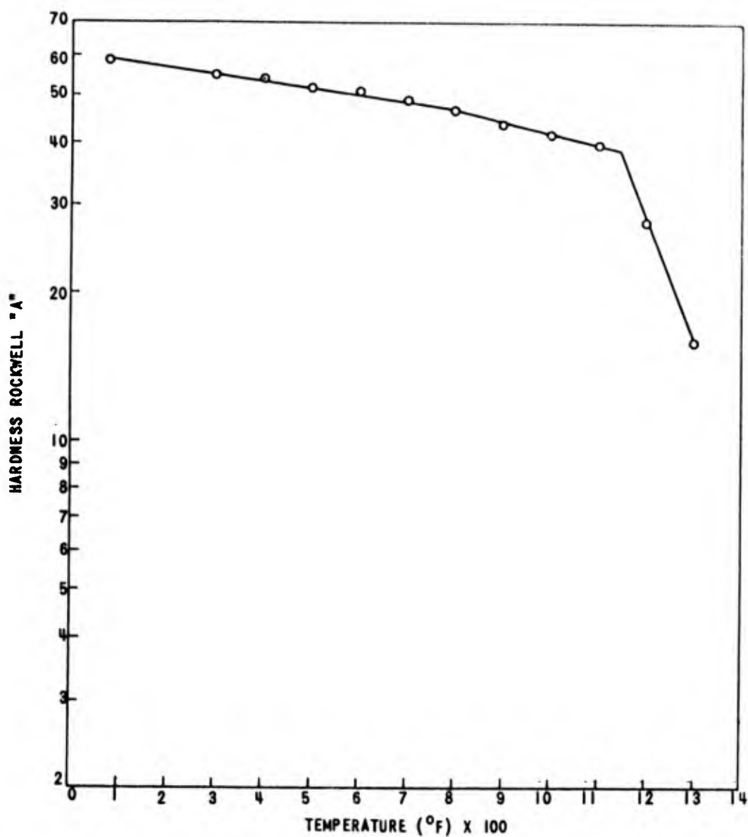
EFFECT OF TEMPERATURE ON THE HARDNESS OF Ti-13.8Zr (TZ4)
