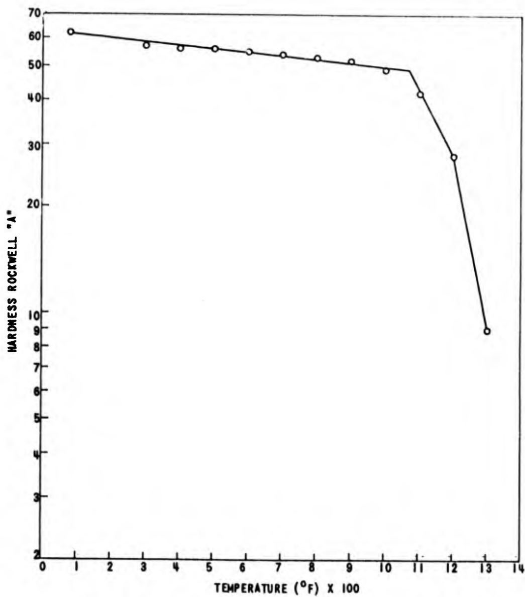
EFFECT OF TEMPERATURE ON THE HARDNESS OF Ti-31.5Zr (TZ7)
