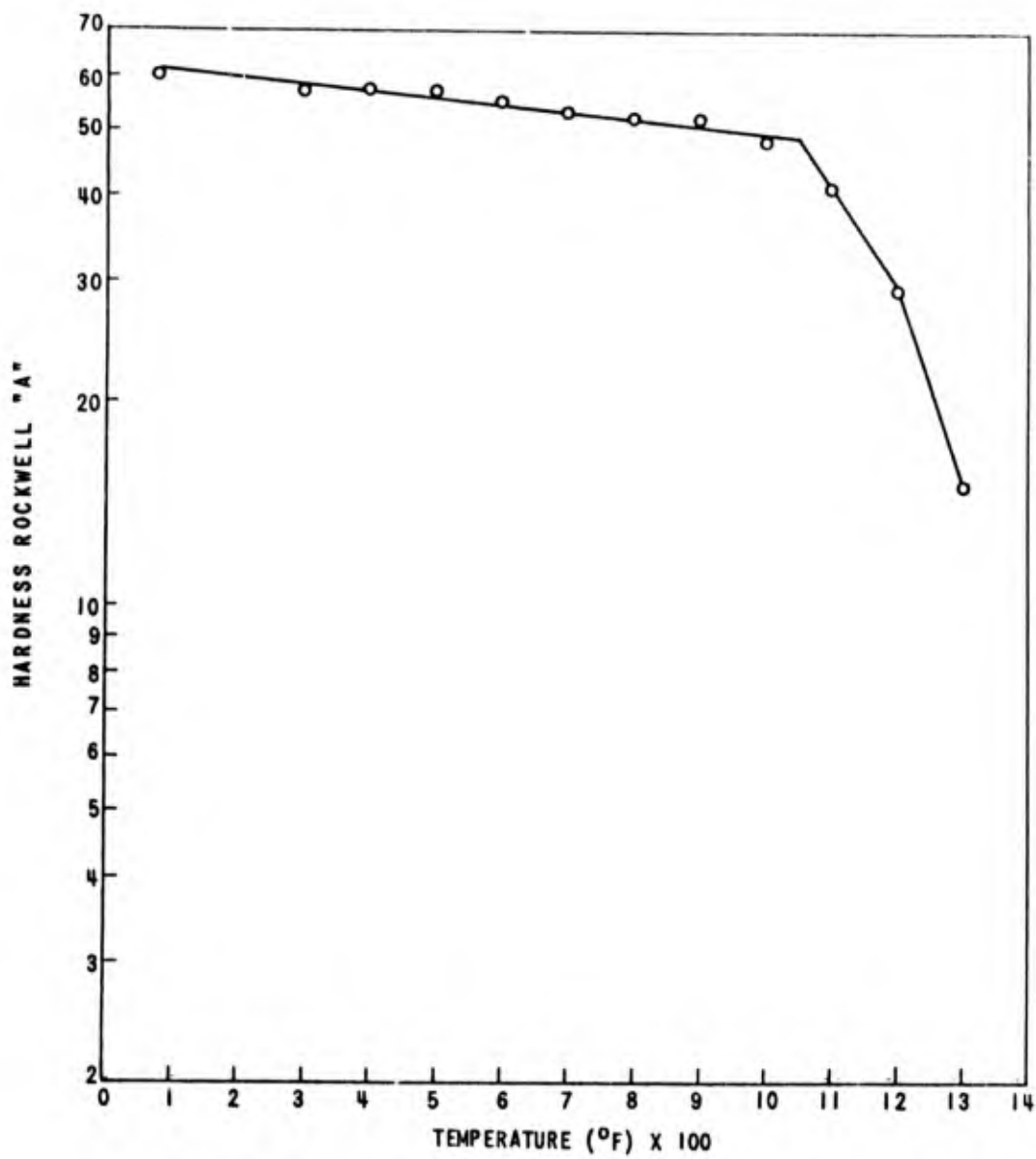
EFFECT OF TEMPERATURE ON THE HARDNESS OF Ti-26.3Zr (TZ6)
