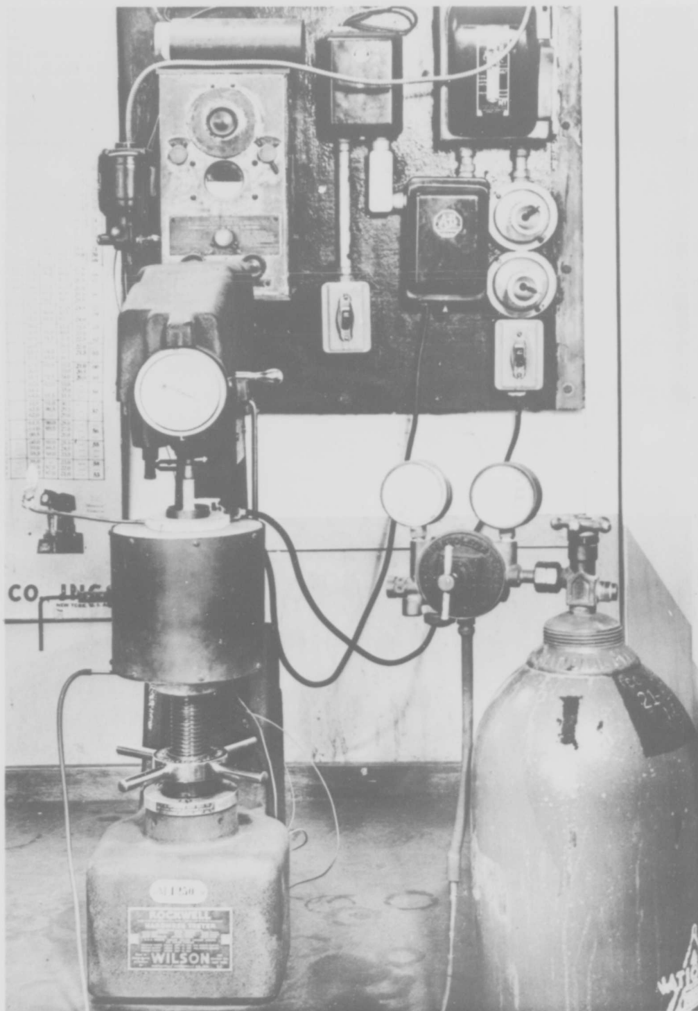
PHOTOGRAPH OF HOT HARDNESS SET-UP
