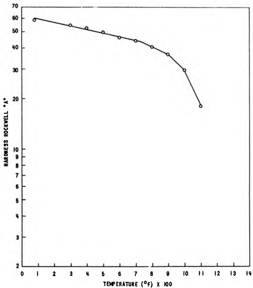
EFFECT OF TEMPERATURE ON THE HARDNESS OF Ti-3.8Cr-2.5Mo (AZ5)
