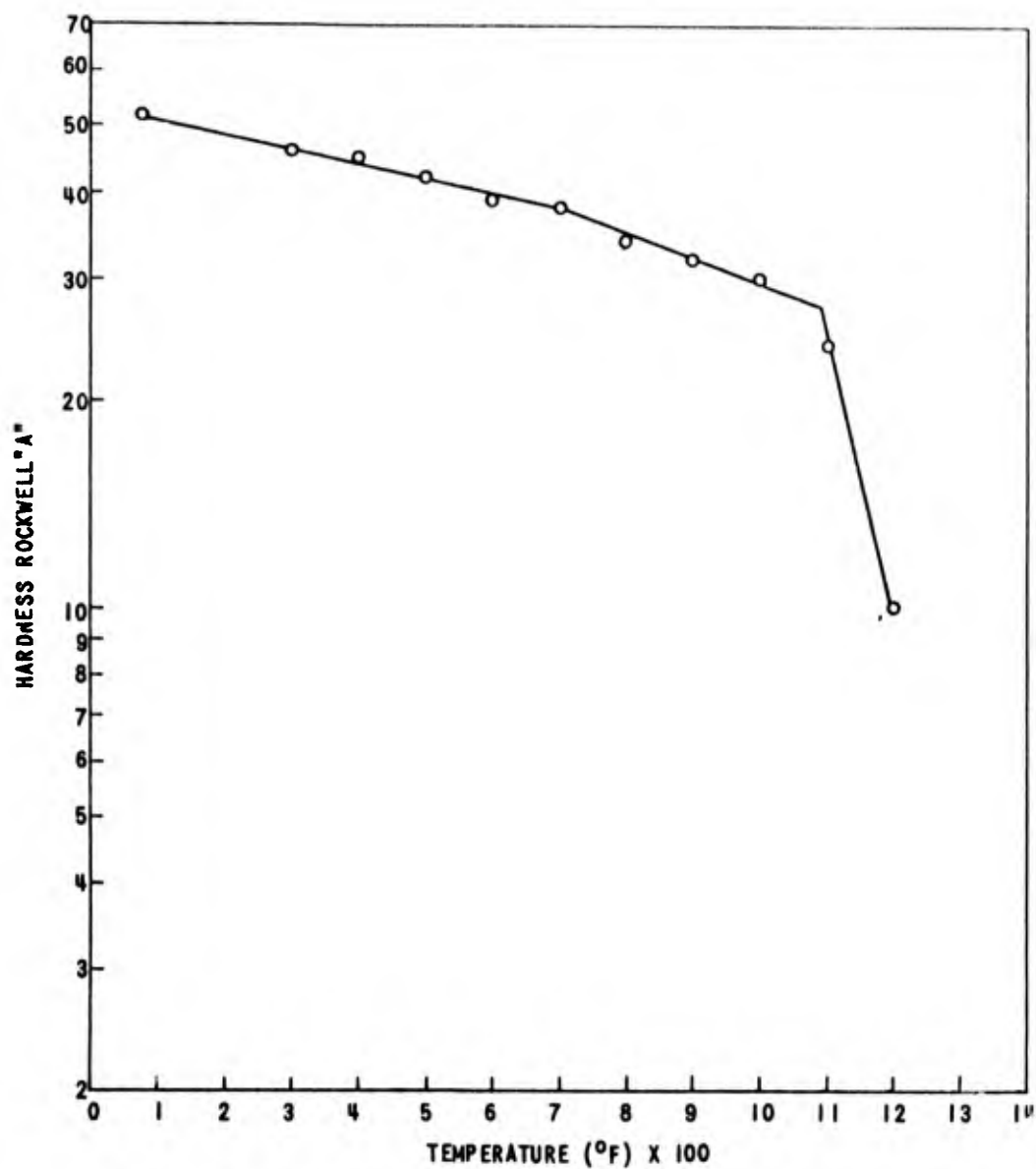
EFFECT OF TEMPERATURE ON THE HARDNESS OF Ti-9.4Zr (723)
