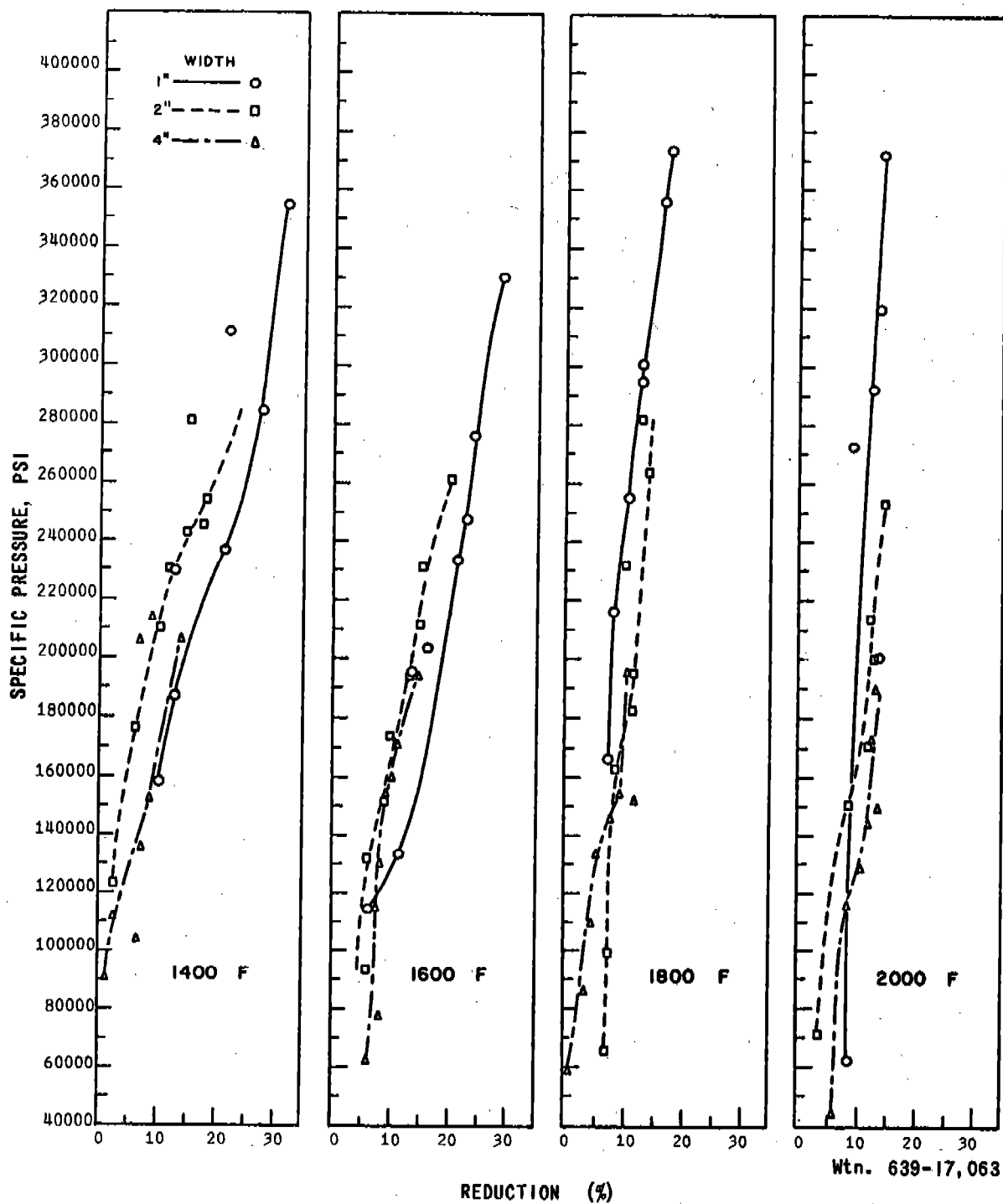
EFFECT OF ROLLING TEMPERATURE, REDUCTION, AND WIDTH ON SPECIFIC PRESSURE FOR Ti-6Al-4V ALLOY 1/32" THICK
