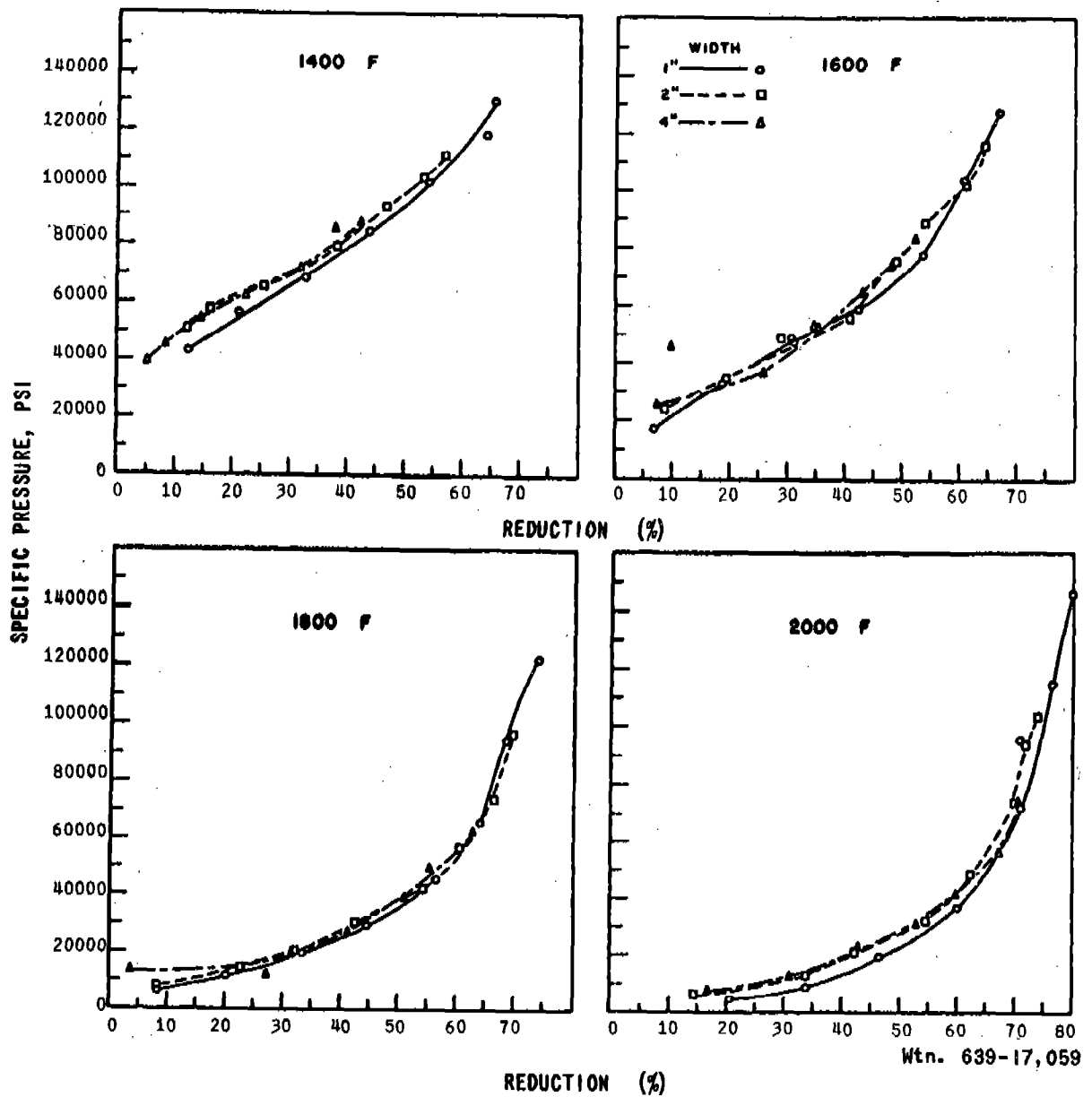
EFFECT OF ROLLING TEMPERATURE, REDUCTION AND WIDTH ON SPECIFIC PRESSURE FOR COMMERCIALLY PURE TITANIUM 1/8" THICK
