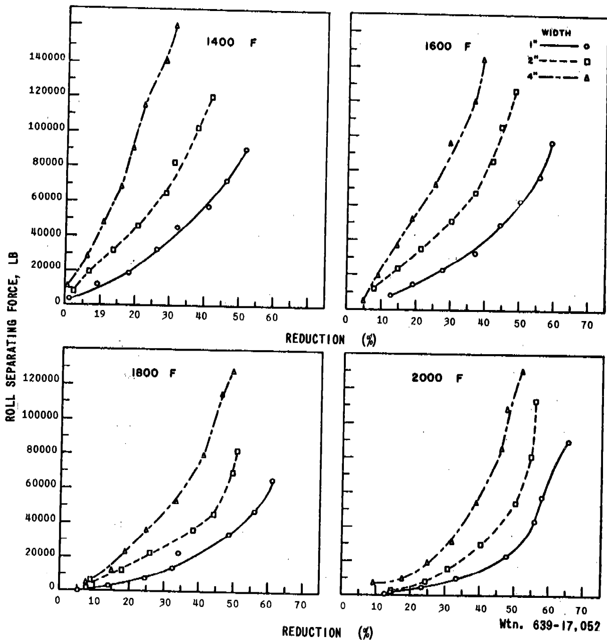
EFFECT OF ROLLING TEMPERATURE, REDUCTION, AND WIDTH ON ROLL SEPARATING FORCE FOR COMMERCIALLY PURE TITANIUM 1/16" THICK
