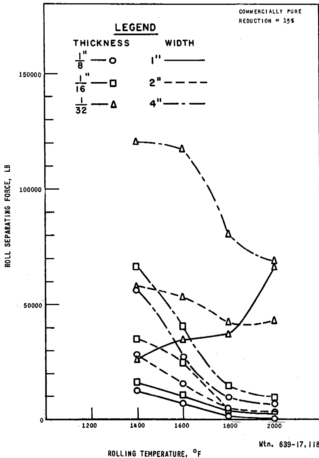
EFFECT OF ROLLING TEMPERATURE AND SPECIMEN SIZE ON ROLL SEPARATING FORCE
