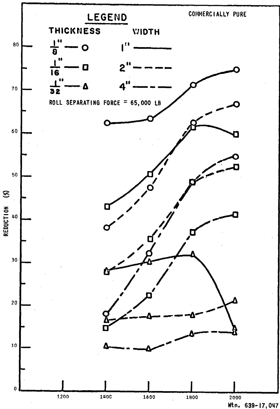
ROLLING TEMPERATURE °F EFFECT OF ROLLING TEMPERATURE AND SPECIMEN SIZE ON PERCENT REDUCTION
