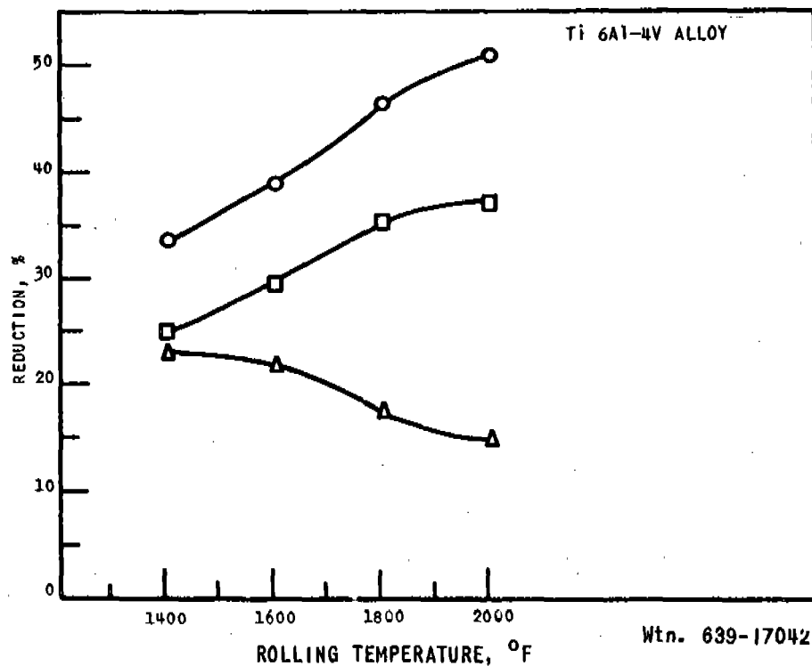
EFFECT OF ROLLING TEMPERATURE AND SPECIMEN THICKNESS ON REDUCTION
