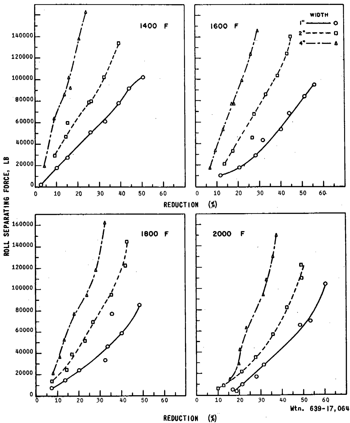
EFFECT OF ROLLING TEMPERATURE, REDUCTION, AND WIDTH ON ROLL SEPARATING FORCE FOR Ti-6Al-4V ALLOY 1/16" THICK
