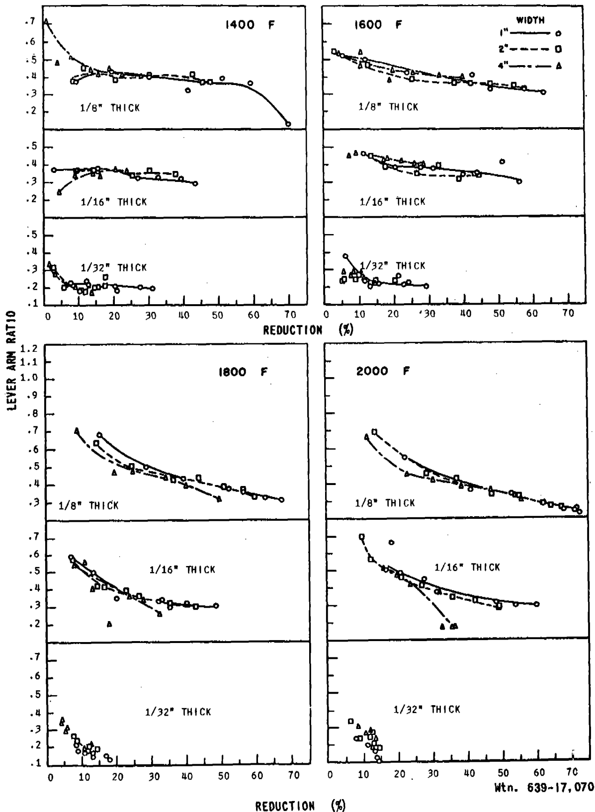
EFFECT OF ROLLING TEMPERATURE, REDUCTION, AND SPECIMEN SIZE ON LEVER ARM RATIO FOR Ti-6Al-4V TITANIUM
