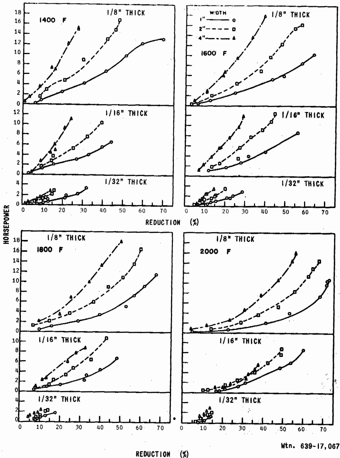
EFFECT OF ROLLING TEMPERATURE, REDUCTION, AND SPECIMEN SIZE ON HORSEPOWER CONSUMPTION FOR Ti-6Al-4V ALLOY
