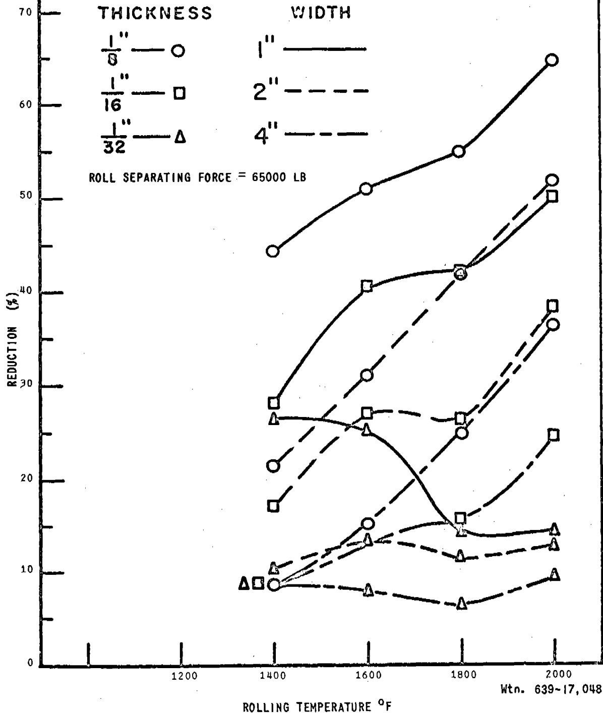
EFFECT OF ROLLING TEMPERATURE AND SPECIMEN SIZE ON PERCENT REDUCTION
