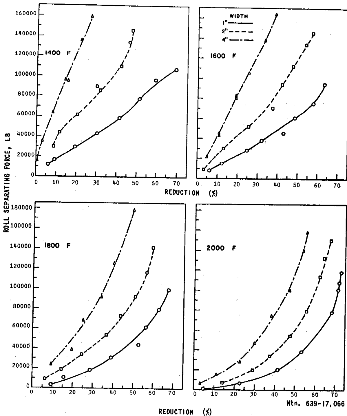
EFFECT OF ROLLING TEMPERATURE, REDUCTION, AND SPECIMEN WIDTH ON ROLL SEPARATING FORCE FOR Ti-6Al-4V ALLOY 1/8" THICK
