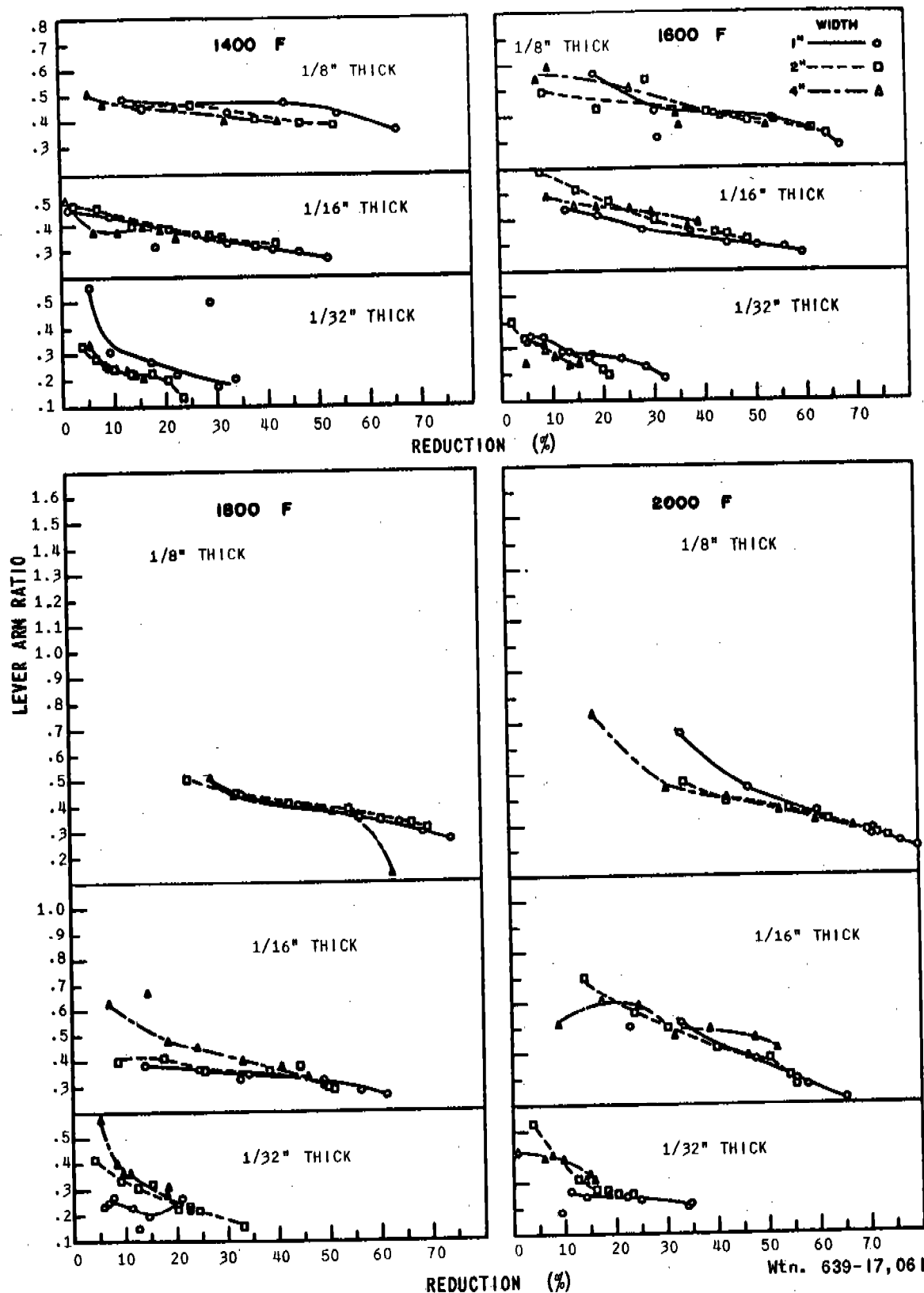
EFFECT OF ROLLING TEMPERATURE, REDUCTION, AND SPECIMEN SIZE ON LEVER ARM RATIO FOR COMMERCIAL PURE TITANIUM
