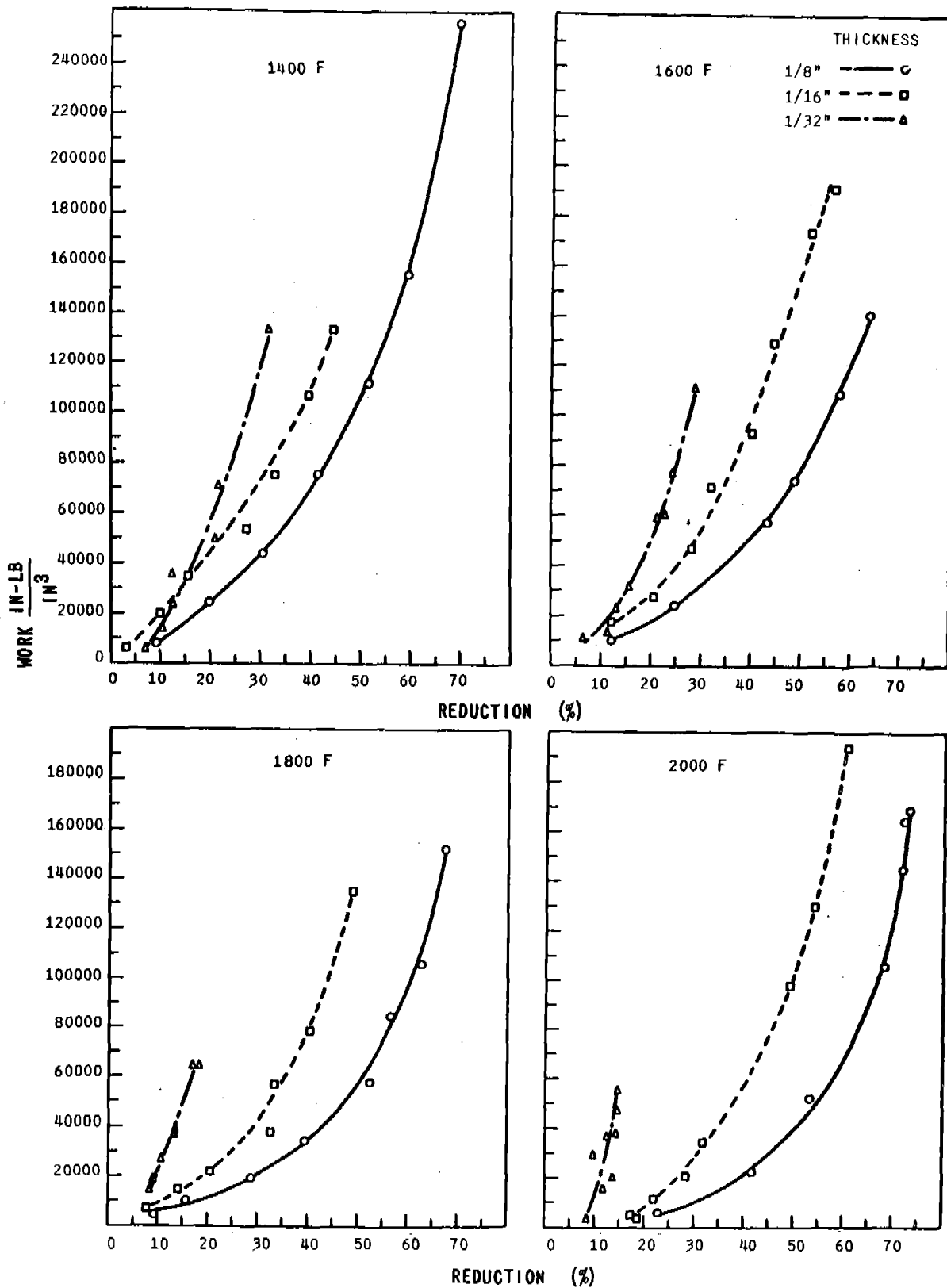
EFFECT OF ROLLING TEMPERATURE, REDUCTION, AND SPECIMEN THICKNESS ON WORK PER UNIT VOLUME FOR Ti-6Al-4V ALLOY 1" WIDE
