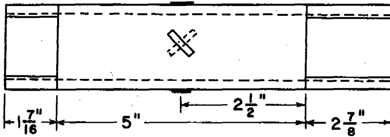
TORQUE ARM — SAE 1020 STEEL
