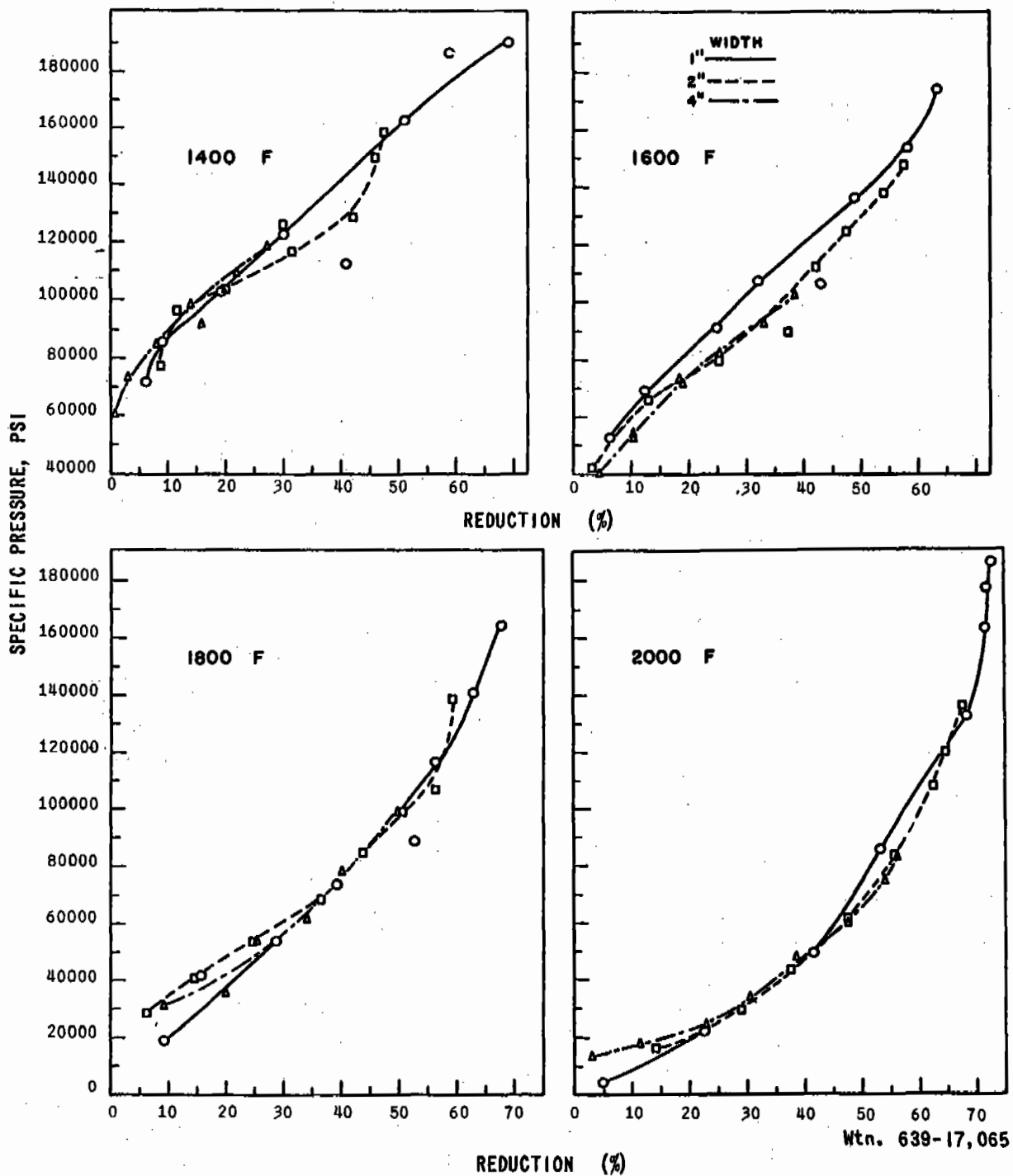
EFFECT OF ROLLING TEMPERATURE, REDUCTION, AND WIDTH ON SPECIFIC PRESSURE FOR Ti-6Al-4V ALLOY 1/8" THICK
