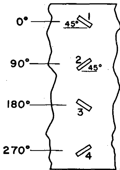
SR 4 STRAIN GAGE LOCATIONS
