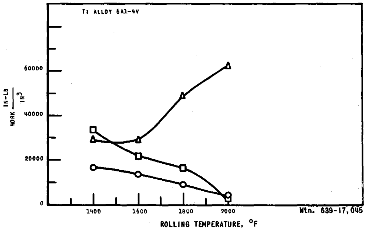
EFFECT OF ROLLING TEMPERATURE AND SIZE ON WORK PER UNIT VOLUME FOR A 15% REDUCTION
