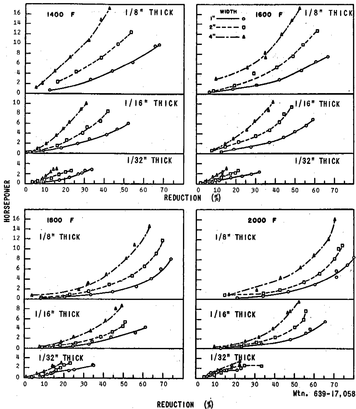
EFFECT OF ROLLING TEMPERATURE, REDUCTION, AND SPECIMEN SIZE ON HORSEPOWER CONSUMPTION FOR COMMERCIALY PURE TITANIUM
