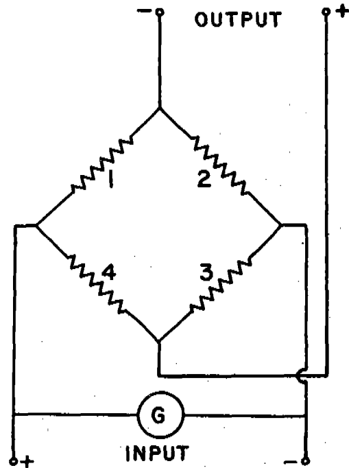
WIRING DIAGRAM
