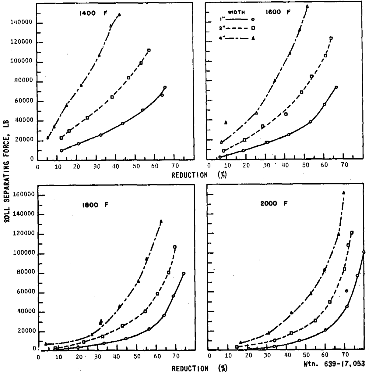
EFFECT OF ROLLING TEMPERATURE, REDUCTION AND WIDTH ON ROLL SEPARATING FORCE FOR COMMERCIALLY PURE TITANIUM 1/8" THICK
