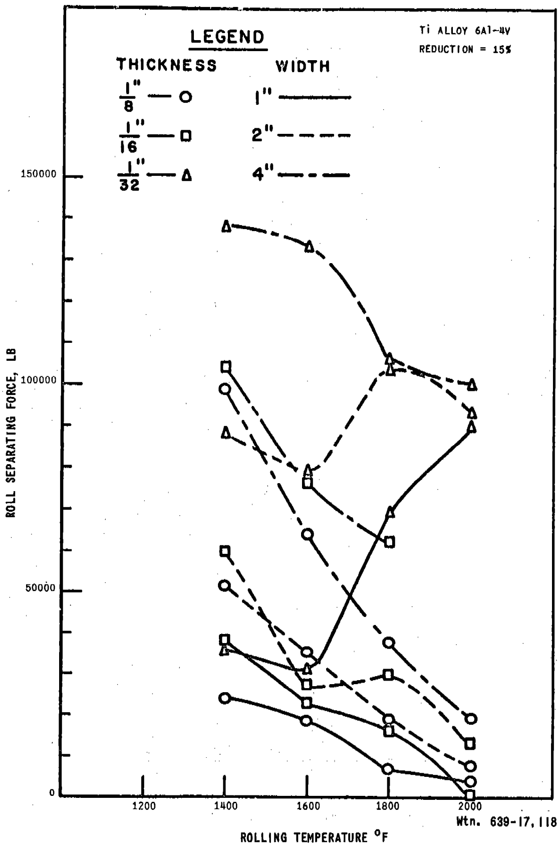
EFFECT OF ROLLING TEMPERATURE AND SPECIMEN SIZE ON ROLL SEPARATING FORCE
