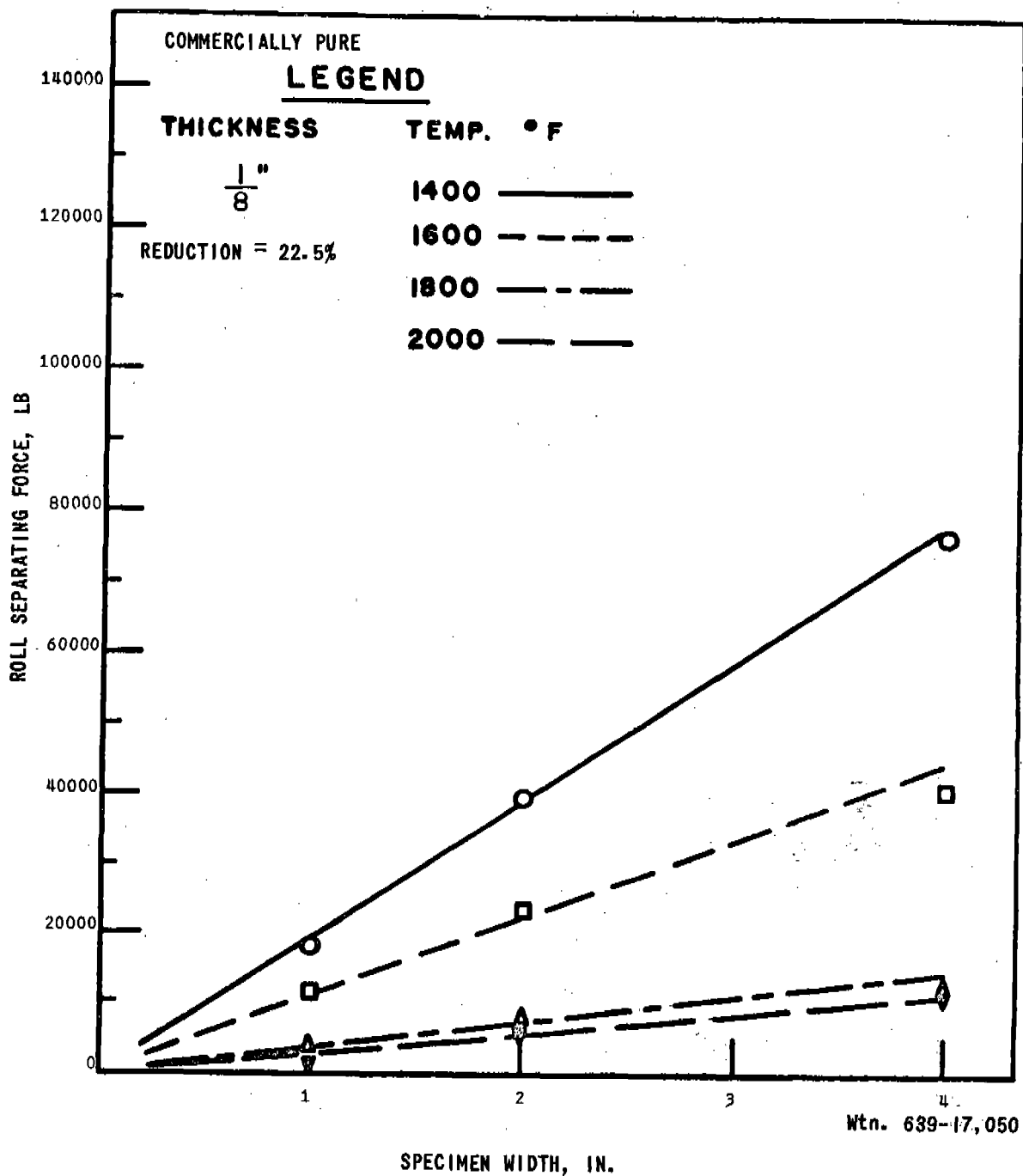
EFFECT OF ROLLING TEMPERATURE AND SPECIMEN WIDTH ON ROLL SEPARATING FORCE
