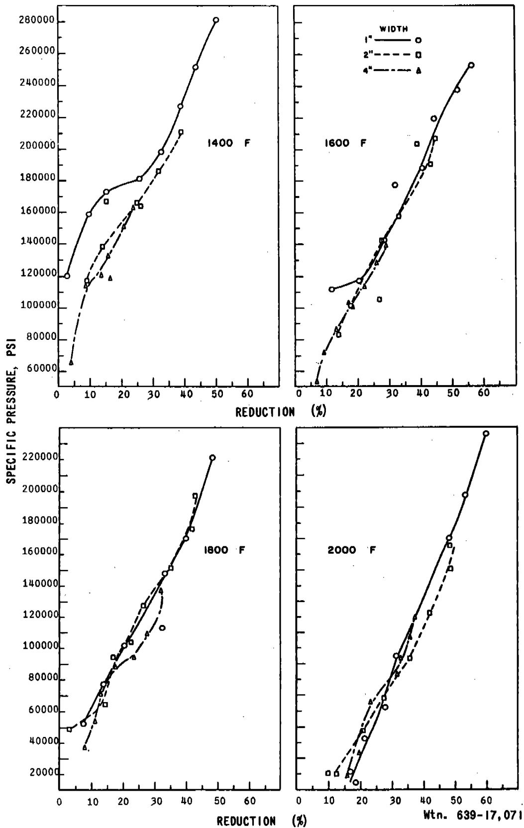
EFFECT OF ROLLING TEMPERATURE, REDUCTION, AND WIDTH ON SPECIFIC PRESSURE FOR Ti-6Al-4V ALLOY 1/16" THICK
