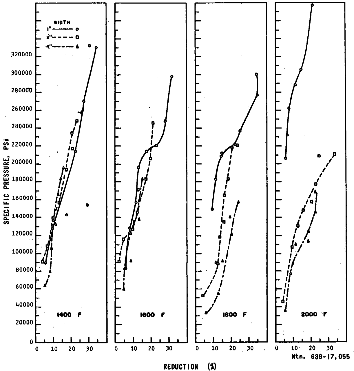
EFFECT OF ROLLING TEMPERATURE, REDUCTION, AND WIDTH ON SPECIFIC PRESSURE FOR COMMERCIALLY PURE TITANIUM 1/32" THICK
