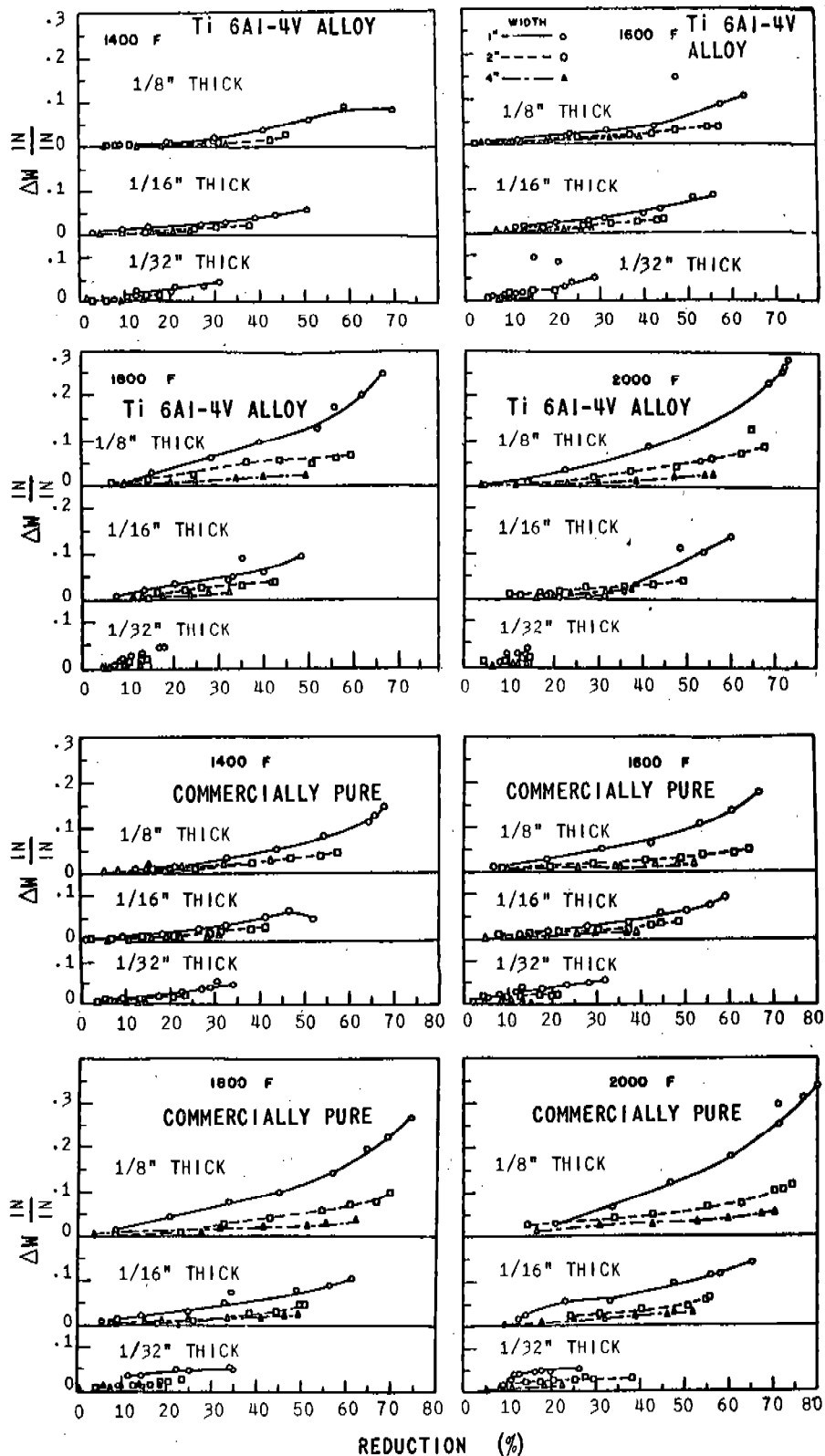
EFFECT OF ROLLING TEMPERATURE, REDUCTION, AND SPECIMEN SIZE ON SPREAD
