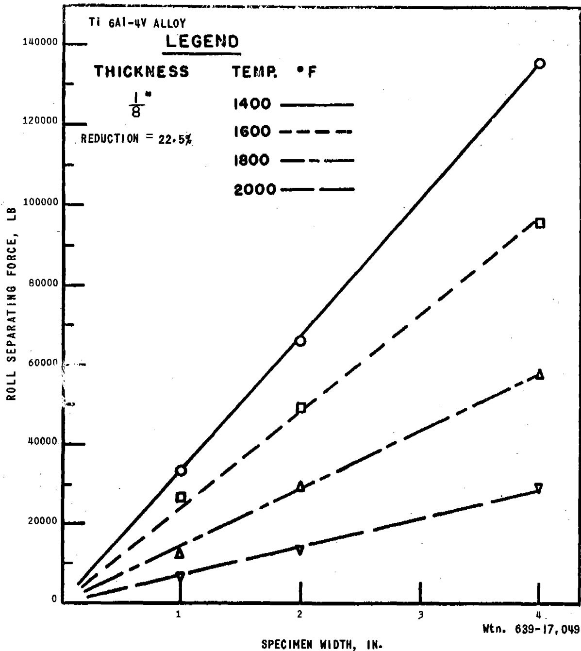
EFFECT OF ROLLING TEMPERATURE AND SPECIMEN WIDTH ON ROLL SEPARATING FORCE
