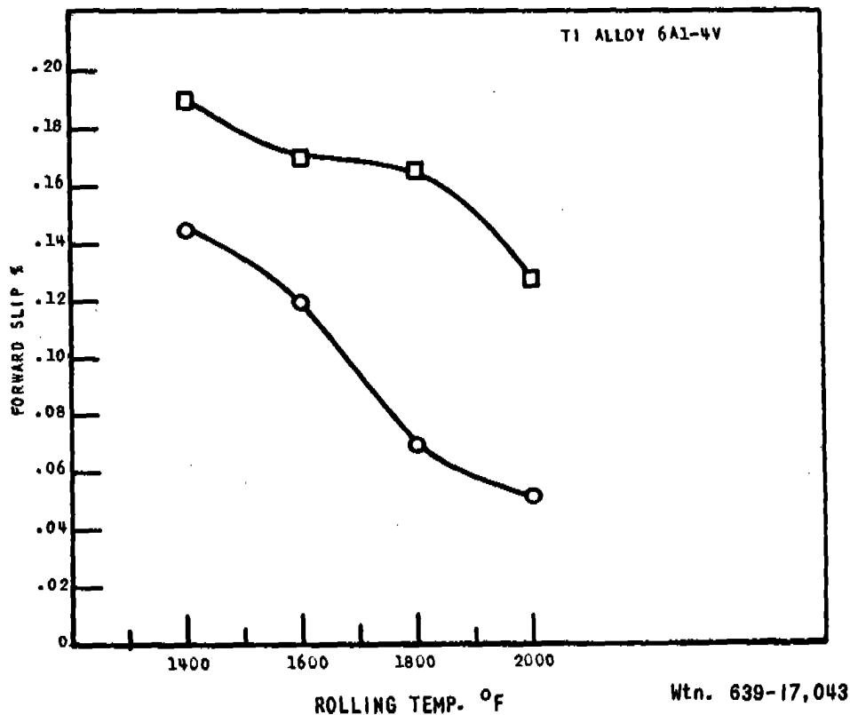
EFFECT OF ROLLING TEMPERATURE AND SPECIMEN THICKNESS ON FORWARD SLIP
