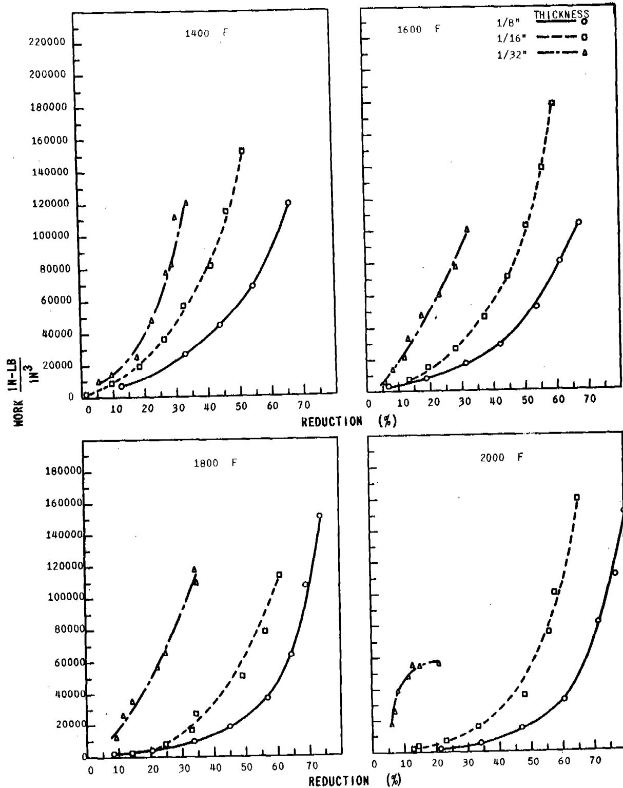
EFFECT OF ROLLING TEMPERATURE, REDUCTION, AND INITIAL THICKNESS ON WORK PER UNIT VOLUME FOR COMMERCIALLY PURE TITANIUM 1" WIDE
