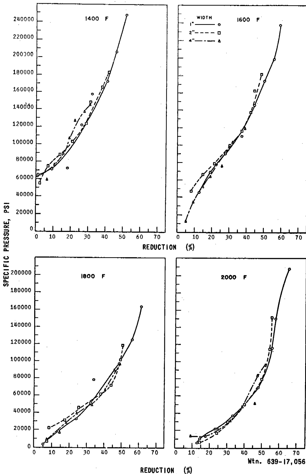
EFFECT OF ROLLING TEMPERATURE, REDUCTION, AND WIDTH ON SPECIFIC PRESSURE FOR COMMERCIALLY PURE TITANIUM 1/16" THICK
