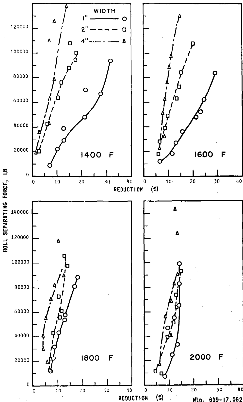
EFFECT OF ROLLING TEMPERATURE, REDUCTION AND WIDTH ON ROLL SEPARATING FORCE FOR Ti-6Al-4V ALLOY 1/32" THICK
