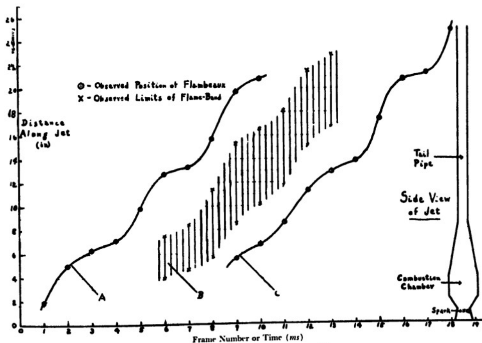
Figure 18. Motion of flame in a jet "cycle."
