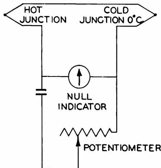
Figure 18. Thermocouple circuit.
