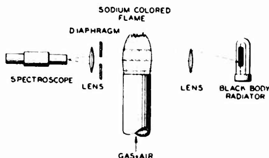
Figure 19. Sodium D-line reversal apparatus.
