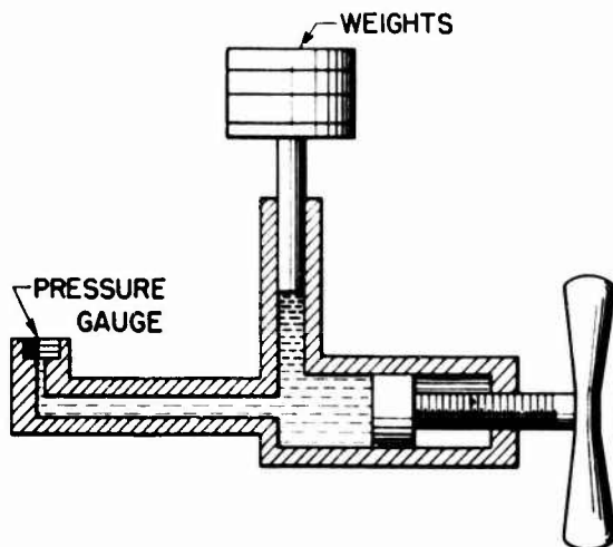
Figure 8. Dead weight gauge.
