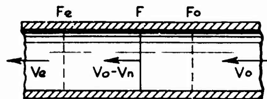
Figure 5. Idealized ramjet combustion.
