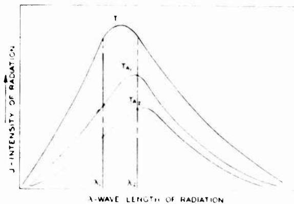
Figure 20. Two-color method.
