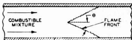
Figure 30. Flow-angle method.
