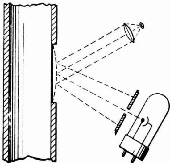
Figure 13. Optical gauge.
