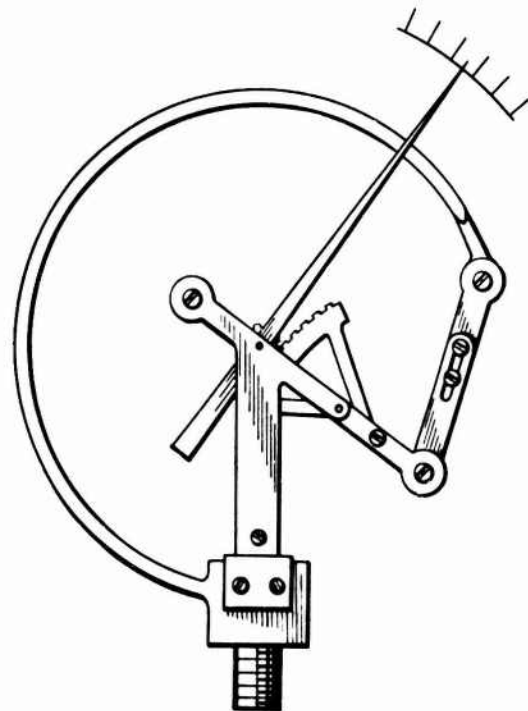
Figure 9. Bourdon gauge.
