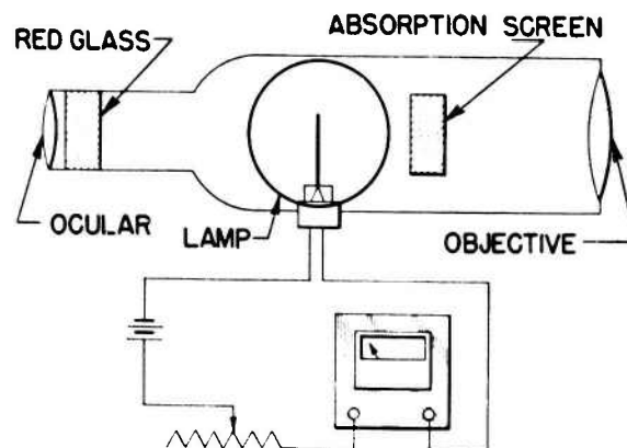
Figure 21. Optical pyrometer.
