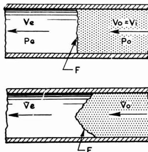
Figure 4. Stationary flame in tube.
