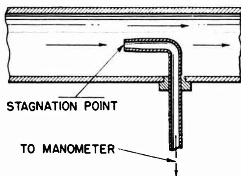
Figure 23. Pitot tube.
