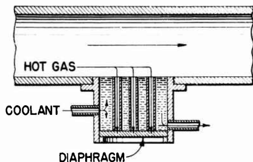
Figure 10. Cooling cell.
