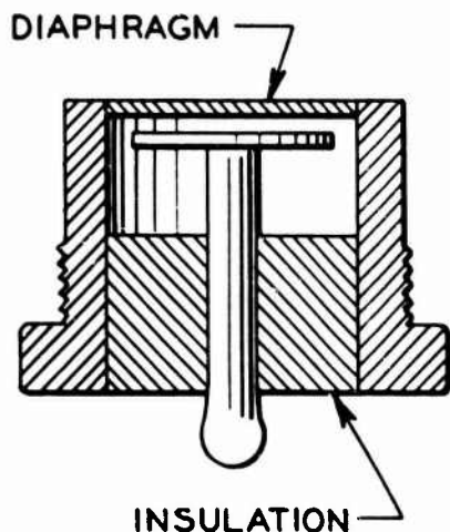
Figure 11. Capacitance gauge.
