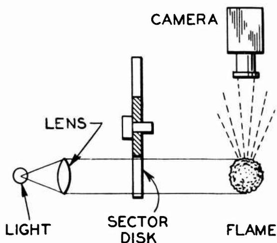
Figure 25. Apparatus for tracer photography.
