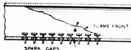
Figure 29. Ignition-angle method.
