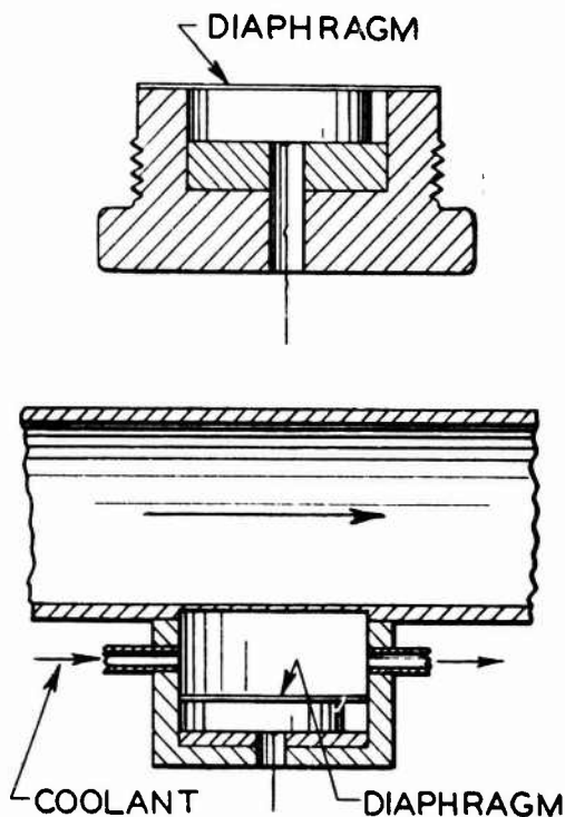
Figure 14. Piezoelectric gauge.
