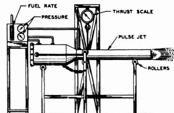
Figure 1. Pulse jet test stand.
