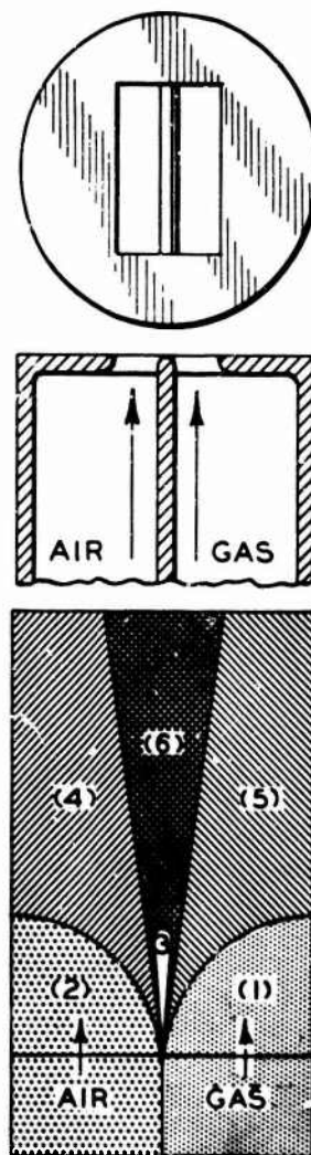
Figure 2. Unmixed combustion.
