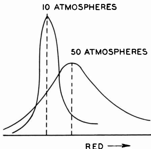
Figure 17. Spectral line pressure shift.
