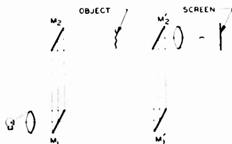
Figure 28. Optical interferometer.
