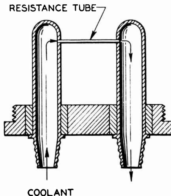
Figure 24. Cold-wire anemometer.
