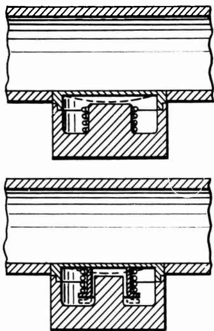
Figure 12. Electromagnetic gauge.
