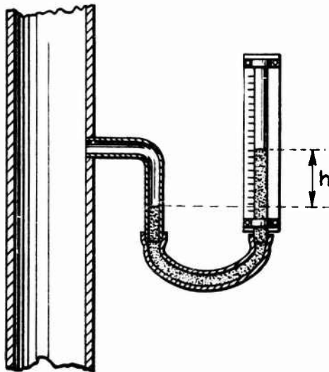
Figure 7. Mercury manometer.
