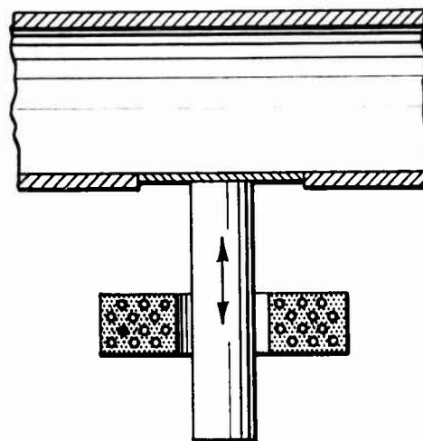
Figure 15. Magnetostriction gauge.
