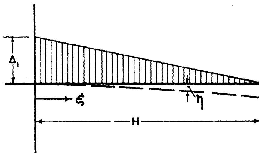
FIGURE 1b Reed loading.
