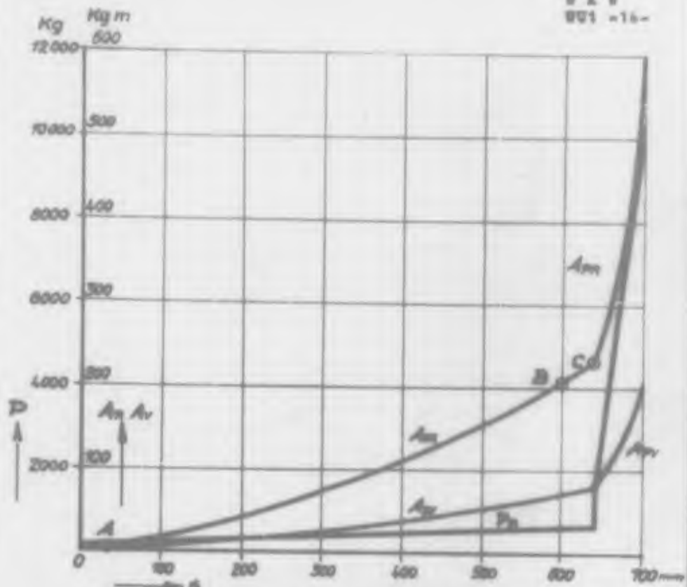
Figure 3 Spring Strength and Max Potential of the Closing Spring and Bottom Surface Springs
