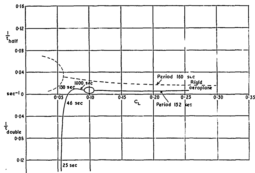
FIG. 9b. 'Phugoid' mass distribution B.
