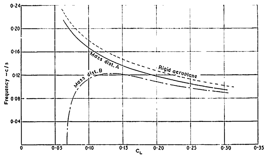
FIG. 10a. 'Short period' frequency.
