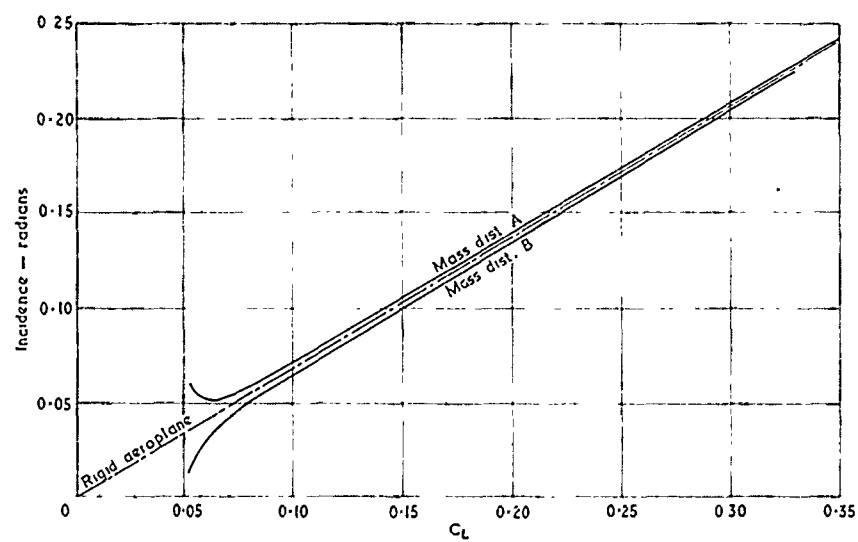
FIG. 7. Incidence in level flight.
