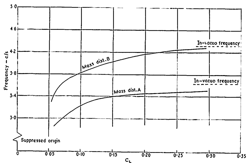
FIG. 12a. 'Second normal mode' frequency.
