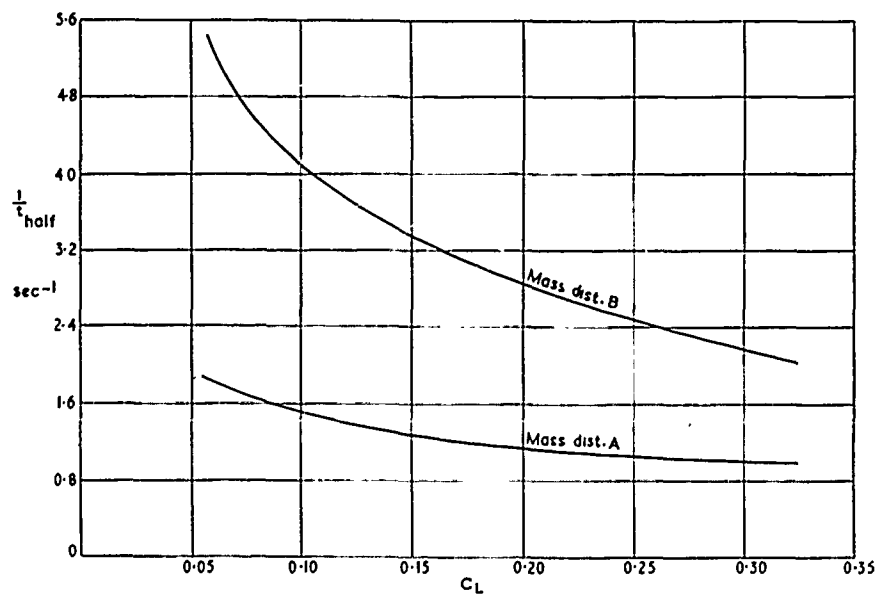
FIG. 12b. 'Second normal mode' damping.
