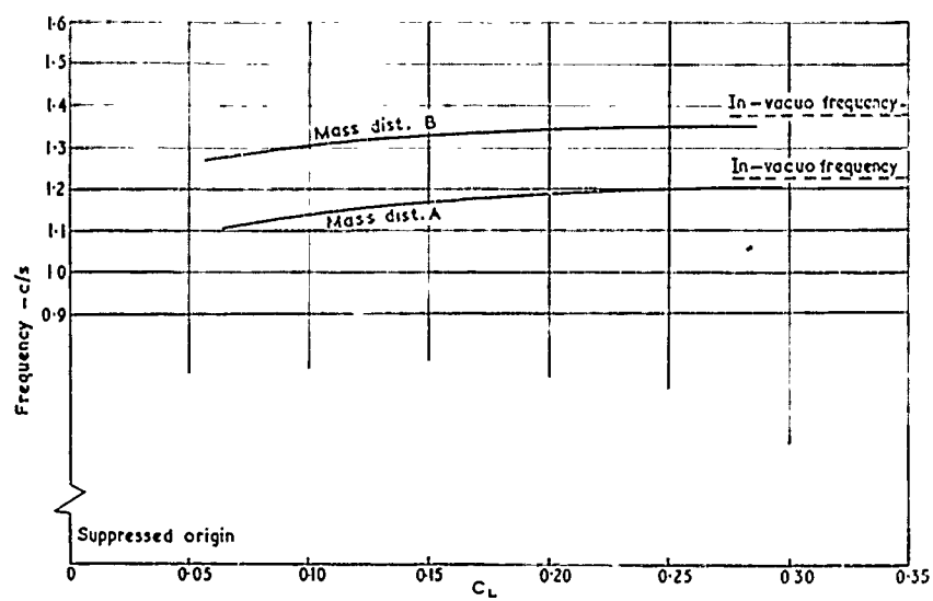
FIG. 11a. 'First normal mode' frequency.
