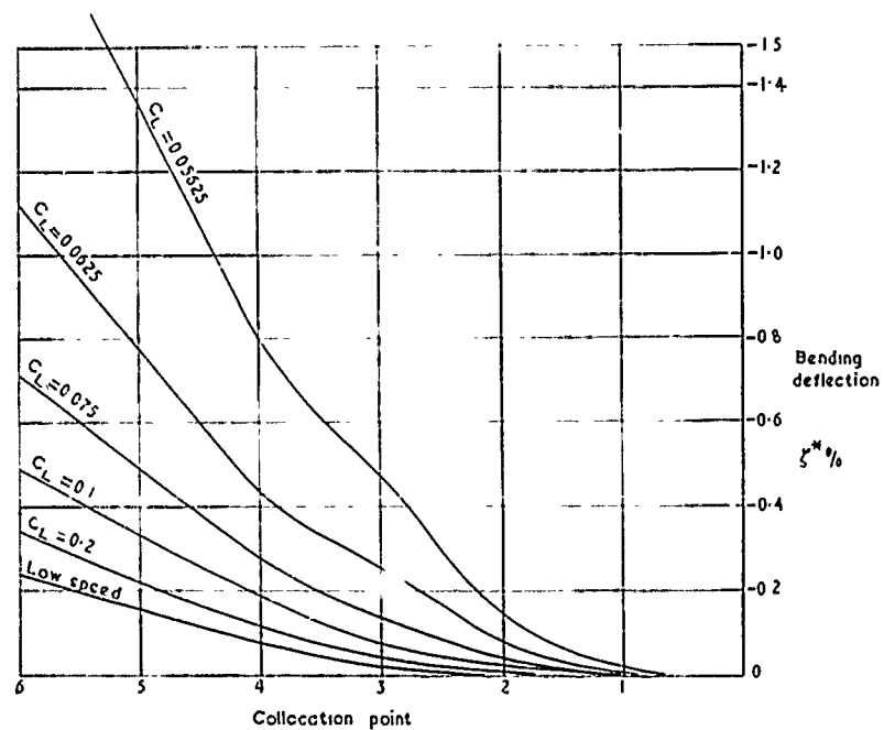
FIG. 6b. Configuration in level flight—mass distribution B.
