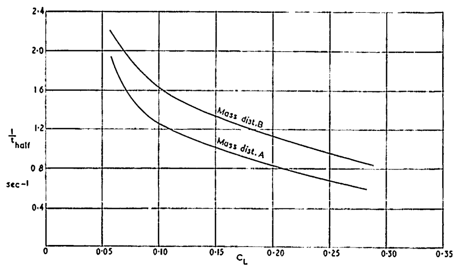
FIG. 11b. 'First normal mode' damping.
