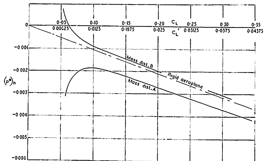
FIG. 13. Control coefficient per g .
