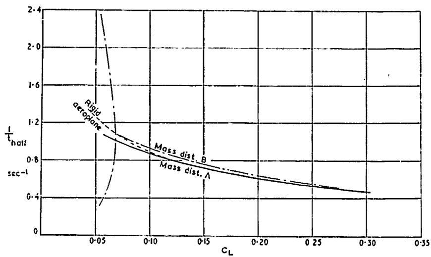
FIG. 10b. 'Short period' damping.
