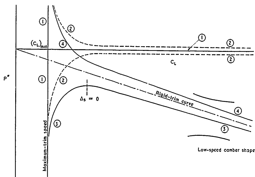
FIG. 3. Trim curves for uncambered aeroplane.
