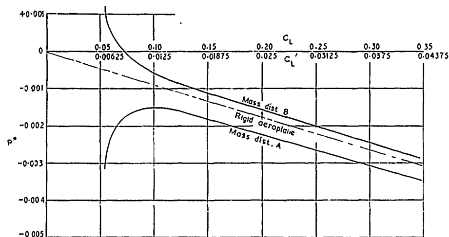
FIG. 5. Level-flight-trim curve.
