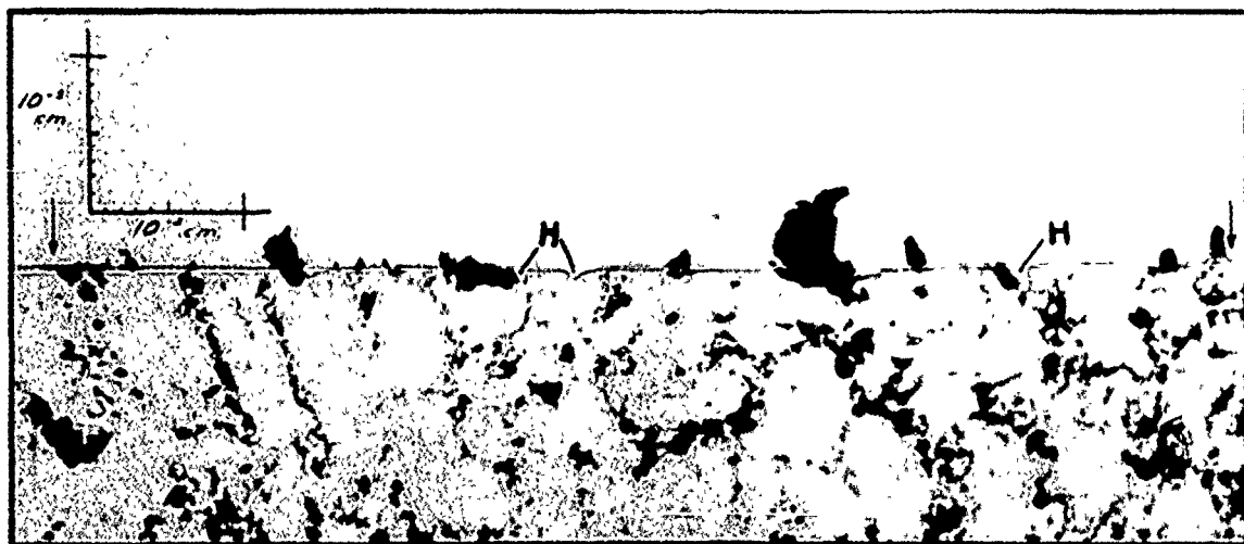
FIG. 2. Taper-section of track formed by sliding a hemispherical copper rider on an unlubricated steel surface. Horizontal magnification 200. Vertical magnification 2000. The width of the track is indicated by arrows. Note the adhering fragments of copper, and the pits marked H where the steel has been plucked out of the surface.
