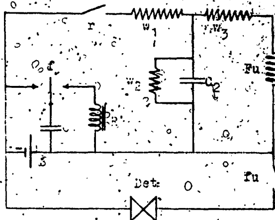
Microphonic Transformer
