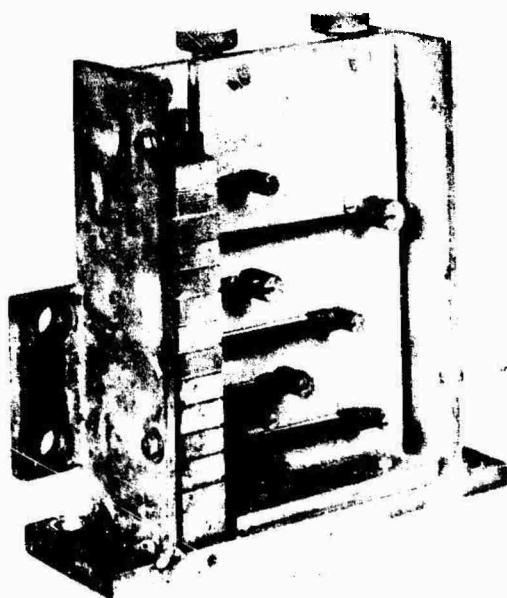
Fig. 3 - Reed gage, (cover removed), showing reeds and records scribed on wax paper
