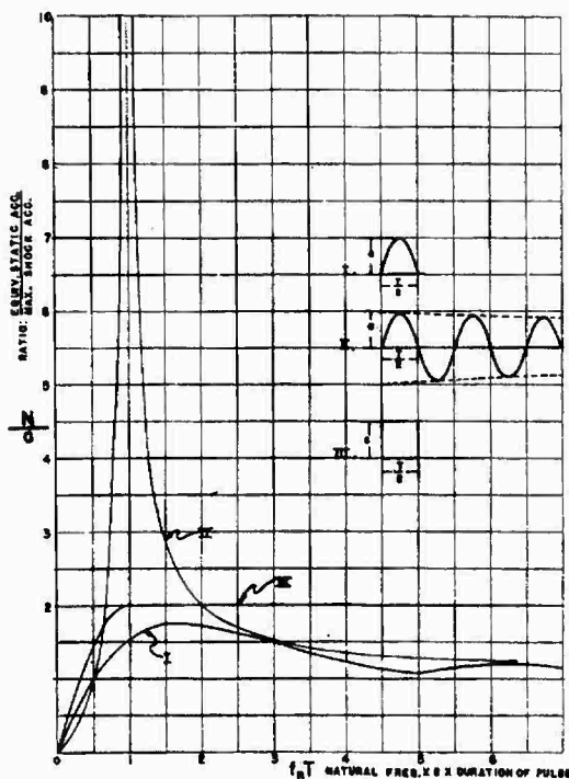
Fig. 4 - Shock spectra for three simple shocks
