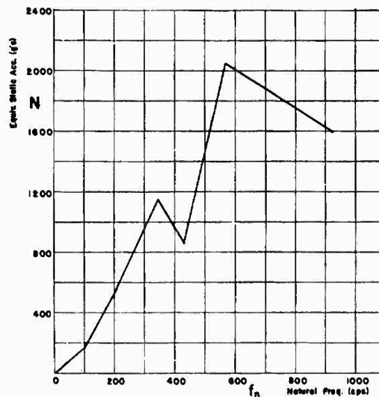
Fig. 14 - Shock spectra of the motion of the Medium-Weight Shock Machine, 3-inch table travel, 2-foot hammer drop, 500-pound load on table
