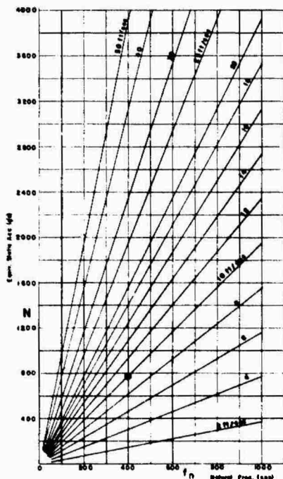
Fig. 5 - Shock spectra for velocity change
