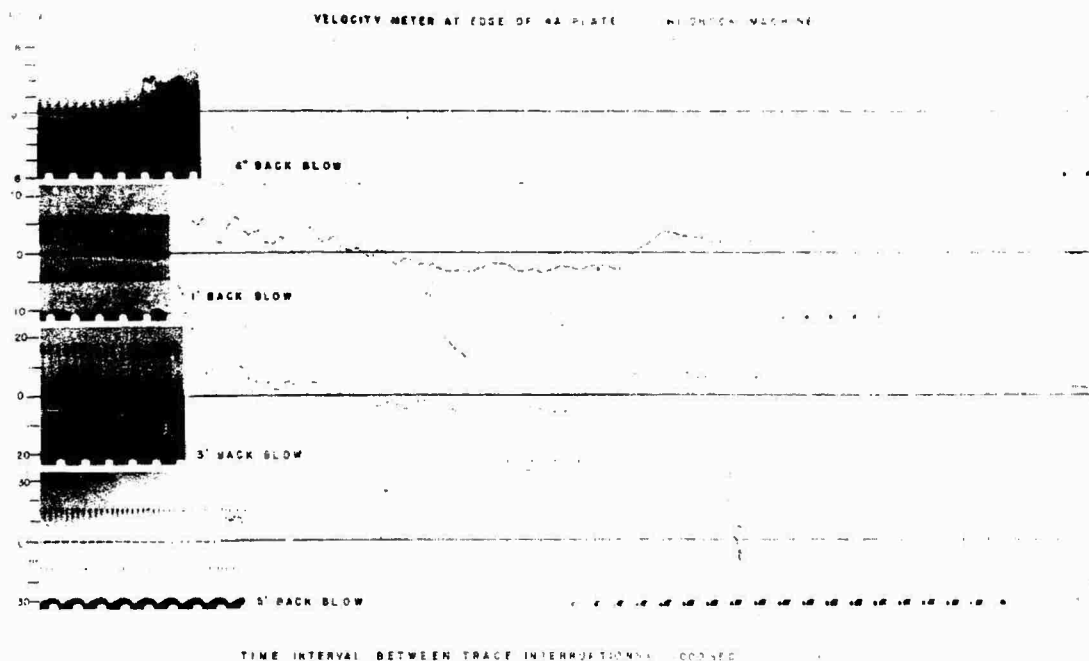
Fig. 12 - Velocity - time record of motion of 4A plate over supporting channel Navy Light-Weight Shock Machine
