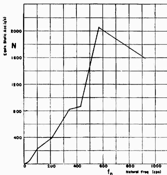
Fig. 13 - Shock spectra of the motion of the Medium-Weight Shock Machine, 3-inch table travel, 1-foot hammer drop, 500-pound load on table
