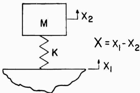
Fig. 1 - A single-degree-of-freedom system
