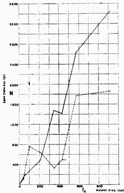
Fig. 10 - 5-foot back blow
