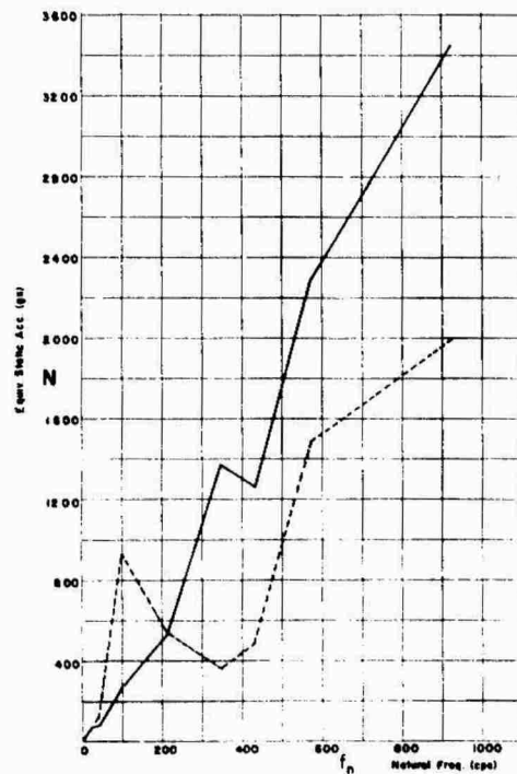
Fig. 9 - 4-foot back blow
