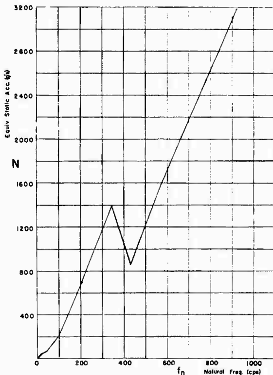
Fig. 15 - Shock spectra of the motion of the Medium-Weight Shock Machine, 1.5-inch table travel, 1-foot hammer drop, 500-pound load on table
