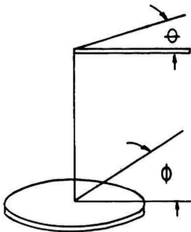
Fig. 2 - Diagram of torsion pendulum
