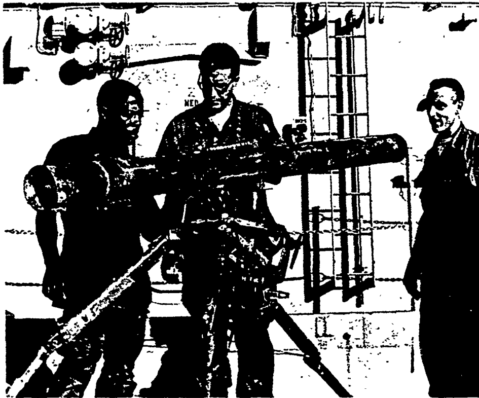
A communist-made 122-mm rocket launcher gets a going over by its captors. The launcher was seized off a sampan on the Dong Nai River, 12 miles east of Saigon, shortly after midnight on 9 July 1968.
