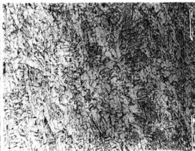
Fig. 10 10% Nital x100 Weld structure - position #5
