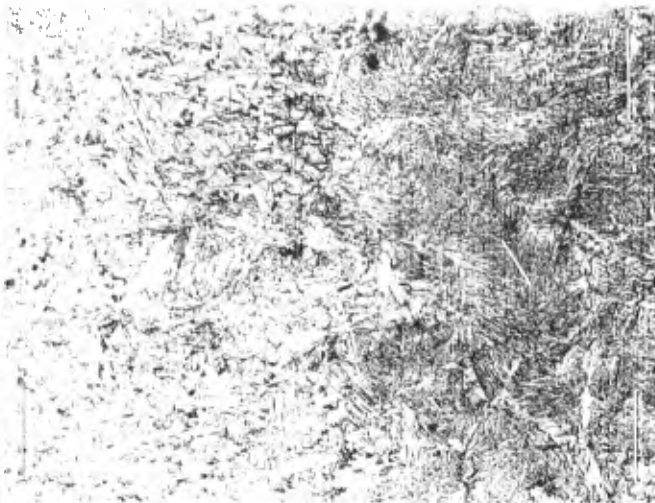
Fig. 7 10% Nital x100 Fusion zone of weld and plate. Position #6
