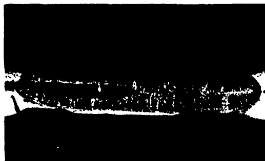
PLATE 4481-M.—Magnified 59× diameter. Etch, chrome regia. Photomicrograph of similar spot weld after 100 hours' Strauss test.
