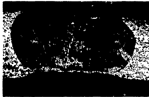
PLATE 4440-M.—Magnified 37× diameter. Etch, glycerol. Photomicrograph of a similar spot weld after 100 hours' Strauss test.
