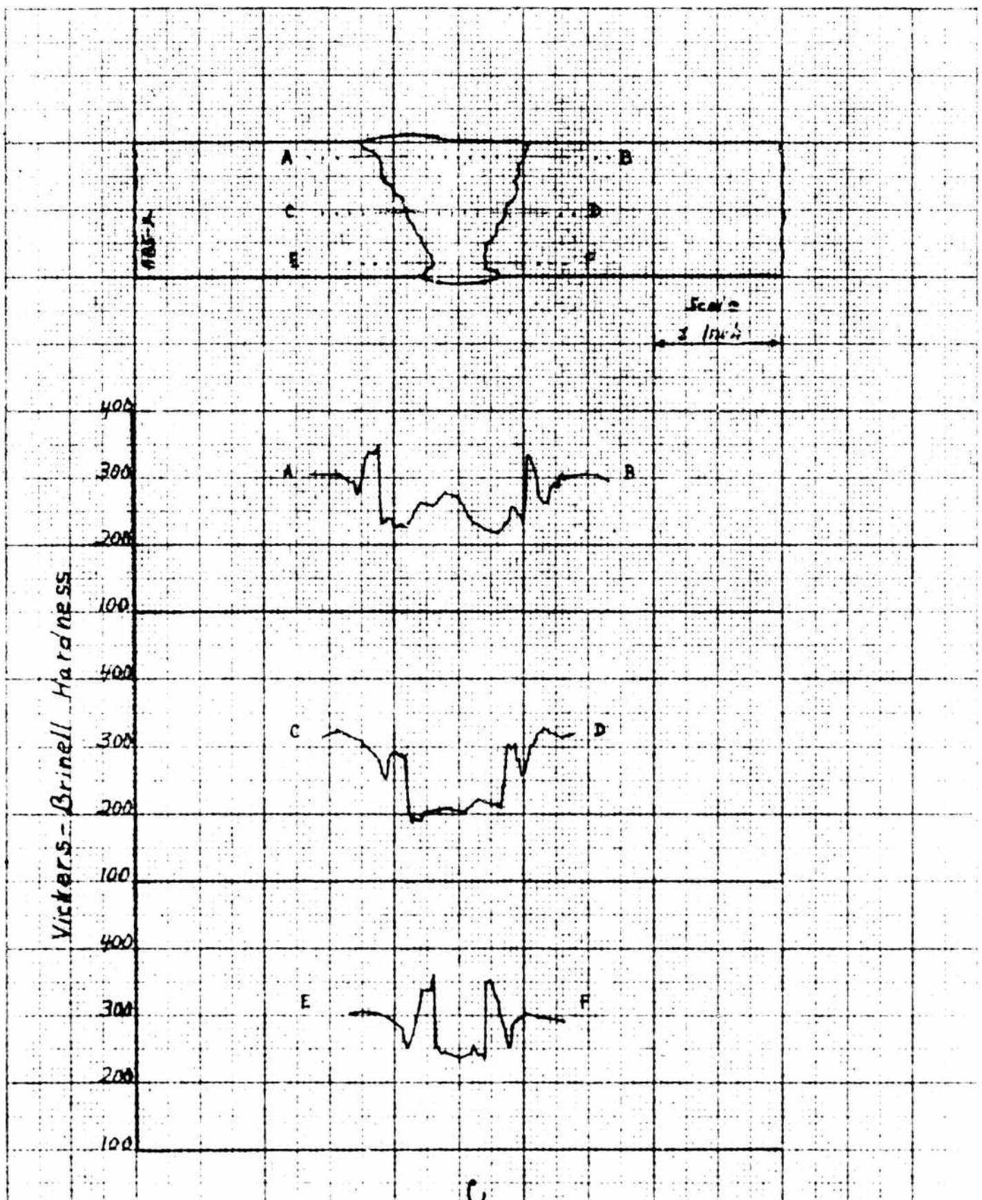
FIGURE 15. SINGLE V JOINT WELDED WITH LOW ALLOY LINCOLN SHIELD METAL ARC ELECT. GDE. STRESS RELIEVED AT 1000°F FOR 3 HRS. AND AIR COOLED.
