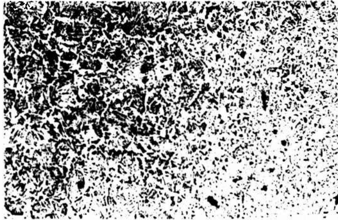
X100 1% NITAL MICROSTRUCTURE OF WELD METAL NEAR ROOT (LOCATION 3)
