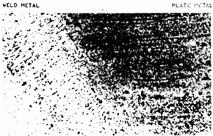
X100 1% NITAL MICROSTRUCTURE AT BOUNDARY BETWEEN PLATE AND WELD METAL (LOCATION 4)
