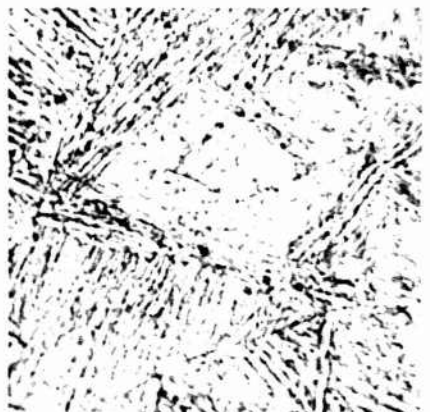
MICROSTRUCTURE OF HEAT AFFECTED PLATE IMMEDIATELY ADJACENT TO WELD NEAR EDGE (LOCATION 13)
