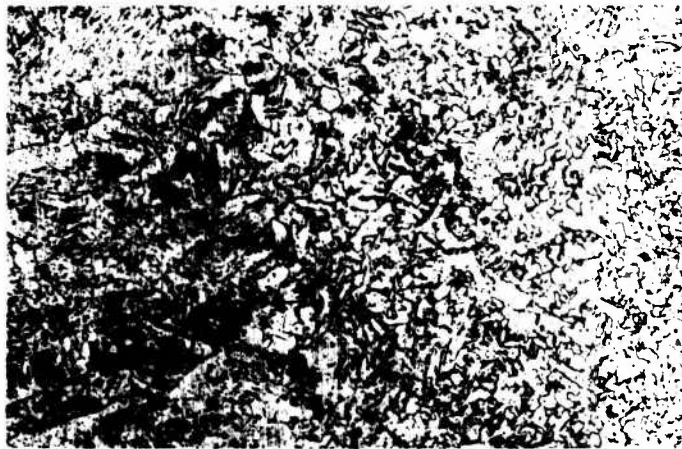
X100 1% NITAL MICROSTRUCTURE OF WELD METAL NEAR CROWN (LOCATION 6)
