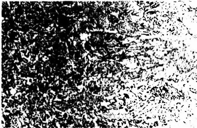
X100 1% NITAL MICROSTRUCTURE OF WELD METAL NEAR ROOT. (LOCATION 7)
