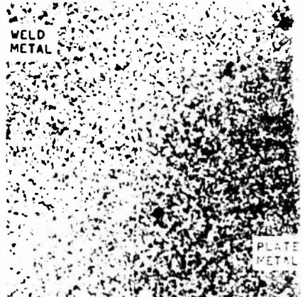
MICROSTRUCTURE AT BOUNDARY BETWEEN PLATE AND WELD METAL (LOCATION 12)
