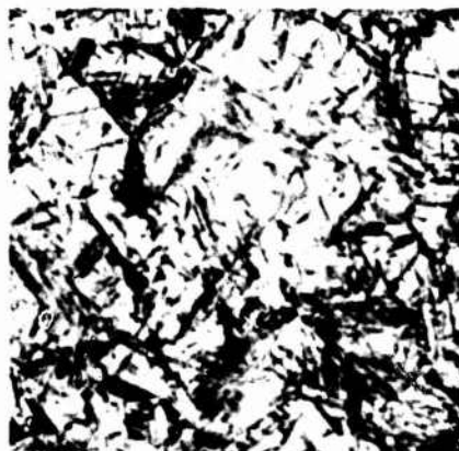
MICROSTRUCTURE OF HEAT AFFECTED PLATE IMMEDIATELY ADJACENT TO WELD NEAR EDGE (LOCATION 13)
