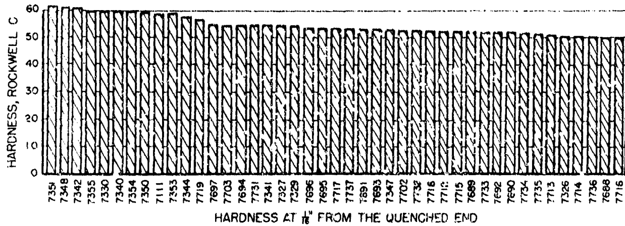
A COMPARISON OF THE HARDENABILITY OF 43 HEATS FIG. 146
