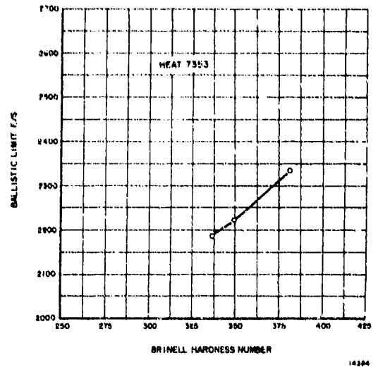
Figure 97. Heat No. 7353. Relationship of ballistic limit to Brinell hardness.
