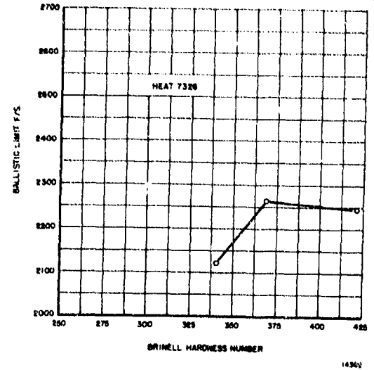
Figure 85. Heat No. 7326. Relationship of ballistic limit to Brinell hardness.
