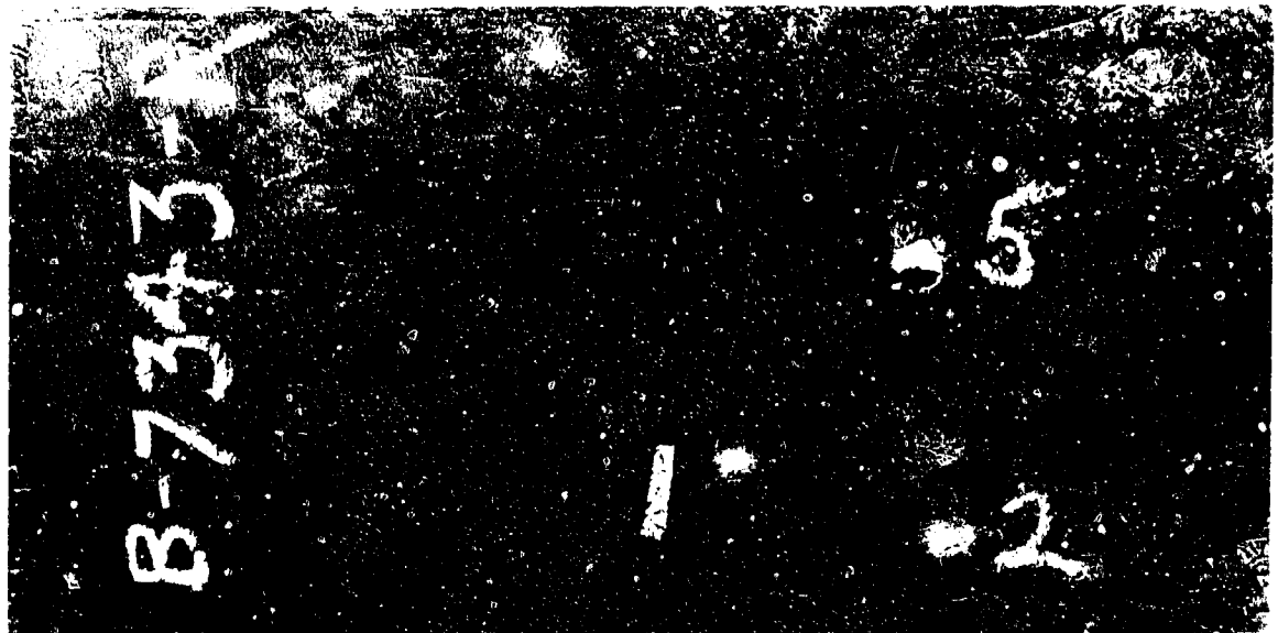
Figure 65. Heat No. 7343. Back of as rolled plate after ballistic tests. Ballistic limit 2312 feet per second, .30 cal. A. P. bullet. Rockwell "C" cross-section hardness survey: 39, 39, 39, 39, 38, 39, 38. Average equivalent Brinell-362. Photograph 1/2 Actual Size.
