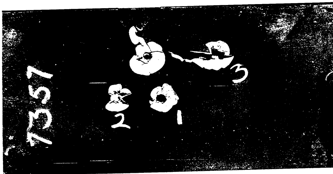
Figure 60. Heat No. 7357. Back of plate after ballistic tests. Ballistic limit not determined, .30 cal. A. P. bullet. Average Brinell- 363. Photograph 1/2 Actual Size.
