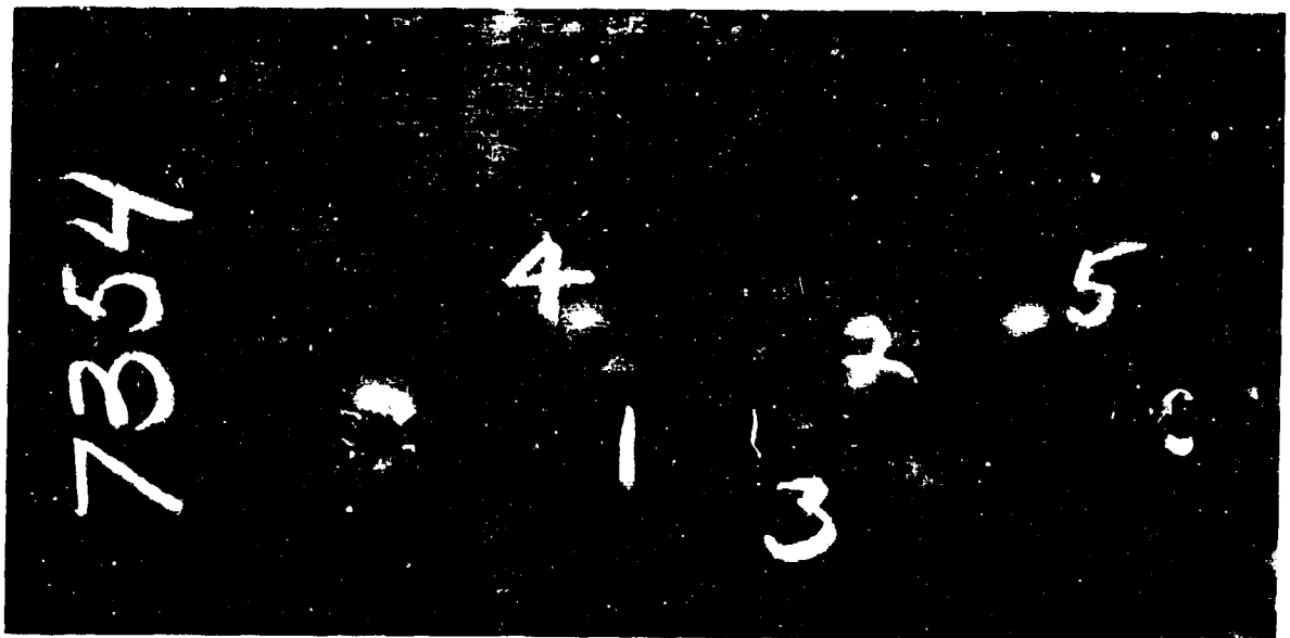
Figure 57. Heat No. 7354. Back of plate after ballistic tests. Ballistic limit: 2300 feet per second, .30 cal. A. P. bullet. Average Brinell-358. Photograph 1/2 Actual Size.
