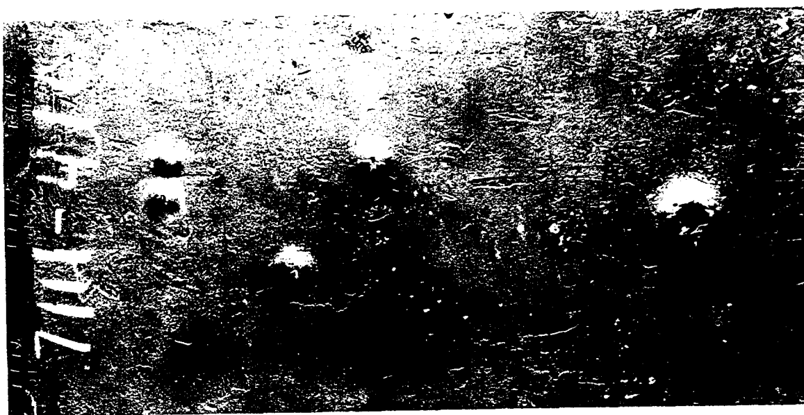
Figure 69. Heat No. 7111:410. Back of as rolled plate after ballistic tests. Ballistic limit: 2445 ft. per sec. Cal. .30 AP. bullet. Rockwell "C" cross-section hardness survey: 43, 43, 43, 43, 43, 43, 43, 43. Composition: Carbon .46%, Silicon .20%, Manganese 1.58%, Vanadium .10/.20%. Average equivalent Brinell 404. Photograph 1/2 actual size.
