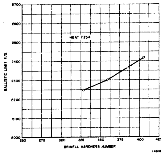
Figure 98. Heat No. 7354. Relationship of ballistic limit to Brinell hardness.
