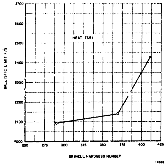
Figure 96. Heat No. 7351. Relationship of ballistic limit to Brinell hardness.
