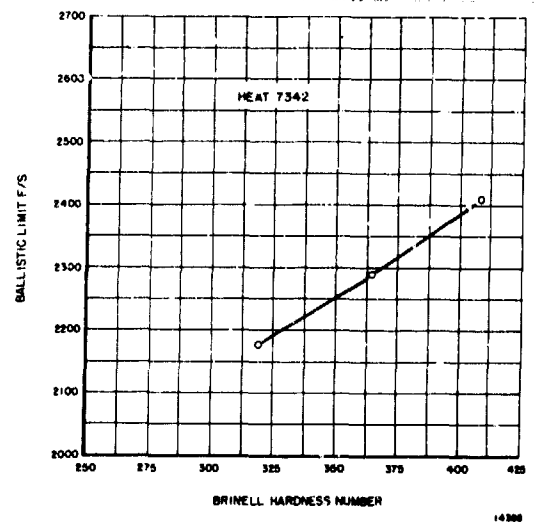
Figure 91. Heat No. 7342. Relationship of ballistic limit to Brinell hardness.
