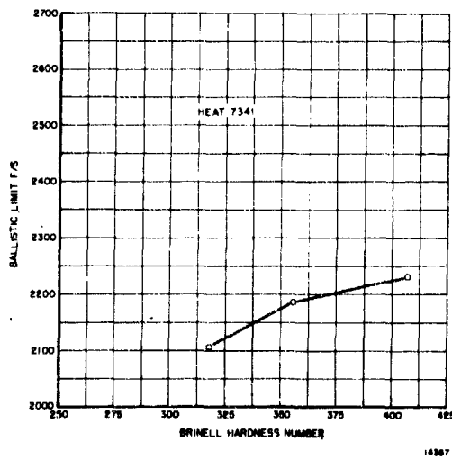
Figure 90. Heat No. 7341. Relationship of ballistic limit to Brinell hardness.
