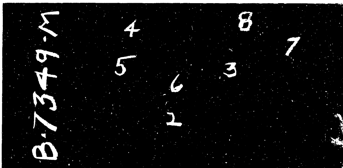
Figure 52. Heat No. 7349. Back of machined plate after ballistic tests. Ballistic limit: 2260 feet per second, .30 cal. A. P. bullet. Rockwell "C" cross-section hardness survey: 37, 36, 35, 37, 37, 35, 36. Average equivalent Brinell-332. Photograph 1/2 Actual Size.
