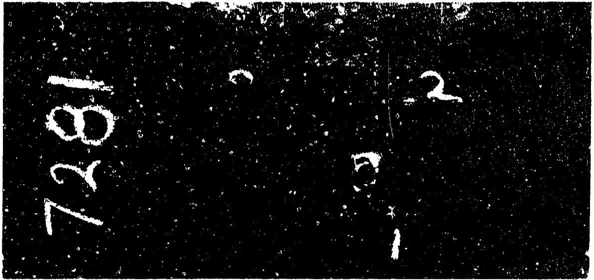
Figure 38. Heat No. 7281. Back of plate after ballistic tests. Ballistic limit: 2275 feet per second, .30 cal. A. P. bullet. Average Brinell- 369. Photograph 1/2 Actual Size.
