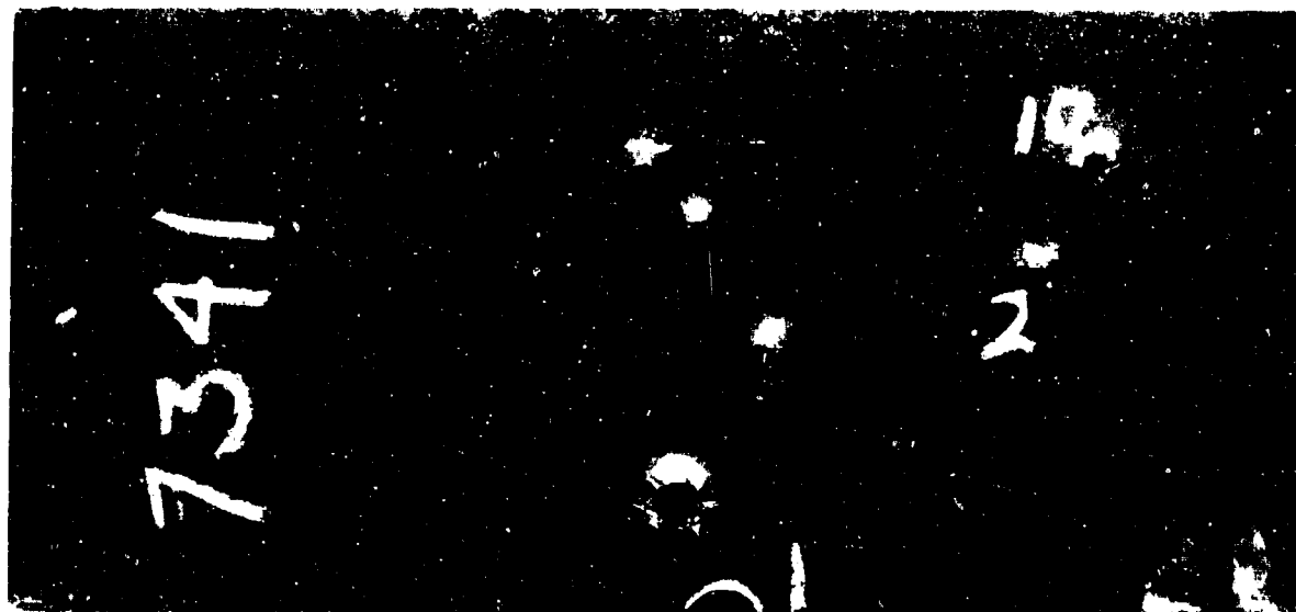
Figure 45. Heat No. 7341. Back of plate after ballistic tests. Ballistic limit: 2181 feet per second, .30 cal. A. P. bullet. Average Brinell-355. Photograph 1/2 Actual Size.
