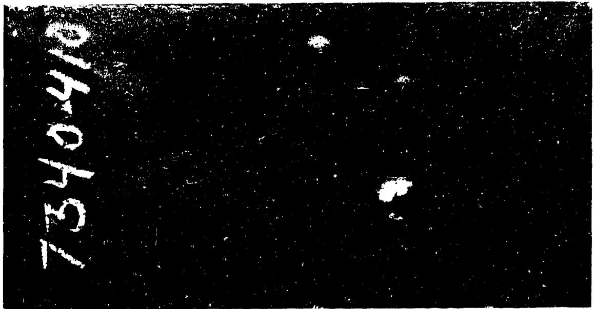
Figure 74. Heat No. 7340:410. Back of as rolled plate after ballistic tests. Ballistic limit: 2383 ft. per sec. Cal. .30 AP. bullet. Rockwell "C" cross-section hardness survey: 45, 44, 44, 45, 44, 44, 44,. Composition: Carbon .46% Manganese .84% Silicon .29% Molybdenum .25/.35. Average equivalent Brinell 418. Photograph 1/2 actual size.
