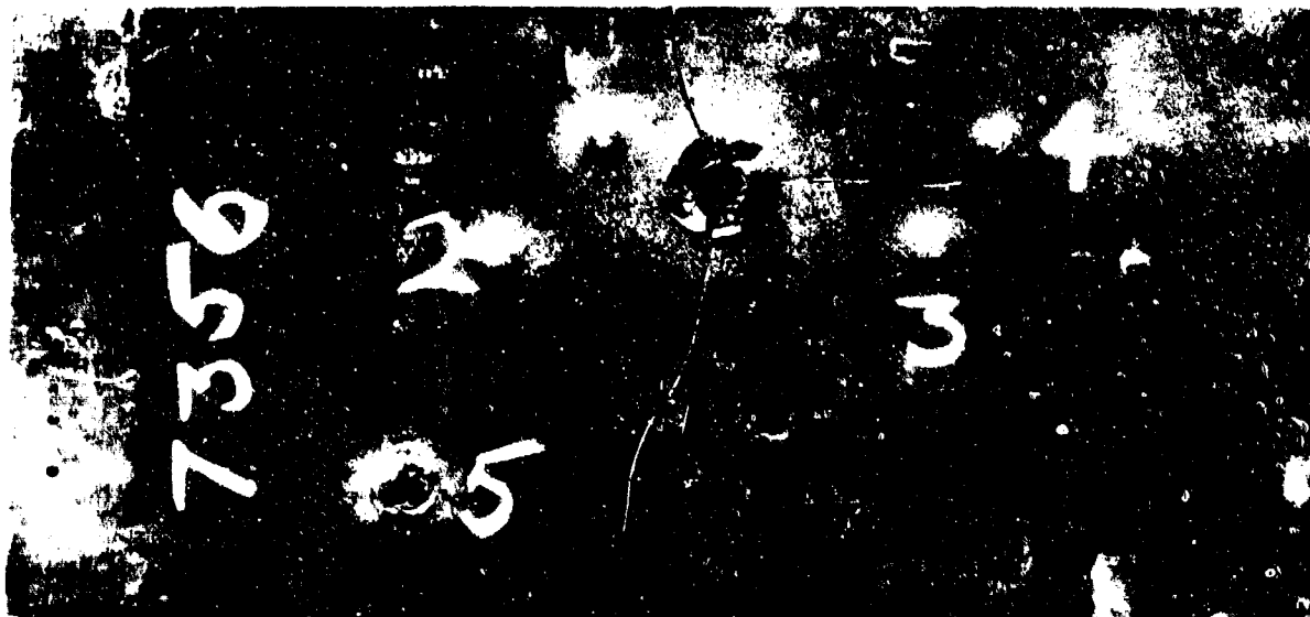
Figure 59. Heat No. 7356. Back of plate after ballistic tests. Ballistic limit: 2300 feet per second, .30 cal. A. P. bullet. Average Brinell-365. Photograph 1/2 Actual Size.
