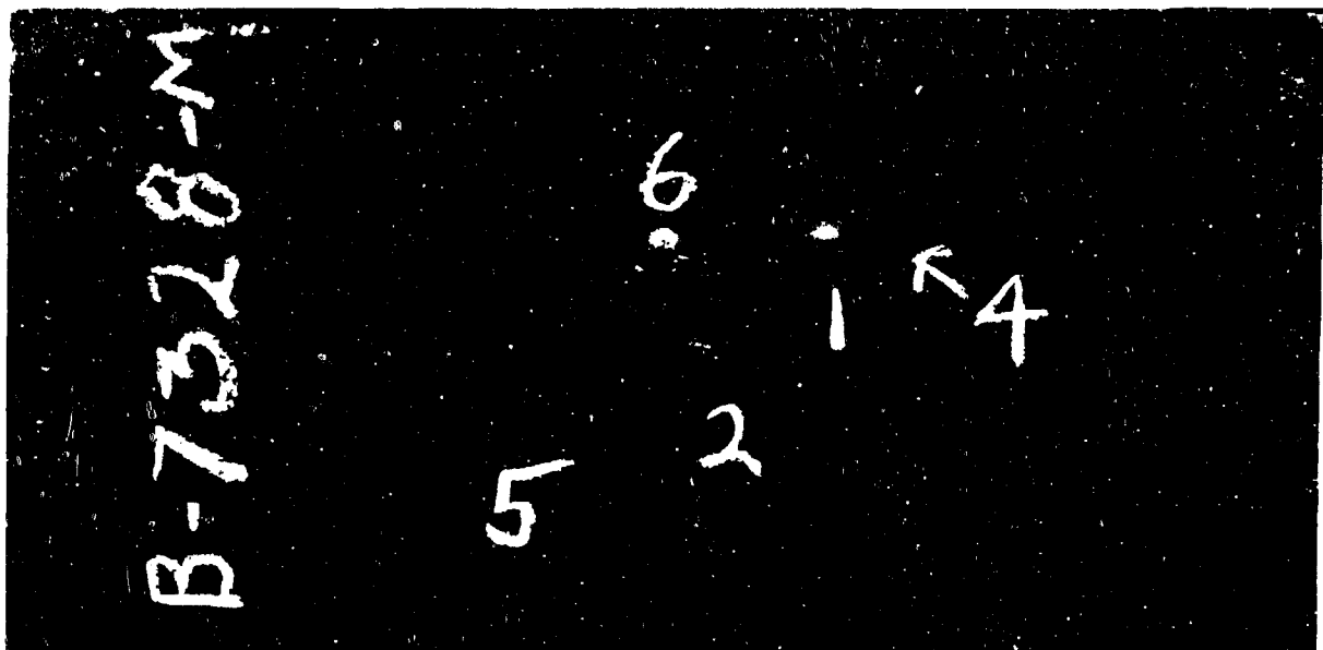
Figure 41. Heat No. 7328. Back of machined plate after ballistic tests. Ballistic limit: 2237 feet per second, .30 cal. A. P. bullet. Rockwell "C" cross-section hardness survey: 38, 38, 38, 38, 38, 38, 38. Average equivalent Brinell-352. Photograph 1/2 Actual Size.
