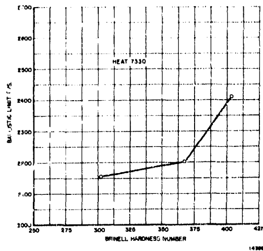
Figure 88. Heat No. 7330. Relationship of ballistic limit to Brinell hardness.
