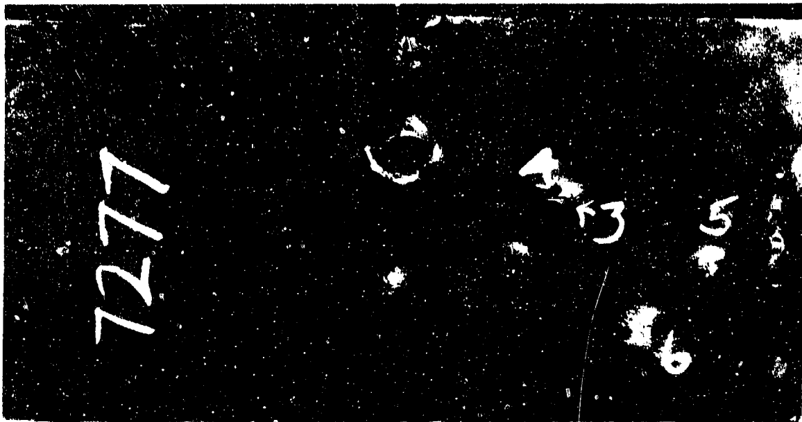
Figure 34. Heat No. 7277. Back of plate after ballistic tests. Ballistic limit: 2142 feet per second, .30 cal.A. P. bullet. Average Brinell-366. Photograph 1/2 Actual Size.
