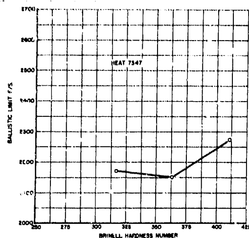
Figure 93. Heat No. 7347. Relationship of ballistic limit to Brinell hardness.
