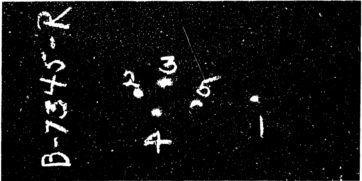
Figure 66. Heat No. 7345. Back of as rolled plate after ballistic tests. Ballistic limit 2287 feet per second, .30 cal. A. P. bullet. Rockwell "C" cross-section hardness survey: 36, 37, 37, 37, 37, 37, 36. Average equivalent Brinell-342. Photograph 1/2 Actual Size.
