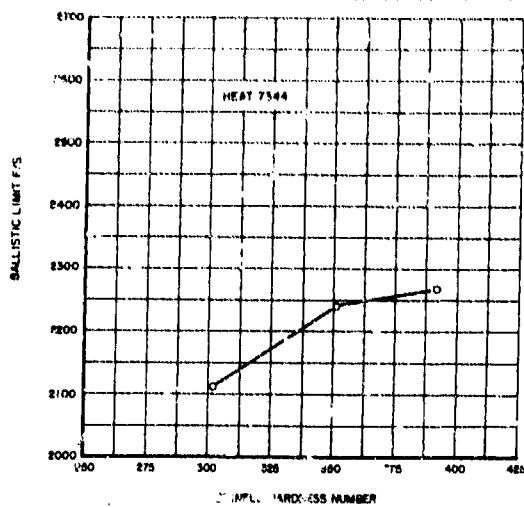
Figure 92. Heat No. 7344. Relationship of ballistic limit to Brinell hardness.
