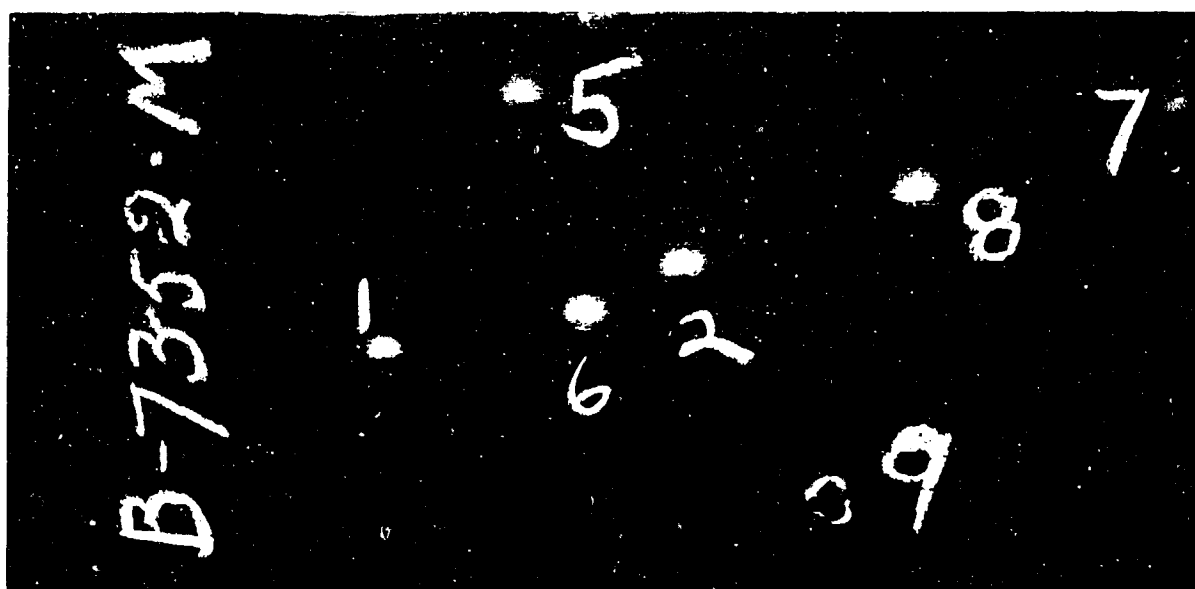
Figure 55. Heat No. 7352. Back of machined plate after ballistic tests. Ballistic limit: 2242 feet per second, .30 cal. A. P. bullet. Rockwell "C" cross-section hardness survey: 38, 38, 38, 37, 38, 38, 38. Average equivalent Brinell-352. Photograph 1/2 Actual Size.
