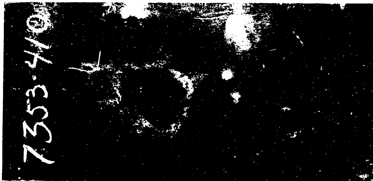
Figure 81. Heat No. 7353:410. Back of as rolled plate after ballistic tests. Ballistic limit: 2328 ft. per sec. Cal. .30 AP. bullet. Rockwell "C" cross-section hardness survey: 41, 41, 41, 41, 40, 41, 40. Composition: Carbon .45% Manganese .84% Silicon .73%. Average equivalent Brinell 379. Photograph 1/2 actual size.
