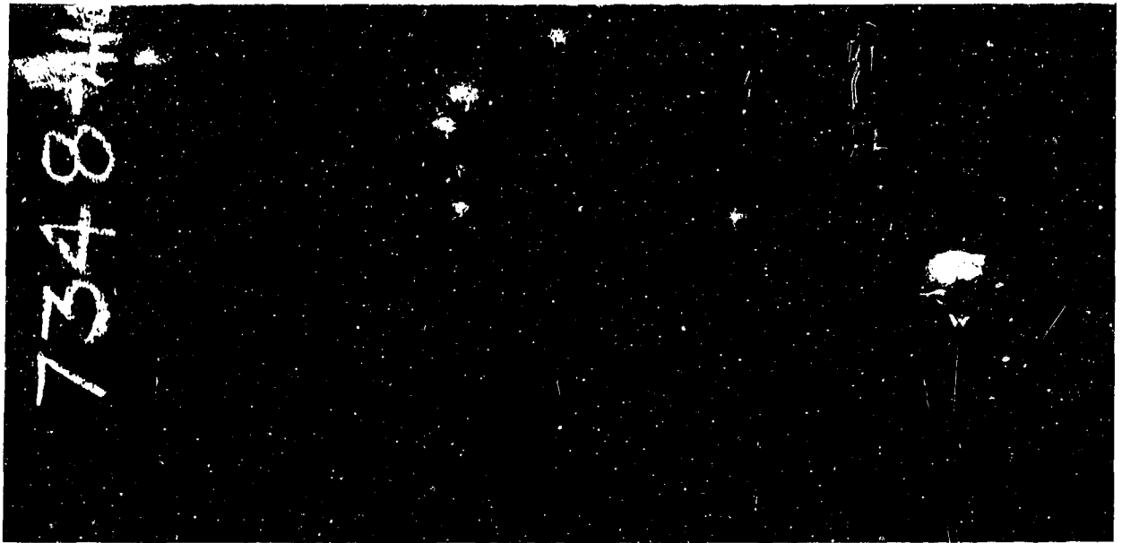
Figure 79. Heat No. 7348:410. Back of as-rolled plate after ballistic tests. Ballistic limit: 2345 ft. per sec. Cal. .30 AP. bullet. Rockwell "C" cross-section hardness survey: 41, 41, 42, 43, 44, 44, 45. Composition: Carbon .47% Manganese 1.48% Silicon .32% Molybdenum .40/.50% Copper .30/.50% Average equivalent Brinell 402. Photograph 1/2 actual size.
