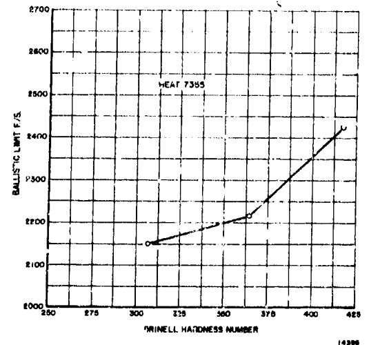
Figure 99. Heat No. 7355. Relationship of ballistic limit to Brinell hardness.
