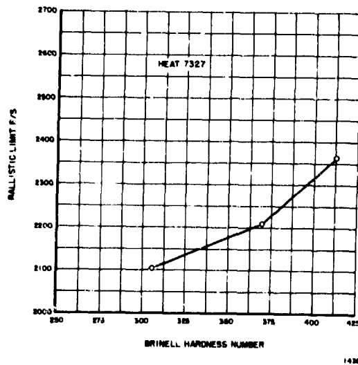
Figure 86. Heat No. 7327. Relationship of ballistic limit to Brinell hardness.
