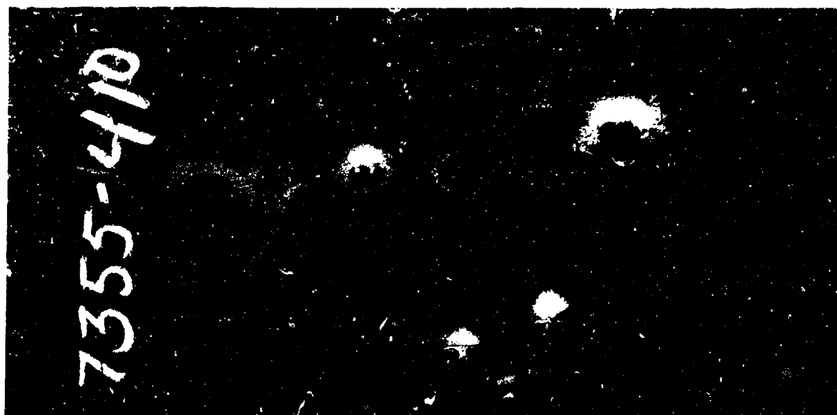
Figure 83. Heat No. 7355:410. Back of as rolled plate after ballistic tests. Ballistic limit: 2427 ft. per sec. Cal. .30 AP bullet. Rockwell "C" cross-section hardness survey: 45, 44, 45, 43, 44, 45, 44. Composition Carbon .46% Manganese .78% Silicon 1.06% Molybdenum .40/.80%. Average equivalent Brinell 417. Photograph 1/2 actual size.
