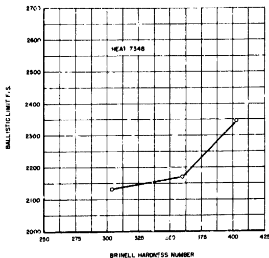
Figure 94. Heat No. 7348. Relationship of ballistic limit to Brinell hardness.
