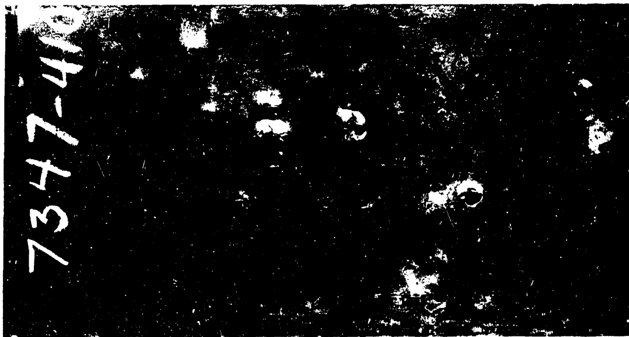
Figure 78. Heat No. 7347:410. Back of as rolled plate after ballistic tests. Ballistic limit: 2274 ft. per sec. Cal. .30 AP. bullet. Rockwell "C" cross-section hardness survey: 34, 38, 33, 33, 34, 34, 34. Composition: Carbon .34% Manganese .83% Silicon .26% Chromium .90/1.10% Copper 1.4/1.6%. Average equivalent Brinell 410. Photograph 1/2 actual size.
