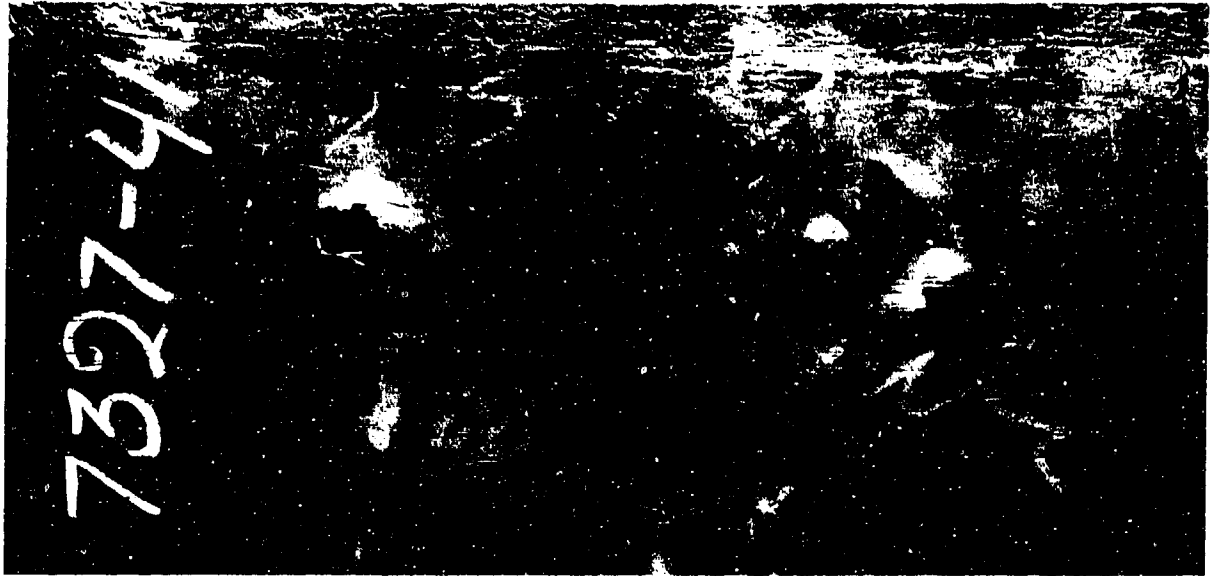
Figure 71. Heat No. 7327:410. Back of as rolled plate after ballistic tests. Ballistic limit: 2362 ft. per sec. Cal. .30 AP. bullet. Rockwell "C" cross-section hardness survey: 43, 43, 44, 44, 44, 44, 44. Composition: Carbon .35% Manganese .88% Silicon .26% Chromium 2.3/2.7%. Average equivalent Brinell 412. Photograph 1/2 actual size.
