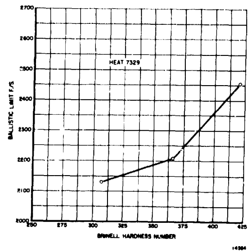
Figure 87. Heat No. 7329. Relationship of ballistic limit to Brinell hardness.
