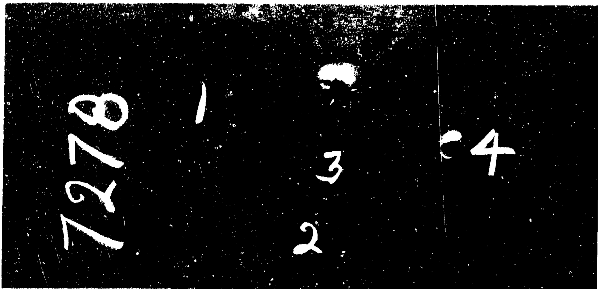
Figure 35. Heat No. 7278. Back of plate after ballistic tests. Ballistic limit: 2250 feet per second, .30 cal. A. P. bullet. Average Brinell-369. Photograph 1/2 Actual Size.
