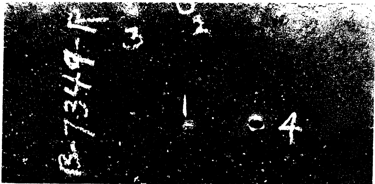
Figure 67. Heat No. 7349. Back of plate after ballistic tests. Ballistic limit: 2309 feet per second, .30 cal. A. P. bullet. Rockwell "C" cross-section hardness survey: 39, 39, 39, 39, 39, 39, 39. Average equivalent Brinell-362. Photograph 1/2 Actual Size.
