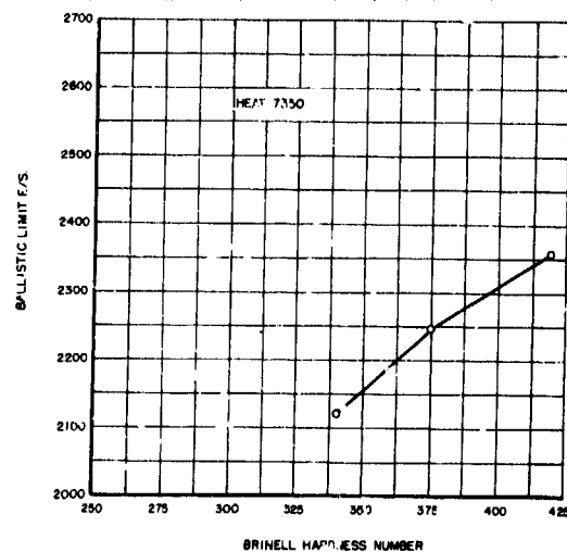
Figure 95. Heat No. 7350. Relationship of ballistic limit to Brinell hardness.
