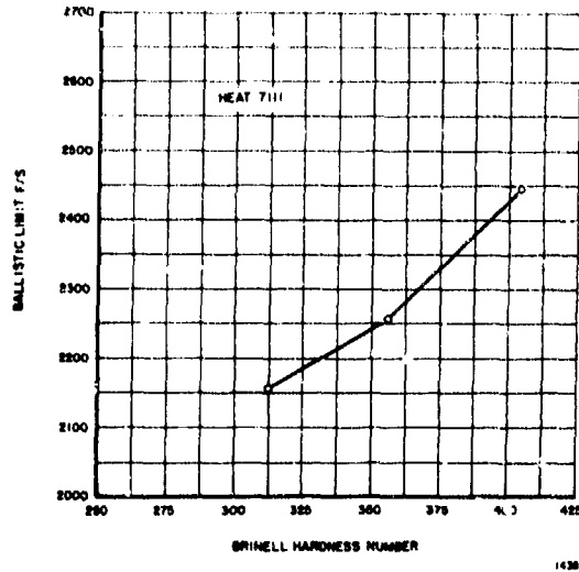
Figure 84. Heat No. 7111. Relationship of ballistic limit to Brinell hardness.
