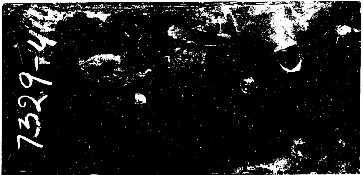
Figure 72. Heat No. 7329:410. Back of as rolled plate after ballistic tests. Ballistic limit: 2455 ft. per sec. Cal. .30 AP bullet. Rockwell "C" cross-section hardness survey: 44, 45, 45, 45, 45, 44. Composition: Carbon .34% Manganese .88% Silicon .25% Chromium 1.3/1.7% Vanadium .10/.20 Average equivalent Brinell 421. Photograph 1/2 actual size.
