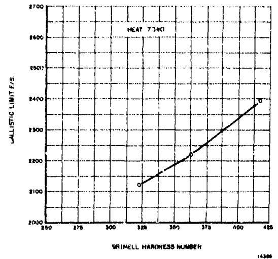
Figure 89. Heat No. 7340. Relationship of ballistic limit to Brinell hardness.
