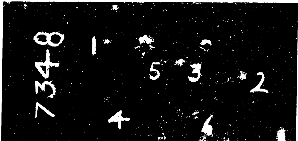
Figure 51. Heat No. 7348. Back of plate after ballistic tests. Ballistic limit: 2170 feet per second, .30 cal. A. P. bullet. Average Brinell-369. Photograph 1/2 Actual Size.
