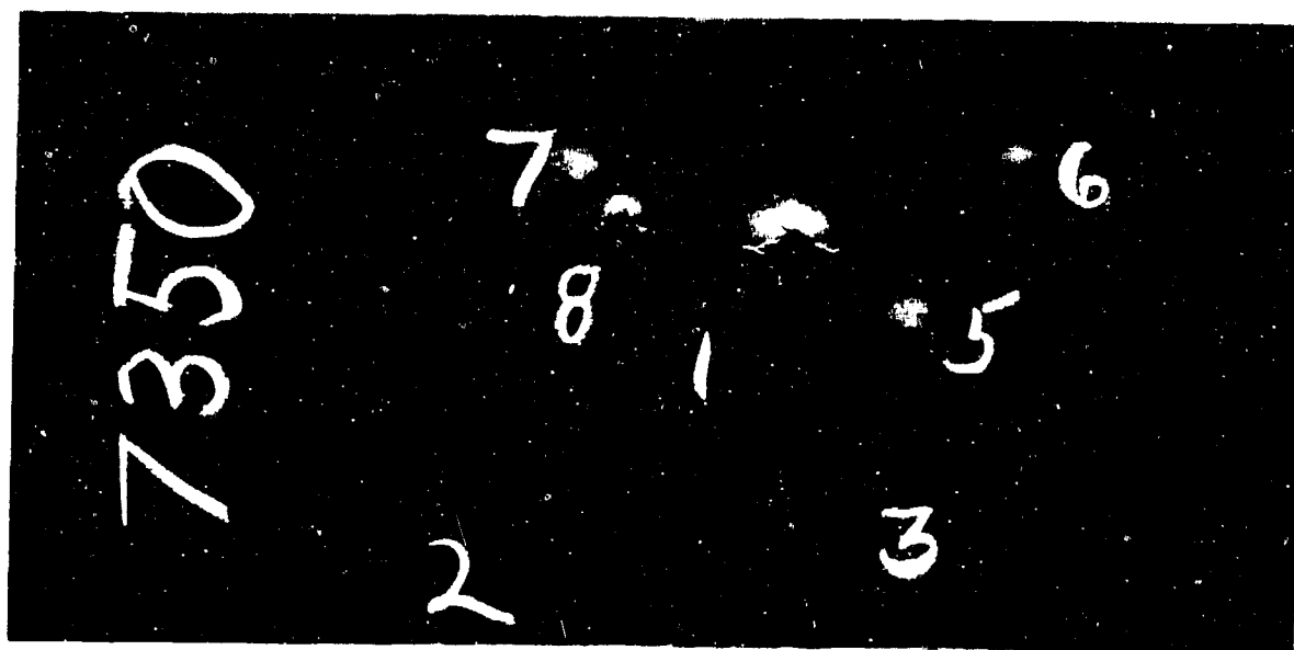
Figure 53. Heat No. 7350. Back of plate after ballistic tests. Ballistic limit: 2246 feet per second, .30 cal. A. P. bullet. Average Brinell-375. Photograph 1/2 Actual Size.
