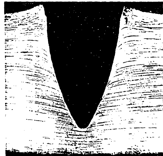
D. Static Penetration No. SS-21372 Bullet - Cal. .30 Core Pushed into Plate under Head of Tensile Machine
