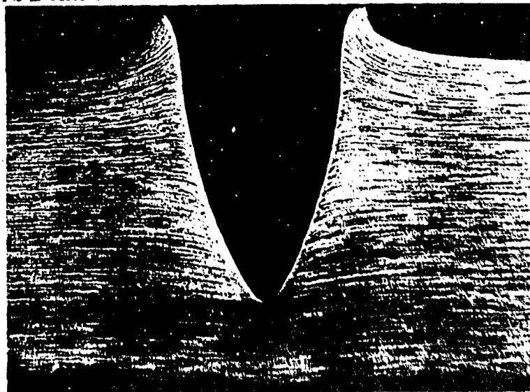
E. Impact Penetration Velocity - 1875 Ft/sec. No. 1113/2042 Bullet - Cal. .30 Core (Duplated) Fired from Smith Baro Rifle
