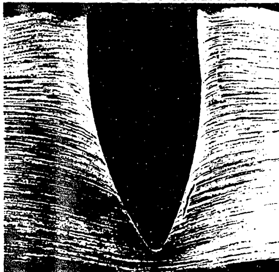
C. Impact Penetration No. SS31-2150 Velocity - 2150 Ft/sec. Bullet - Cal. .40 AP Fired from Mann Barrel
