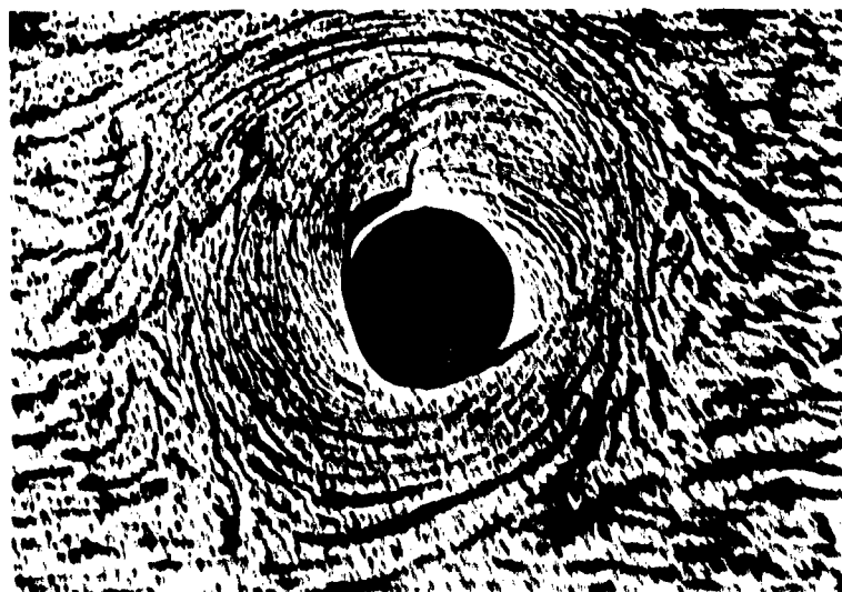
C. Section Parallel to and 0.401" Below Front Surface of Plate and 0.091" Above Back Surface of Plate.
