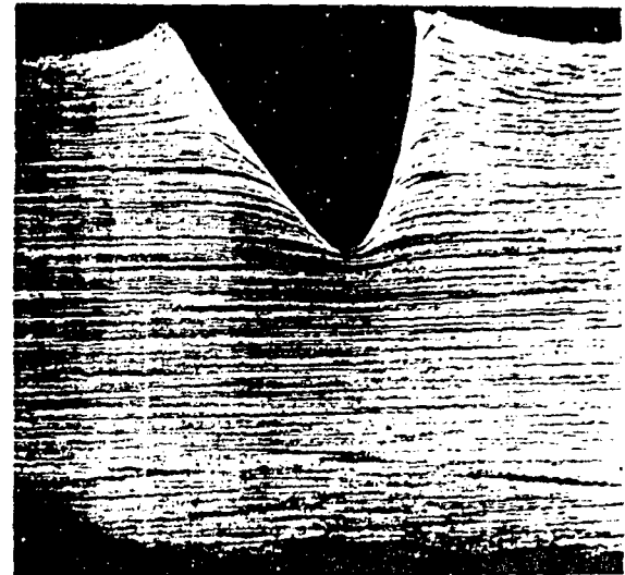
B. Static Penetration No. SS31-CT1 Bullet - Cal. .30 Core Pushed into Plate under Head of Tensile Machine
