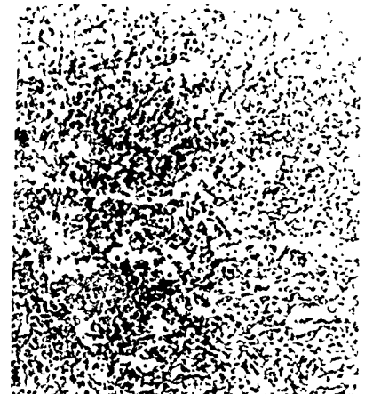
-C- X1000 Martensite, undissolved carbides and ferrite.
