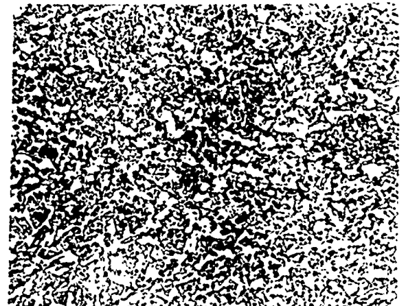
-E- X1000 Martensite, undissolved carbides, and ferrite. Hardness - Rc 40.5.
