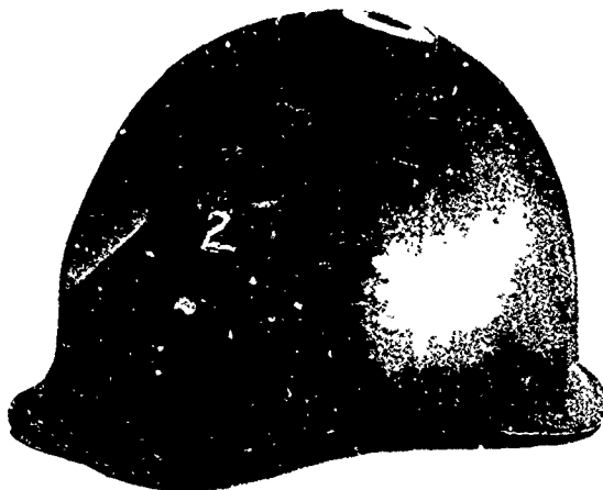
American helmet No. 15. McCord Lot 595E. Tested with caliber .45 ball ammunition. Ballistic limit - 948 ft./sec. Note ductile behavior.
