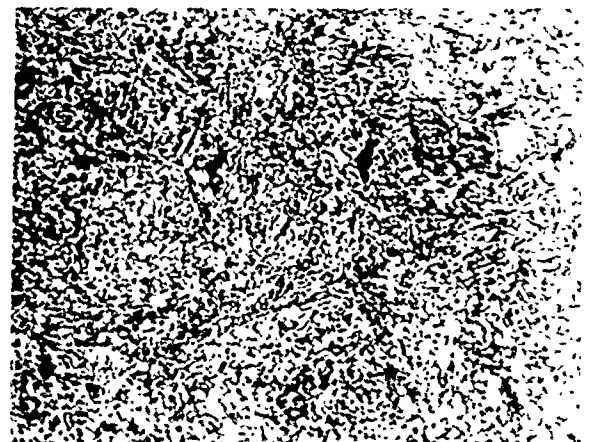
-G- X1000 Completely martensitic microstructure. Hardness - Rc 49.5
