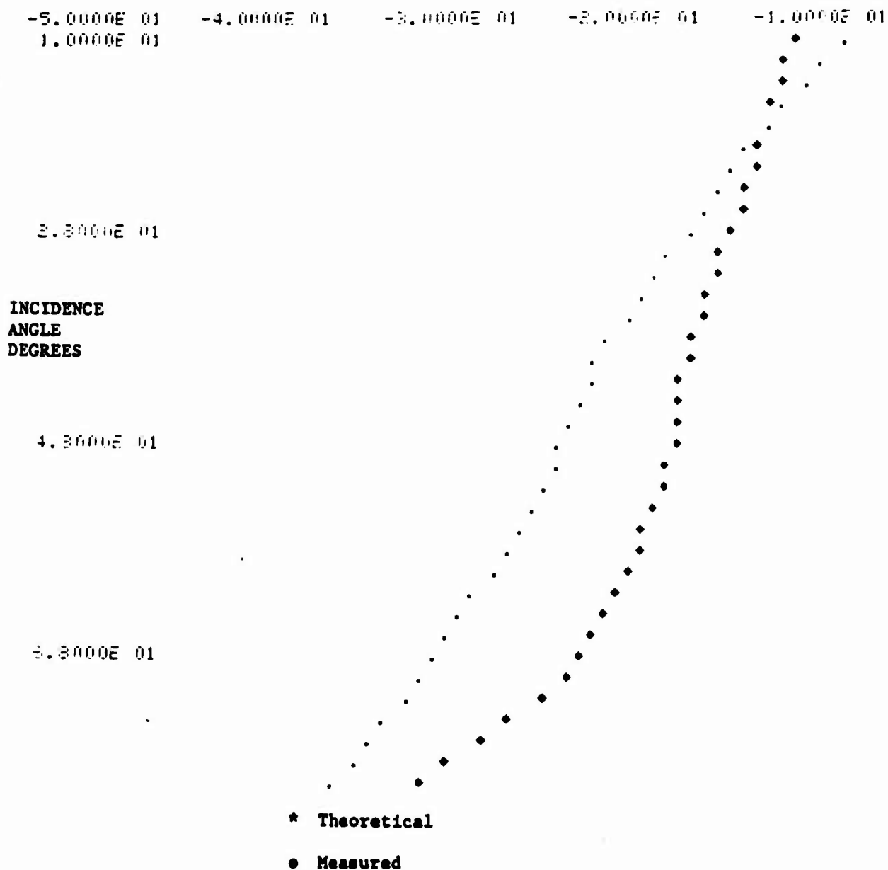
Figure C-9-- Backscatter from concrete at K_u band, horizontal polarization
