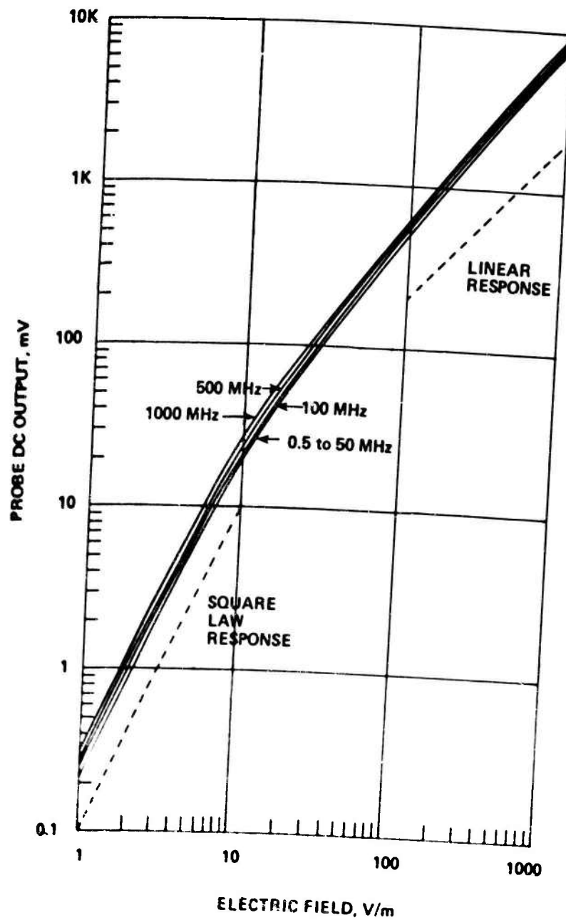
Figure 12. Typical detected output of an EFM-5 dipole as a function of field strength, at several frequencies.
