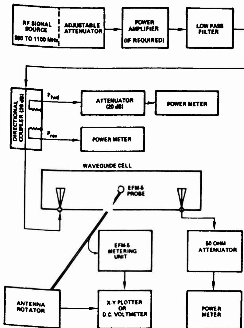
Figure 15. Instrumentation for generating a standard field in a waveguide cell for calibrating an EFM-5 monitor.
