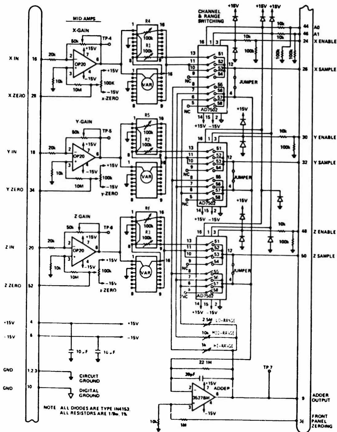
Figure 25. Schematic diagram of the shaping board.
