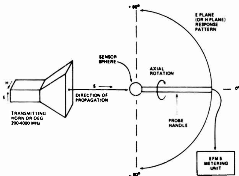
Figure 22. Instrumentation for measuring various response patterns of an rf radiation monitor.
