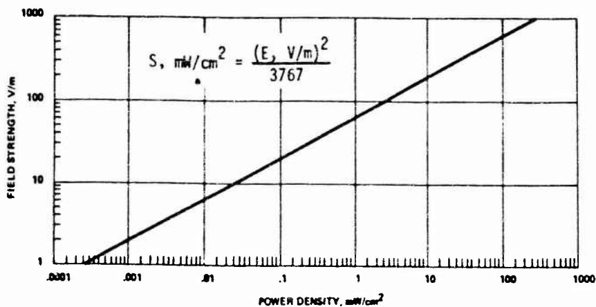
Figure 2. Graph of the EFM-5 field intensity range, comparing units of V/m and mW/cm².
