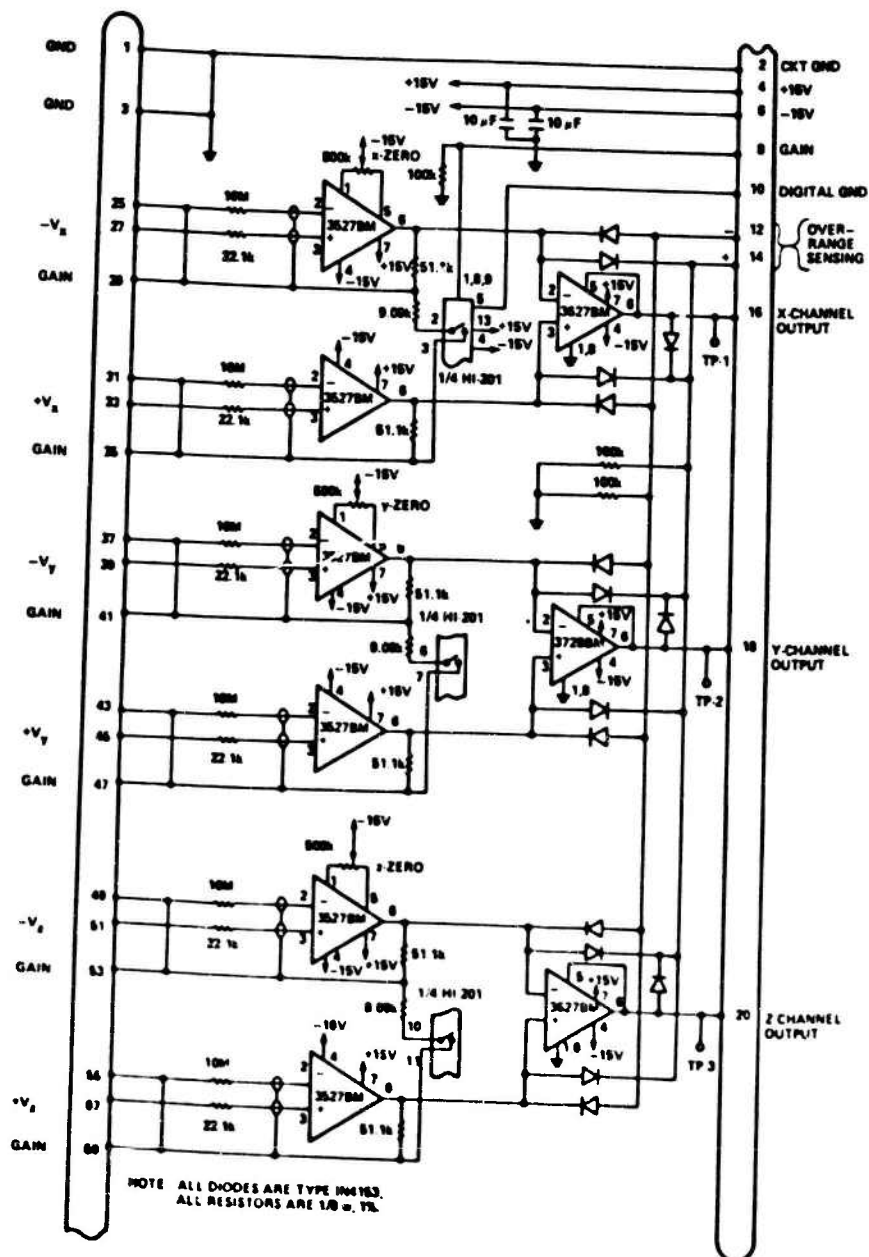
Figure 23. Schematic diagram of the preamplifier board.
