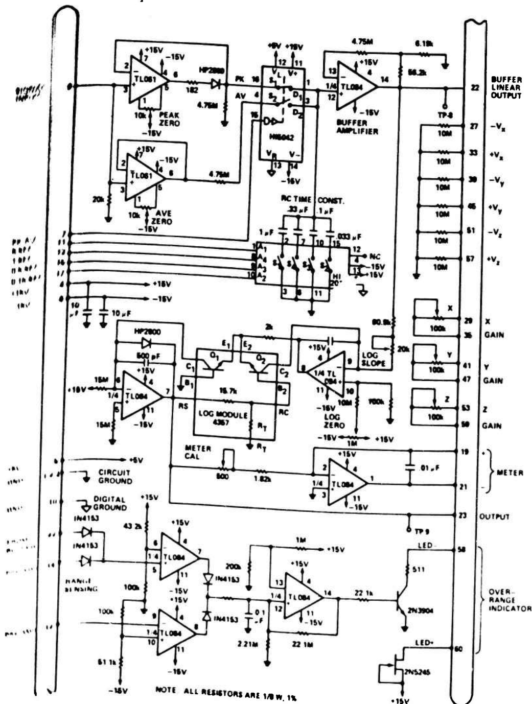
Figure 27. Schematic diagram of the logarithm board.
