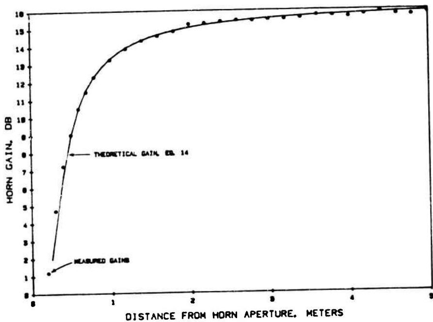
Figure 20. Graph of SGH-0.75 horn gain vs distance at 1000 MHz.
