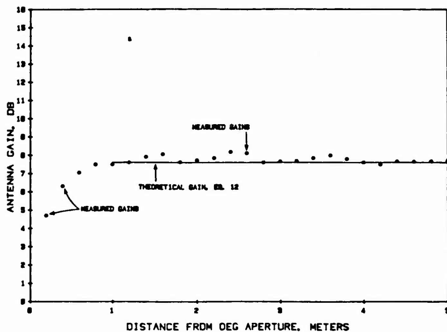
Figure 17. Graph of WR-2100 OEG gain vs distance at 500 MHz.
