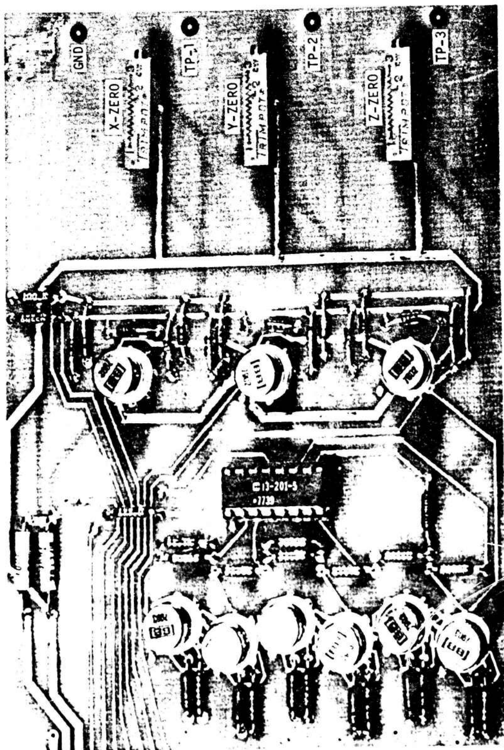
Figure 24. Photograph of the preamplifier board showing the zeroing controls and test points.
