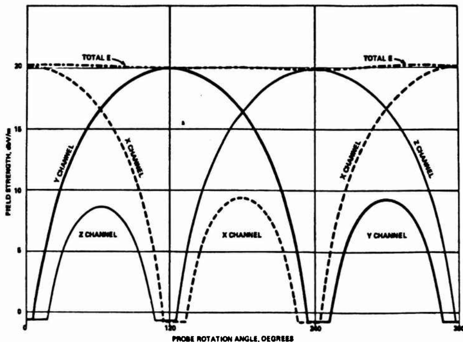
Figure 21. Response pattern of an EFM-5 antenna at 100 MHz and 10 V/m, with the probe handle at the analytic angle.
