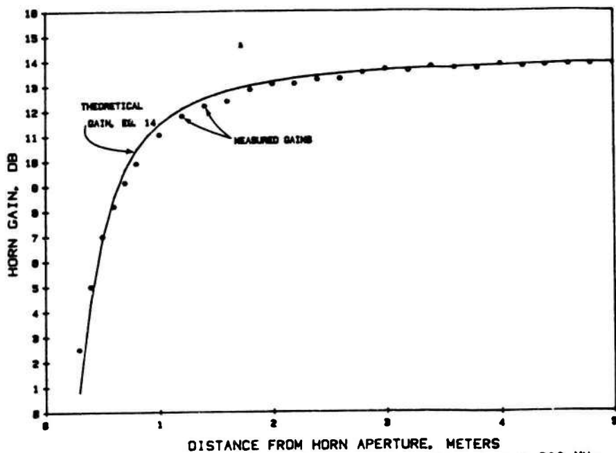
Figure 19. Graph of SGH-0.5 horn gain vs distance at 500 MHz.
