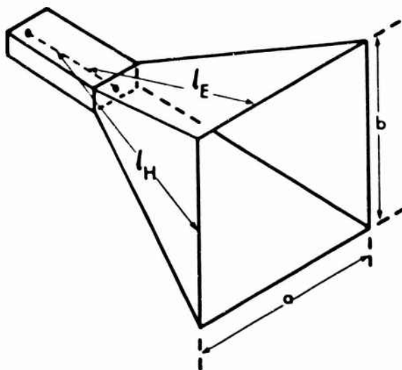
Figure 18. Sketch of a pyramidal horn showing the pertinent dimensions.
