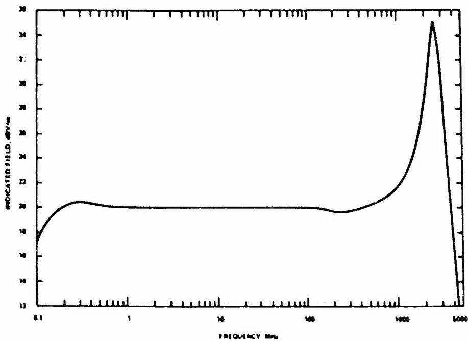
Figure 3. Typical response of an EFM-5 monitor vs frequency, at a field strength of 20 dBV/m (10 V/m).
