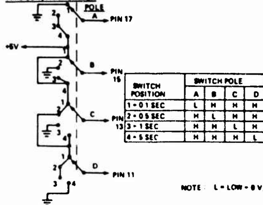
Figure 30. Schematic diagrams of the other front panel controls and components.
