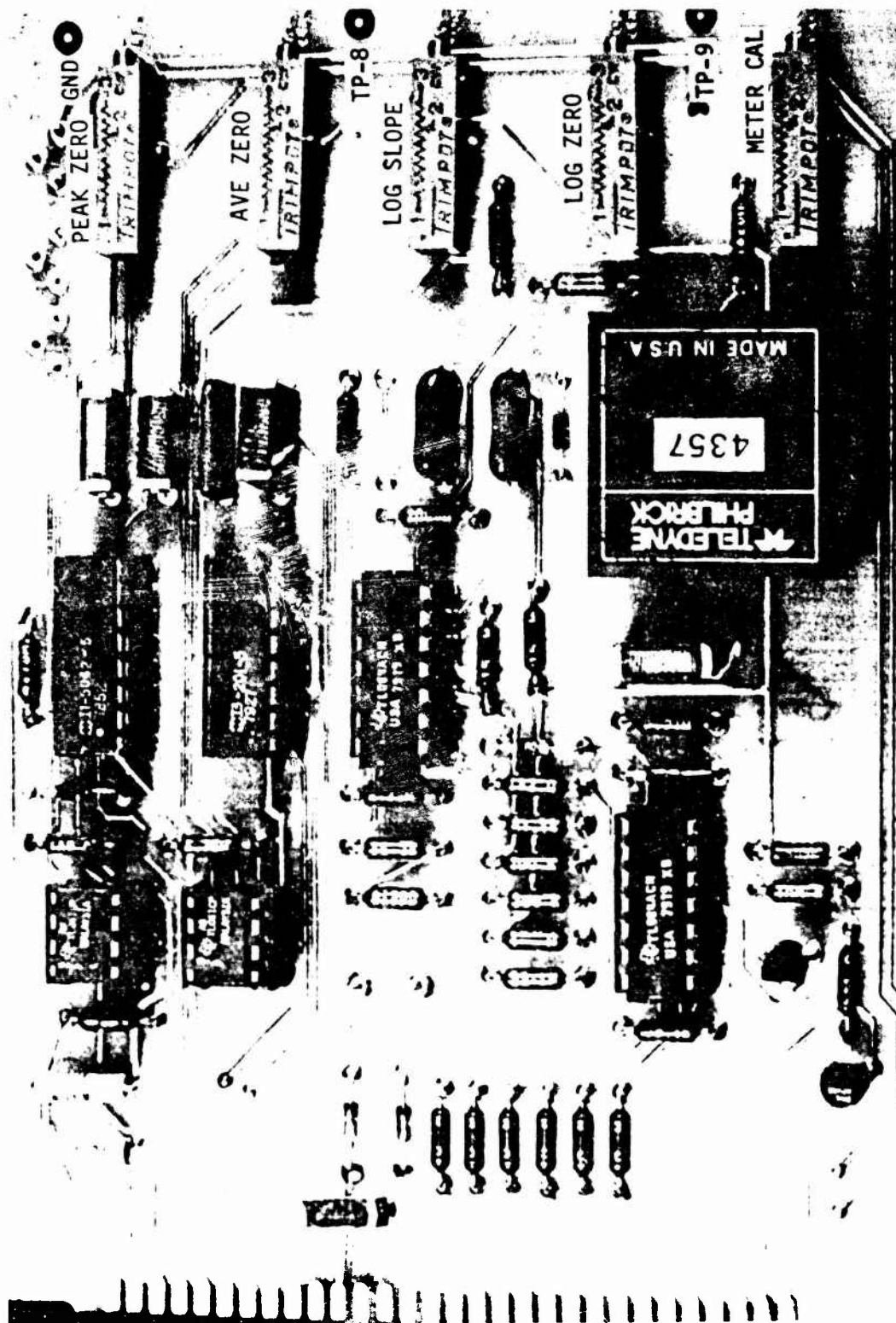
Figure 28. Photograph of the logarithm board showing the zeroing and alignment controls and the test points.
