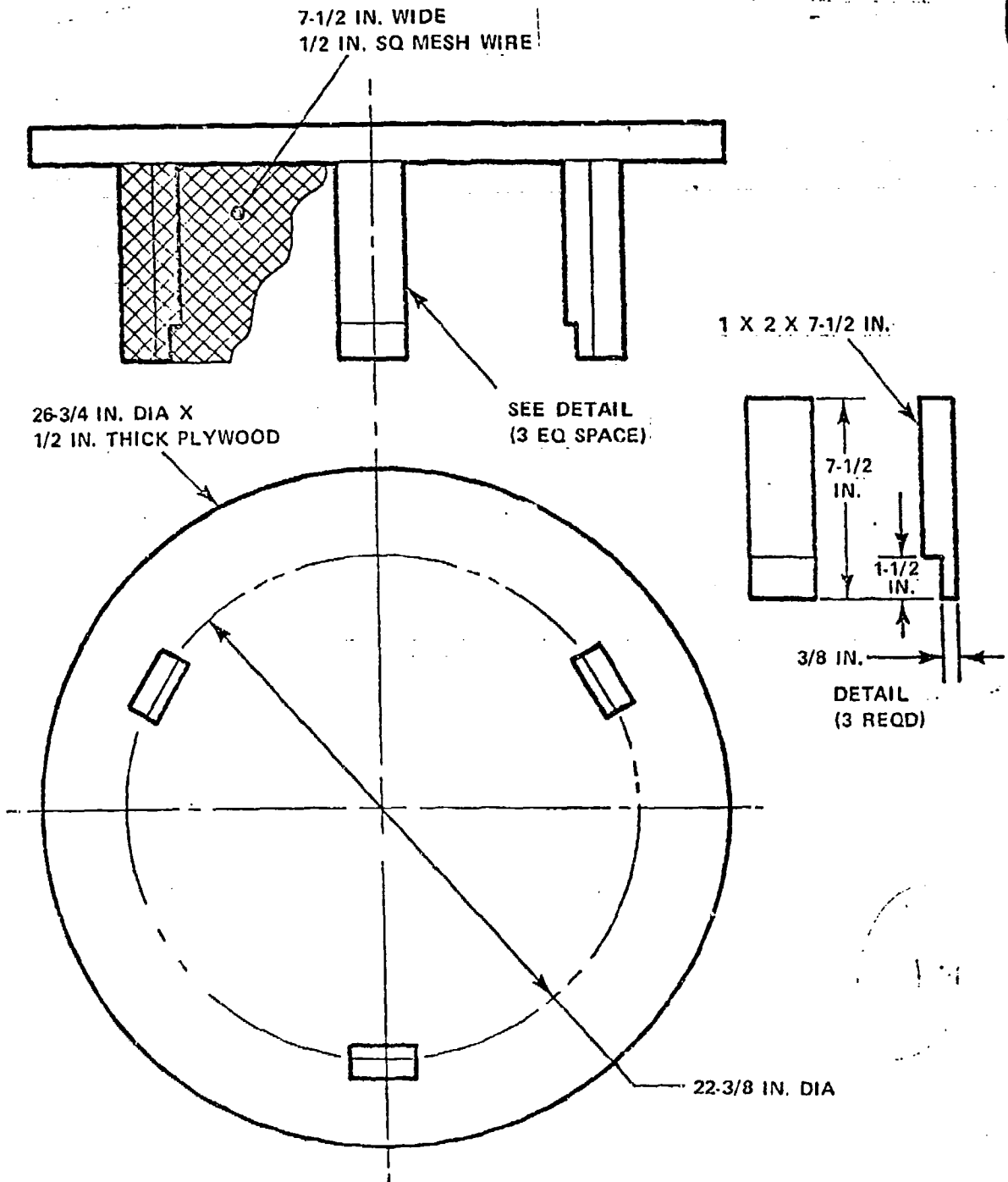
Figure 38. Lysimeter Cover.
