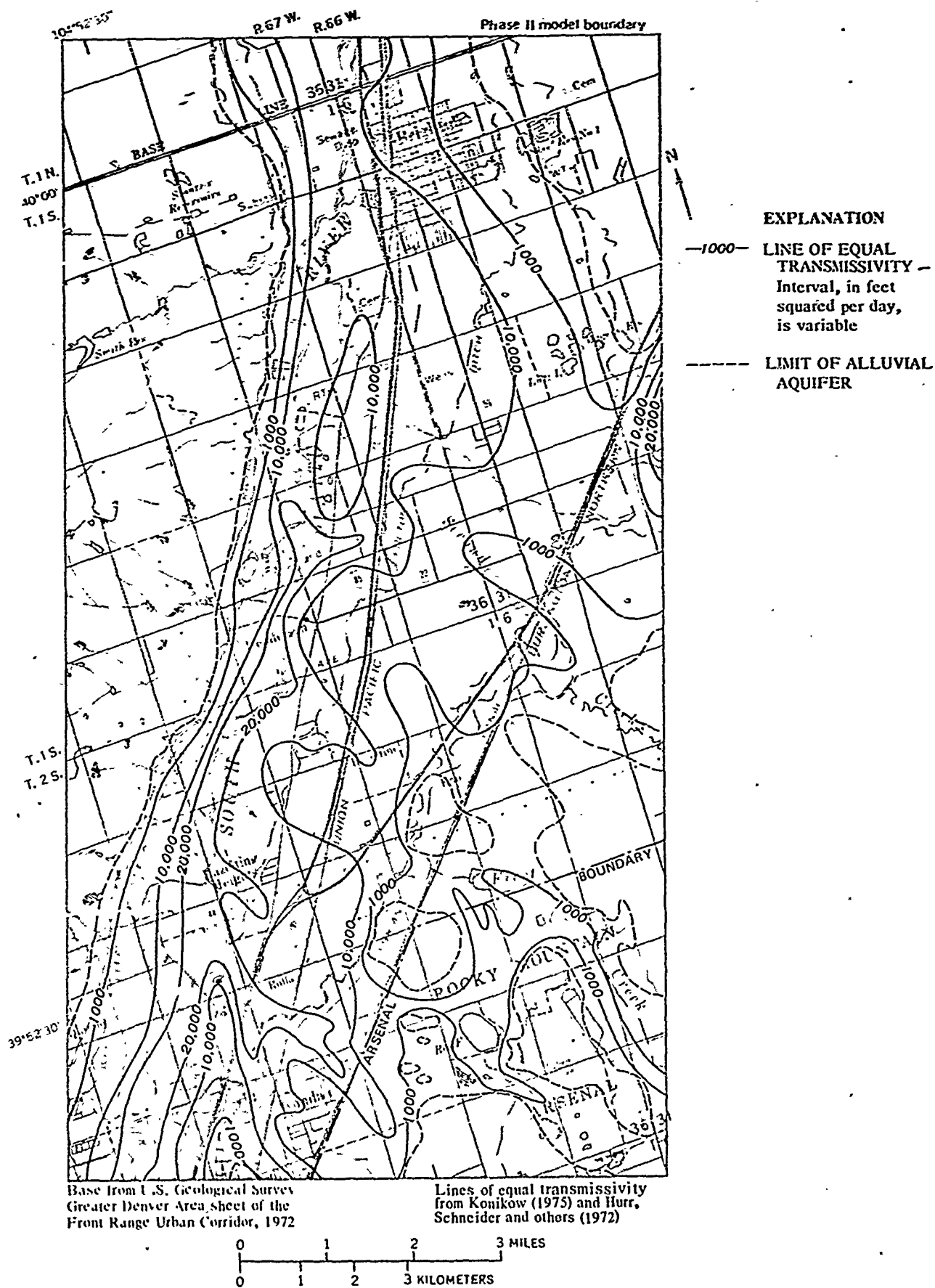
Figure 2.-- Transmissivity of alluvial aquifer.
