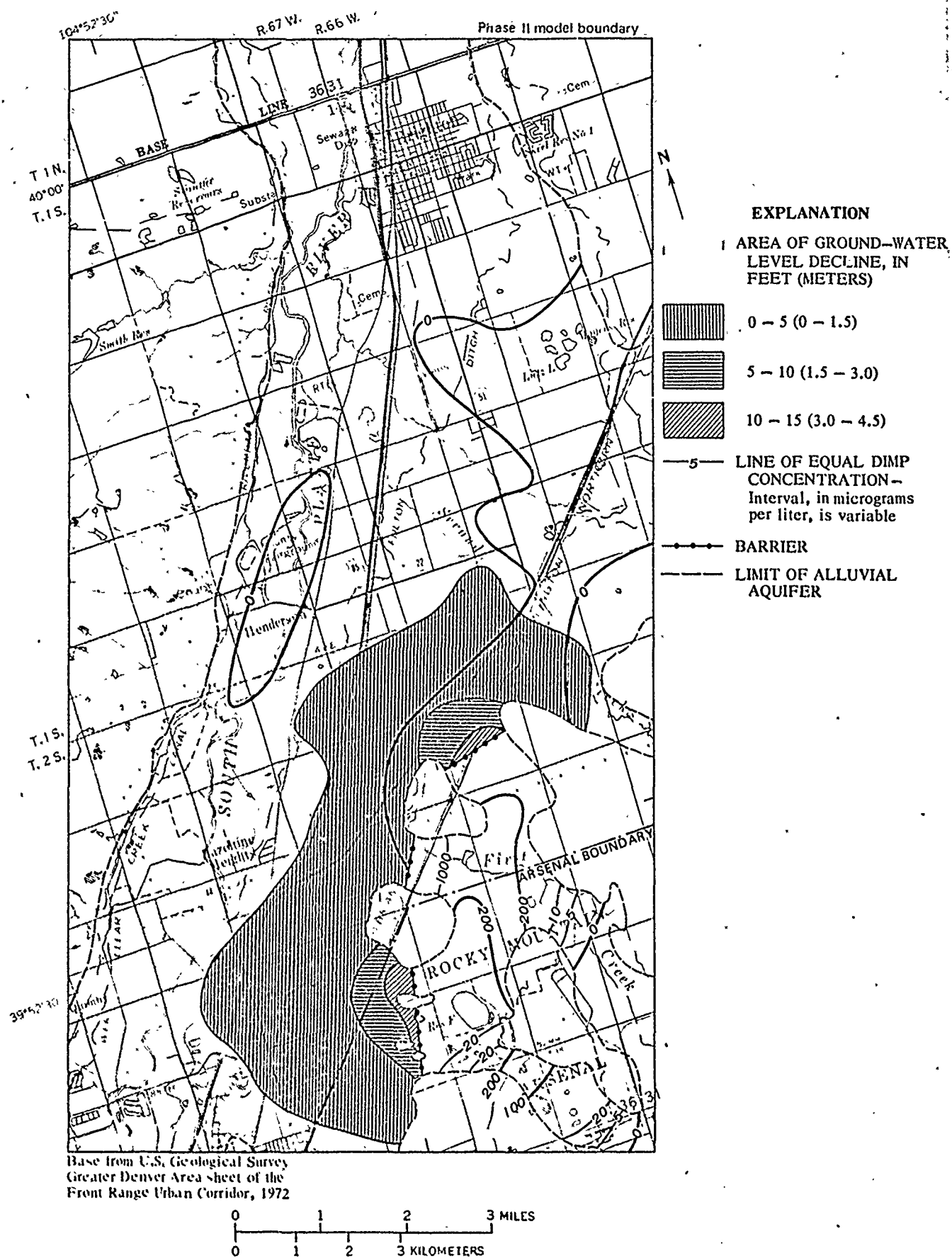
Figure 21.--Phase II model--calculated 1995 DIMP concentrations and water-level decline for Run 6, three barriers near arsenal.
