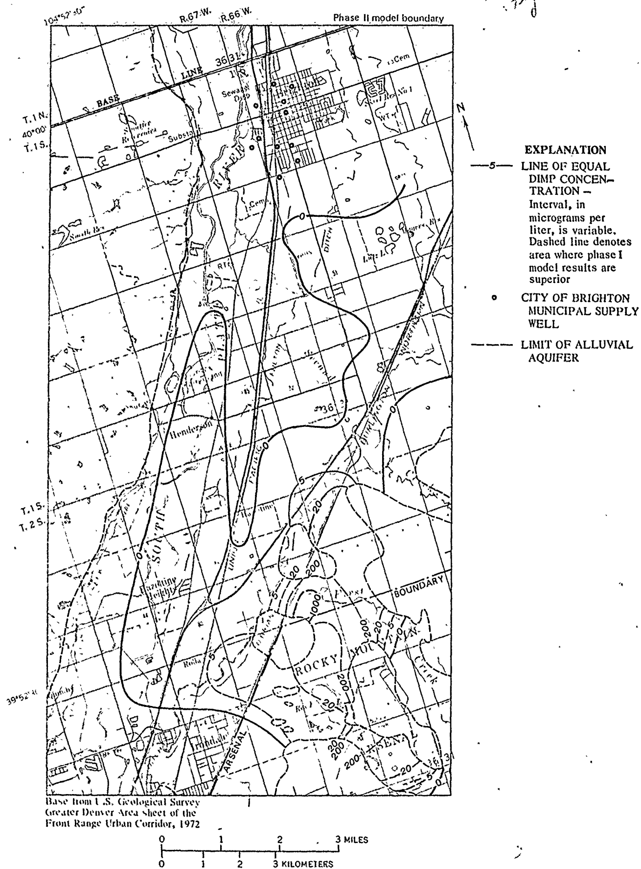
Figure 15.--Phase II model--calculated 1995 DIMP concentrations for Run 1, no remedial measures.
