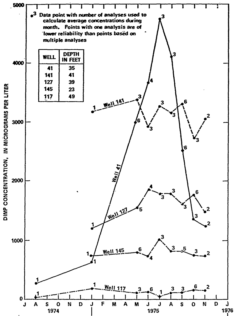
Figure 11.-- Change in DIMP concentration with time in selected wells. (See figure 1 for location of wells)
