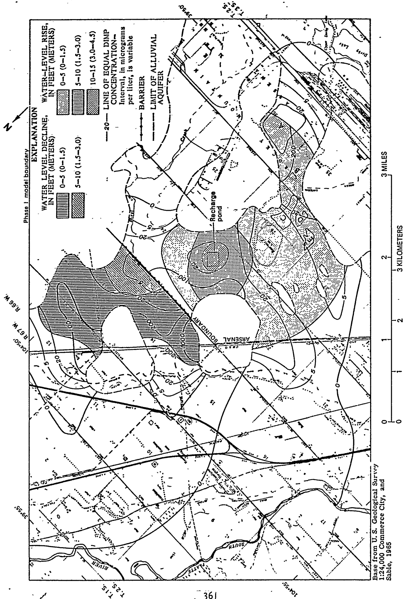
Figure 19.—Phase I model-calculated 1995 DIMP concentrations for run 4, barrier at north arsenal boundary with recharge pond above barrier.
