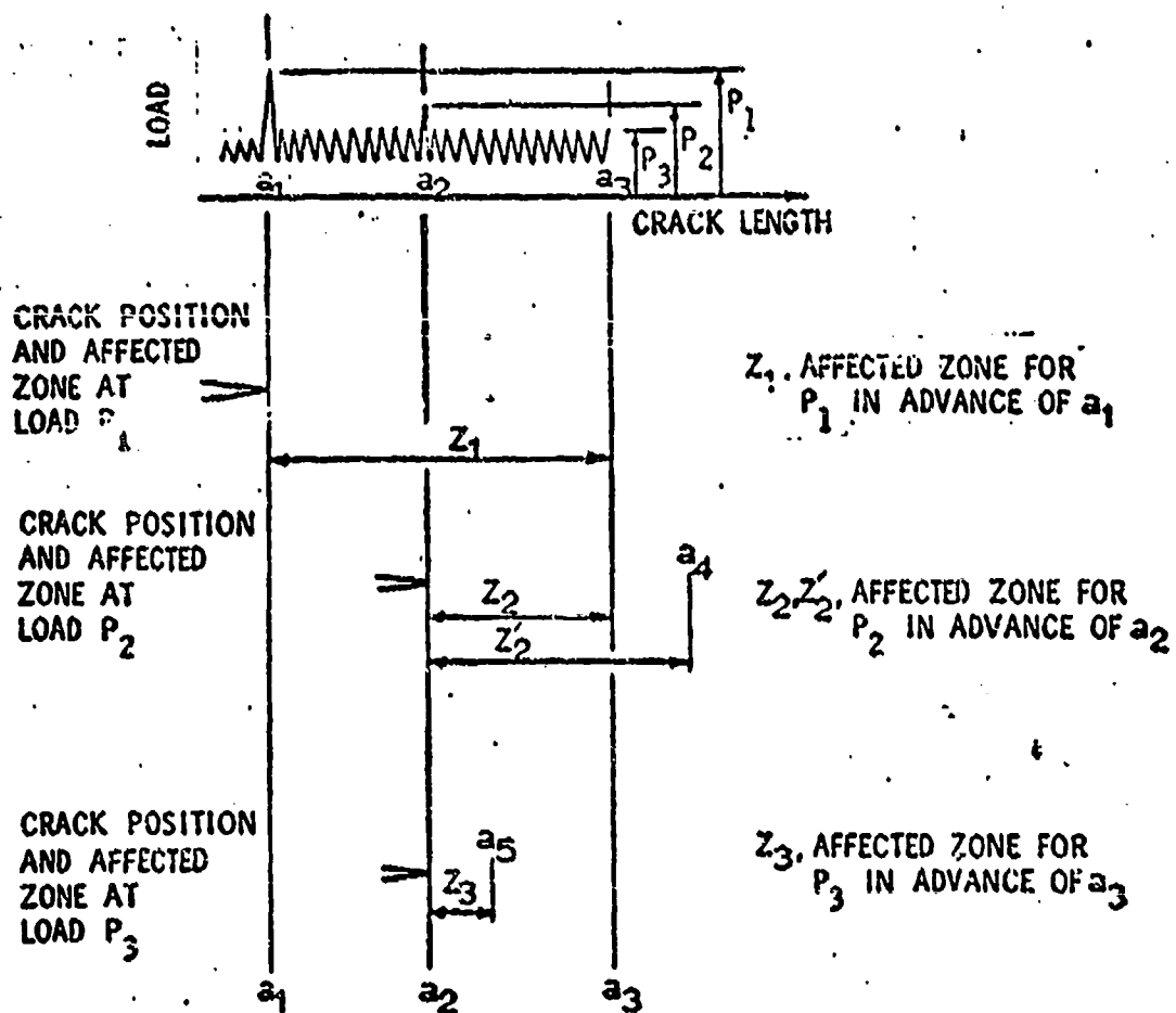
FIGURE 1 SCHEMATIC ILLUSTRATING THE LOAD INTERACTION ZONE CONCEPT
