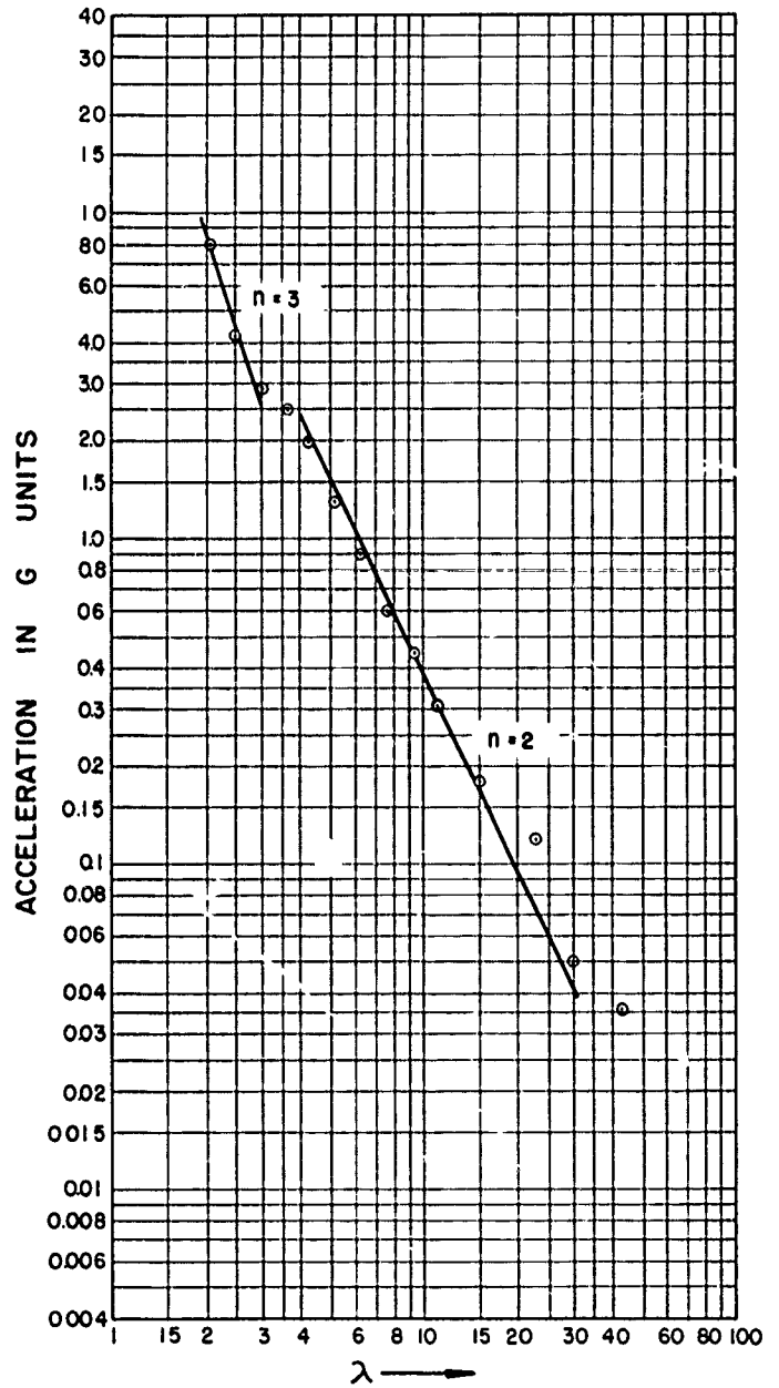
FIGURE 9 HORIZONTAL EARTH ACCELERATION - FIRST PEAK HE - 2
