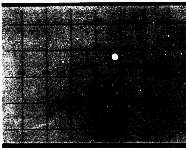
Fig. 4.1 Typical Flash Ranging Picture of Fireball with Grid Lines in Background
