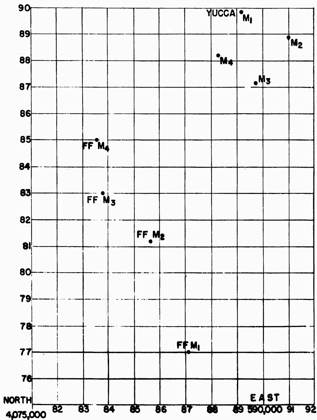
Fig. 3.3 Geophone Locations - UTM Grid Coordinates
