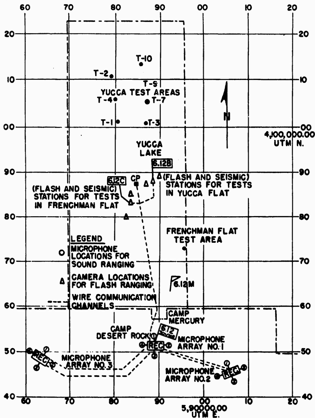
Fig. 2.7 General Layout of Project 6.12 Instrumentation
