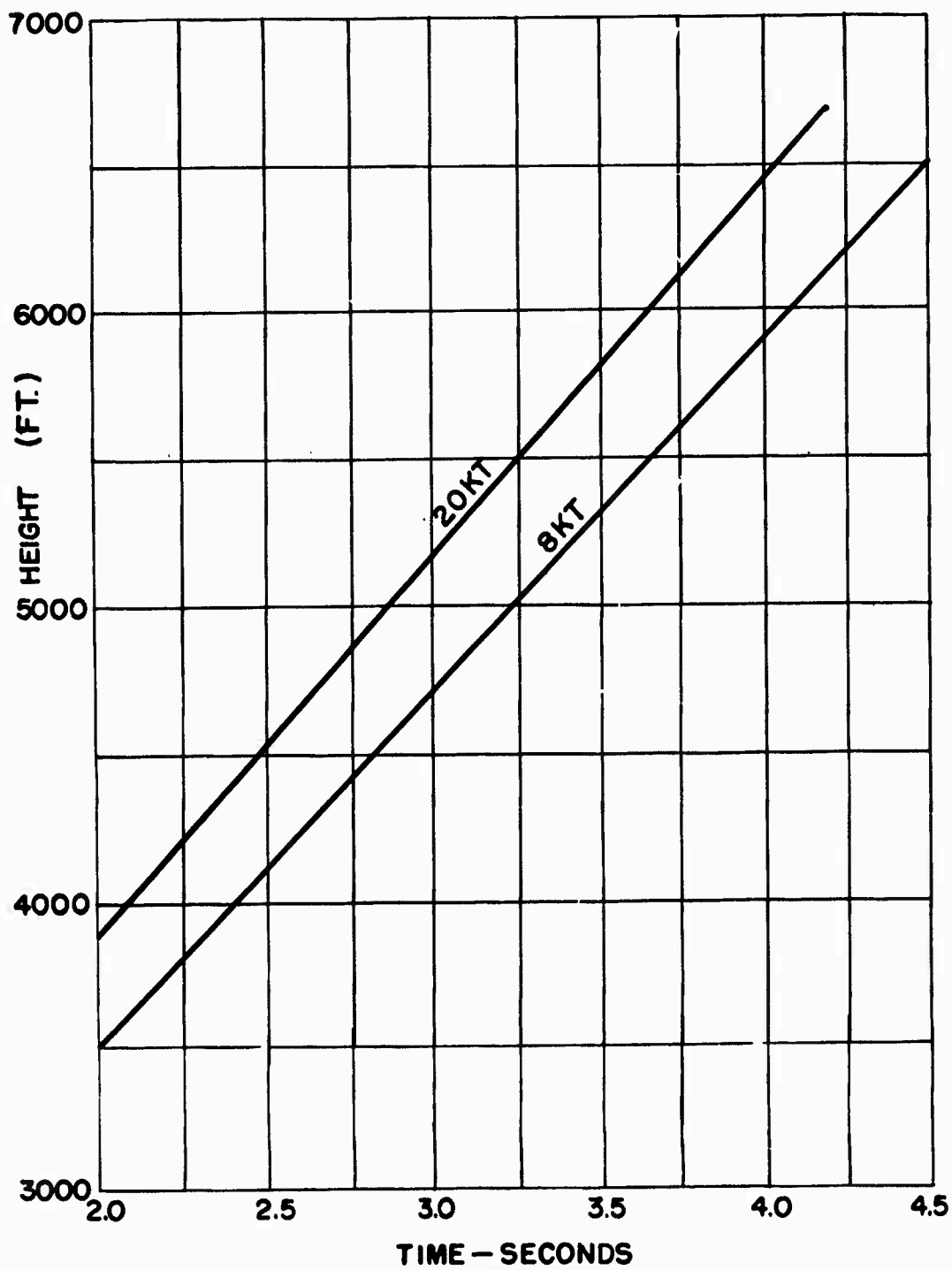
Fig. 3.2 Height of Burst vs Shock Wave Travel Time
