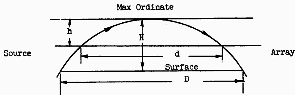
Fig. 2.6 Parabolic Sound Trajectory
