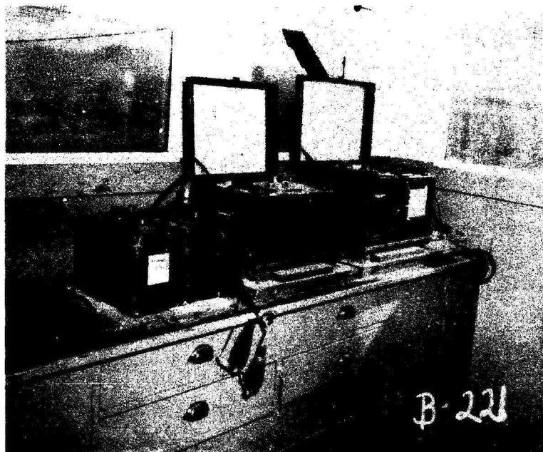
Fig. 4.3 Interior View of Van showing Sound Ranging Set GR-8 which was used for Sound and Seismic experiments.
