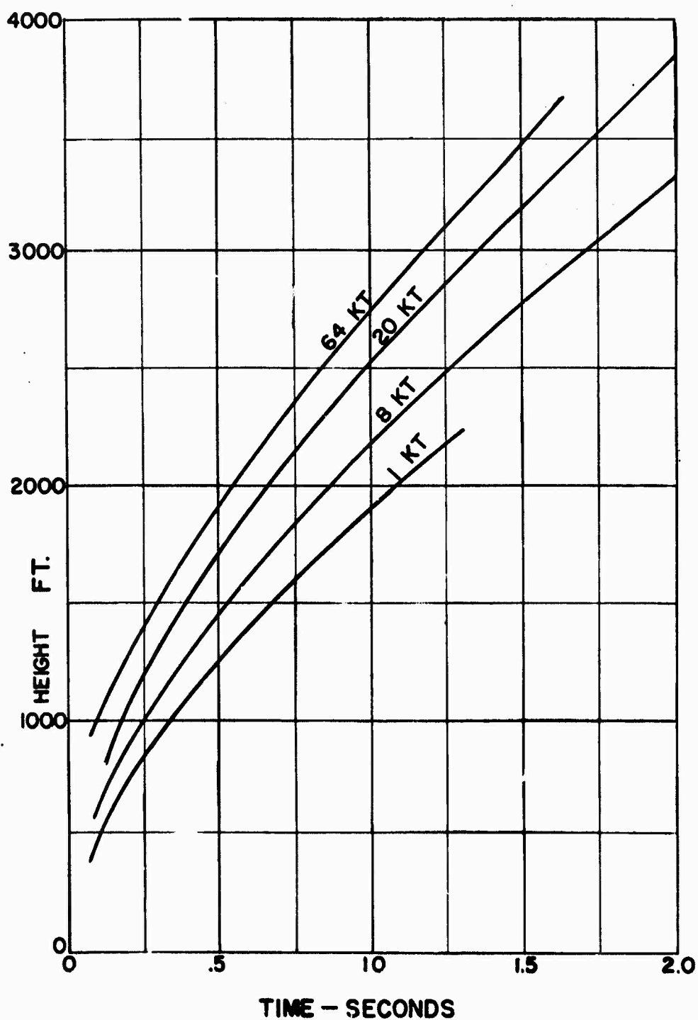
Fig. 3.1 Height of Burst vs Shock Wave Travel Time
