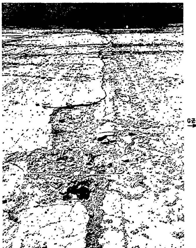
Fig. 4.2 Peeling from Construction Joint
