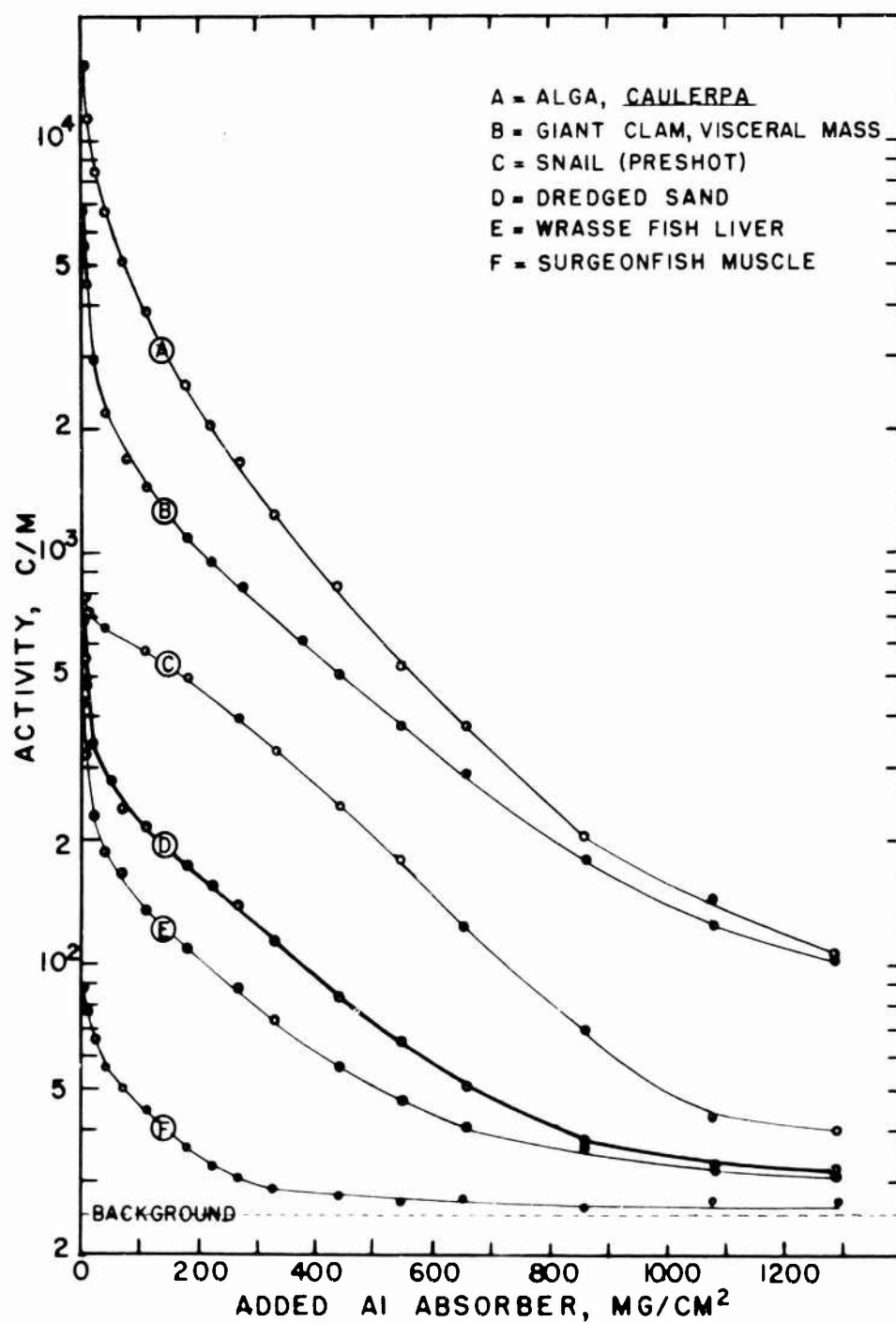
Fig. 3.3—Mass-absorption curves.
