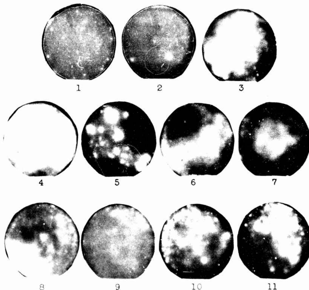
Fig. 4.15—Actual-size autoradiographs of eleven of the more radioactive posttest ashed samples. Pictures should not be compared because of different photographic treatment. (1) Plate 423, Bogallua, damselfish muscle. (2) Plate 407, Bogallua, Tridacna (clam) muscle. (3) Plate 403, Bogallua, octopus digestive gland. (4) Plate 427, Bogallua, damselfish viscera. (5) Plate 353, Bogallua, plankton. (6) Plate 354, Bogallua, plankton. (7) Plate 483, Engebi, hermit-crab viscera. (8) Plate 500, Engebi, H. atra (sea-cucumber) gut and contents. (9) Plate 676, Aaraanbiru, tattler (bird) gizzard. (10) Plate 816, Aaraanbiru, Lyngbya (alga), entire. (11) Plate 819, Aaraanbiru, Jania -like alga, entire.
