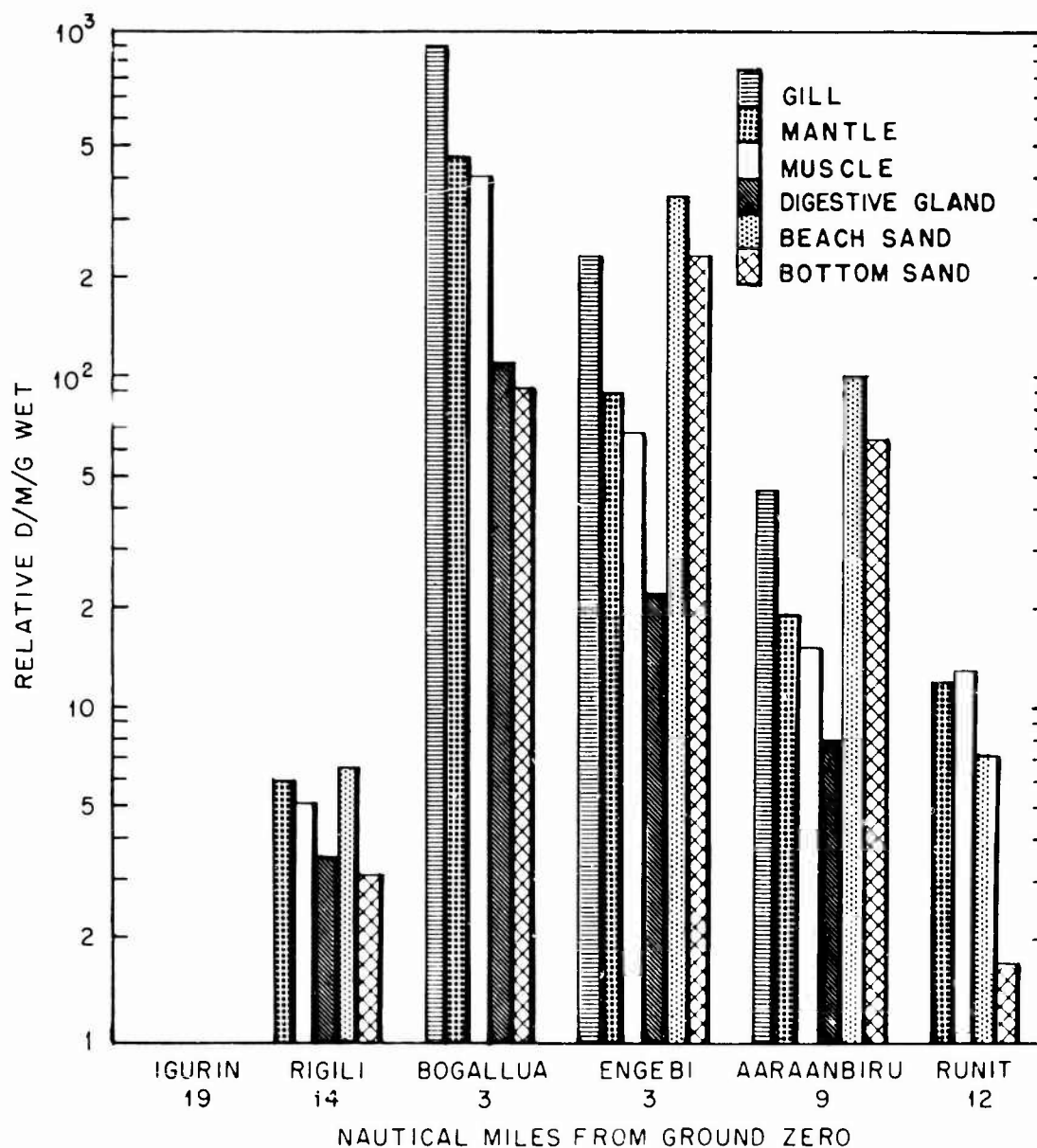
Fig. 4.1 — Relative radioactivity of soil or beach sand, Bottom sand taken from sea-cucumber guts and giant-clam gill, mantle, muscle, and digestive gland. The relative activity of each type of sample at Iguirin is taken as 1.
