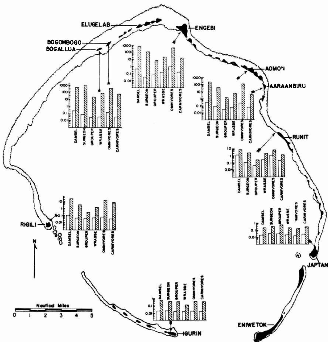
Fig. 4.4—Histograms showing radioactivity of various species of fish. Omnivores and carnivores and all omnivores and carnivores combined are represented. Open histograms, preshot, Shaded histograms, postshot.
