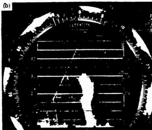
Figure 3.3 RHI presentations, Eniwetok, Shot Butternut. Range markers, 5-mile intervals; height values, thousand-foot levels; target, 15 miles. Photo (a) was taken at H + 7 minutes; photo (b) was taken at H + 9 minutes.
