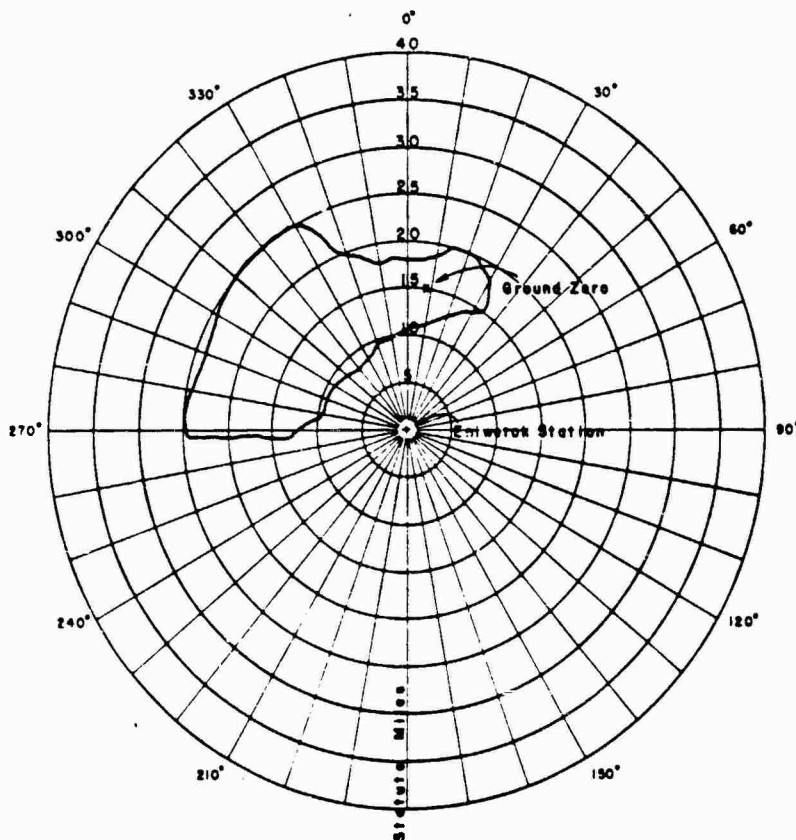
Figure 3.13 Area covered by Shot Cactus cloud during time of radar detectability.
