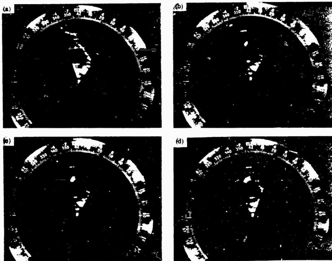
Figure 3.2 PPI presentations, Eniwetok, Shot Butternut. Range markers, 5-mile intervals; target, 15 miles and 354-degree azimuth. Photos (a) through (d) were taken at H + 5, 6, 7, and 9 minutes, respectively.
