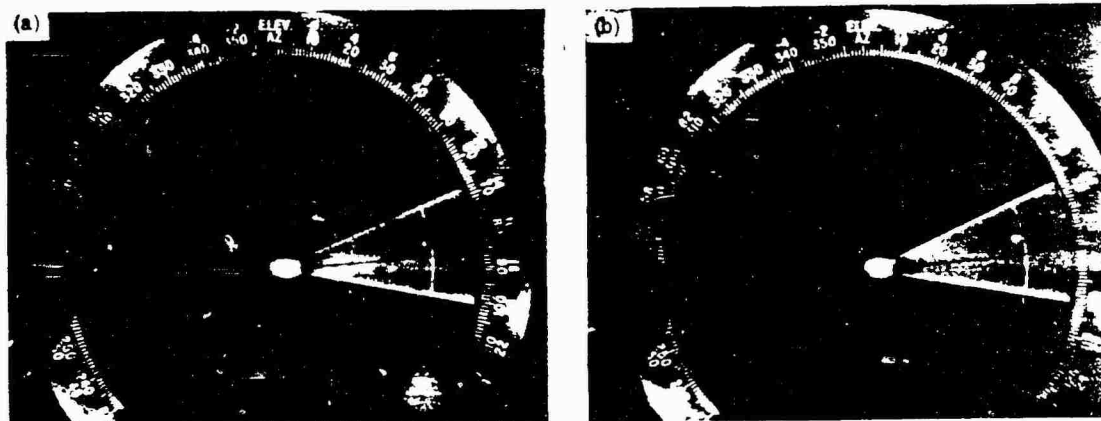
Figure 3.1 PPI presentations, Eniwetok, Shot Fir (detonated at Bikini). Range marker, 210 miles; target, 201 miles and 81-degree azimuth. Photo (a) was taken at H + 6 minutes, 25 seconds; photo (b) was taken at H + 11 minutes, 55 seconds.
