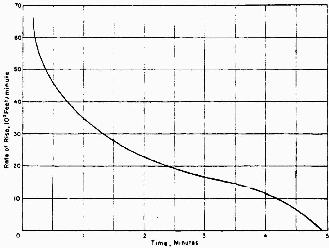
Figure 3.5 Rate of rise versus time, Shot Koa.
