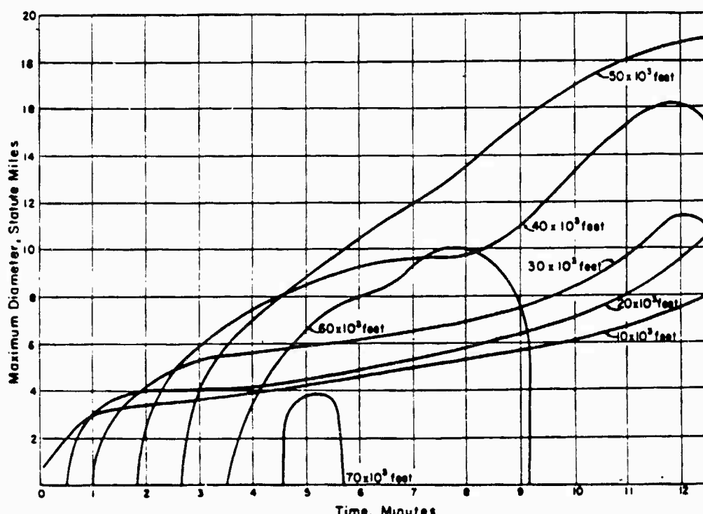
Figure 3.7 Maximum diameter at constant heights versus time, Shot Koa.
