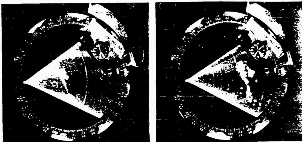
Figure 3.14 Cloud cover to the east of Johnston Island prior to zero time, Shot Orange
