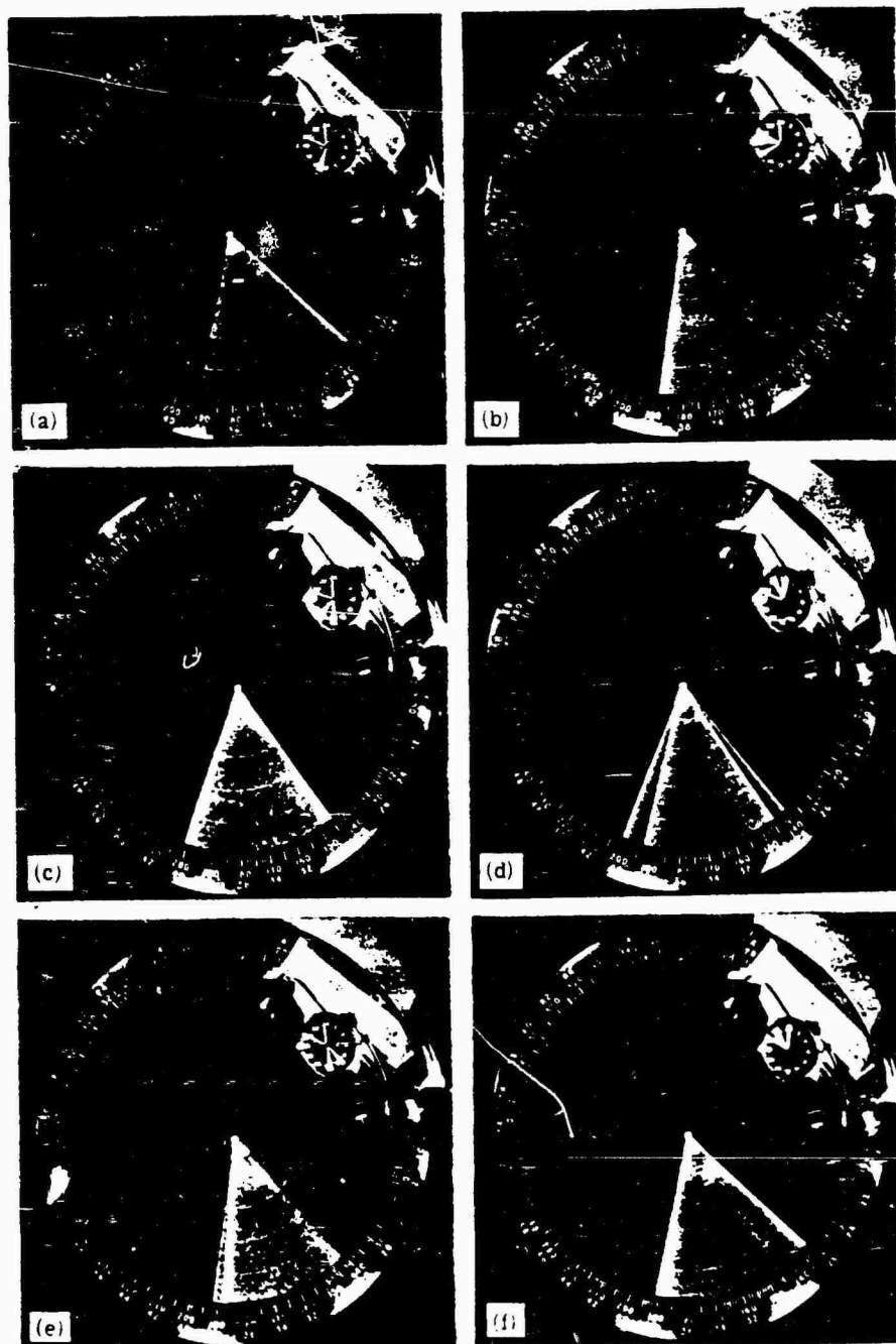
Figure 3.16 PPI presentations of unidentified radar echoes received during Shot Orange.
