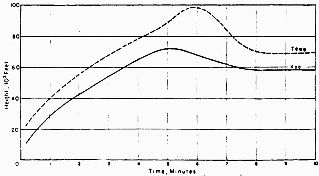
Figure 3.6 Comparison of stabilized height versus time, Shots Koa and Tewa.
