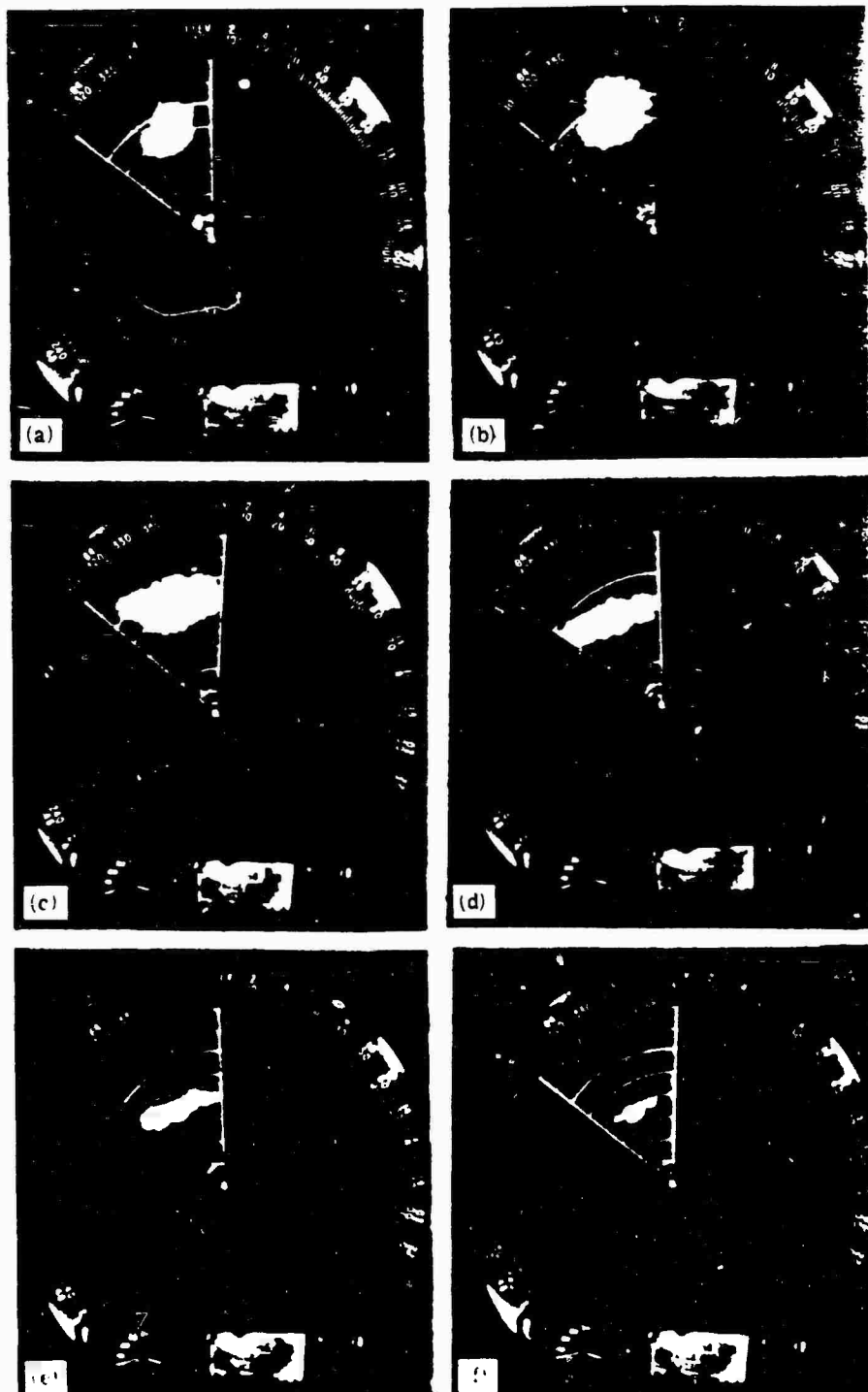
Figure 3.8 PPI presentations, Eniwetok, Shot Koa. Range markers are at 5-mile intervals. Photos (a) through (c) were recorded at angles of 10 to 20 degrees in 5-degree steps, and (d) through (f) at 25 to 35 degrees in 5-degree steps.
