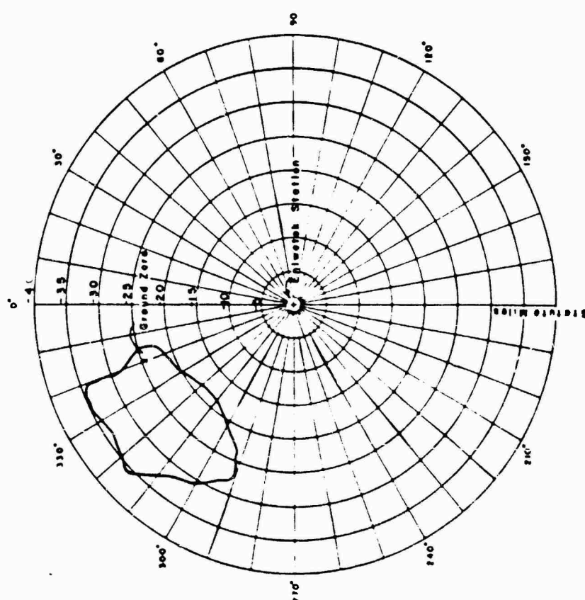
Figure 3.11 Area covered by Shot Yellowwood cloud during time of radar detectability.
