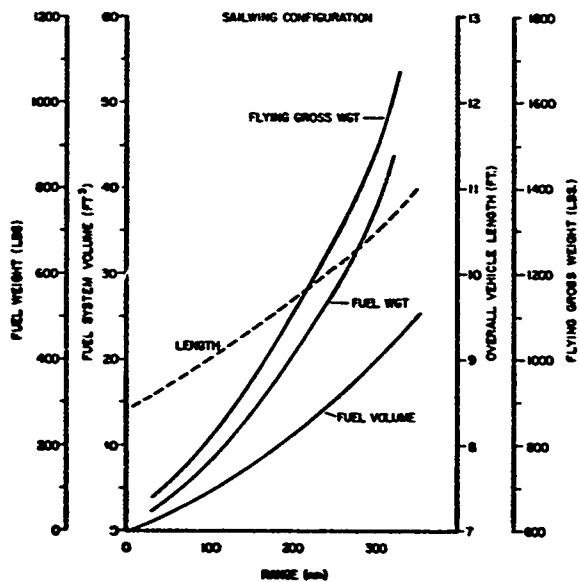
Figure 20. Sailing Parameters
