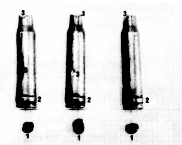
Figure 1.4-2: Cartridge Case Casualties of the 5.56 x 45-MM Cases Fired in an HK-23A1 Machine Gun with Fluted Chamber. No. 1: Blown Primers. No. 2: Radially Bulged Case Heads. Case Neck and Body Indentations (No. 3) Are Ejection Marks. The Longitudinal Striations on the Case Neck Are Chamber Flute Marks.
