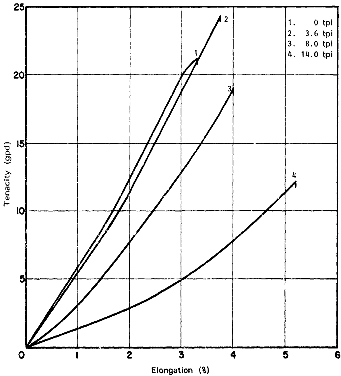
Figure 20. Typical Stress-Strain Diagrams of Kevlar 29 Twisted Yarn
