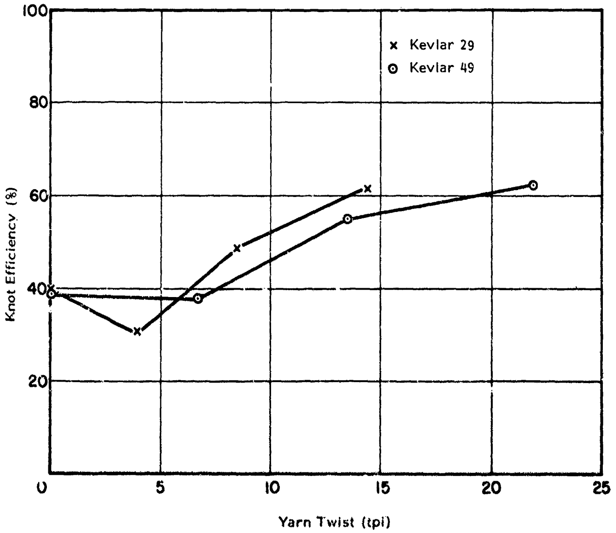
Figure 28. Knot Efficiency of Twisted Kevlar Yarns
