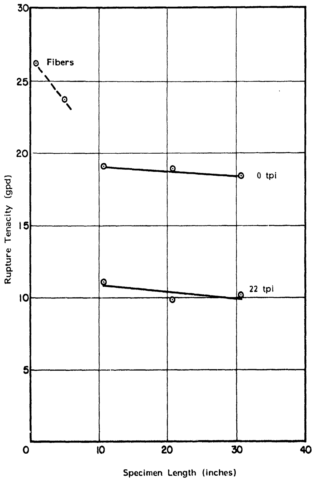
Figure 24. Effect of Specimen Length on Rupture Tenacity of Kevlar 49 Yarn
