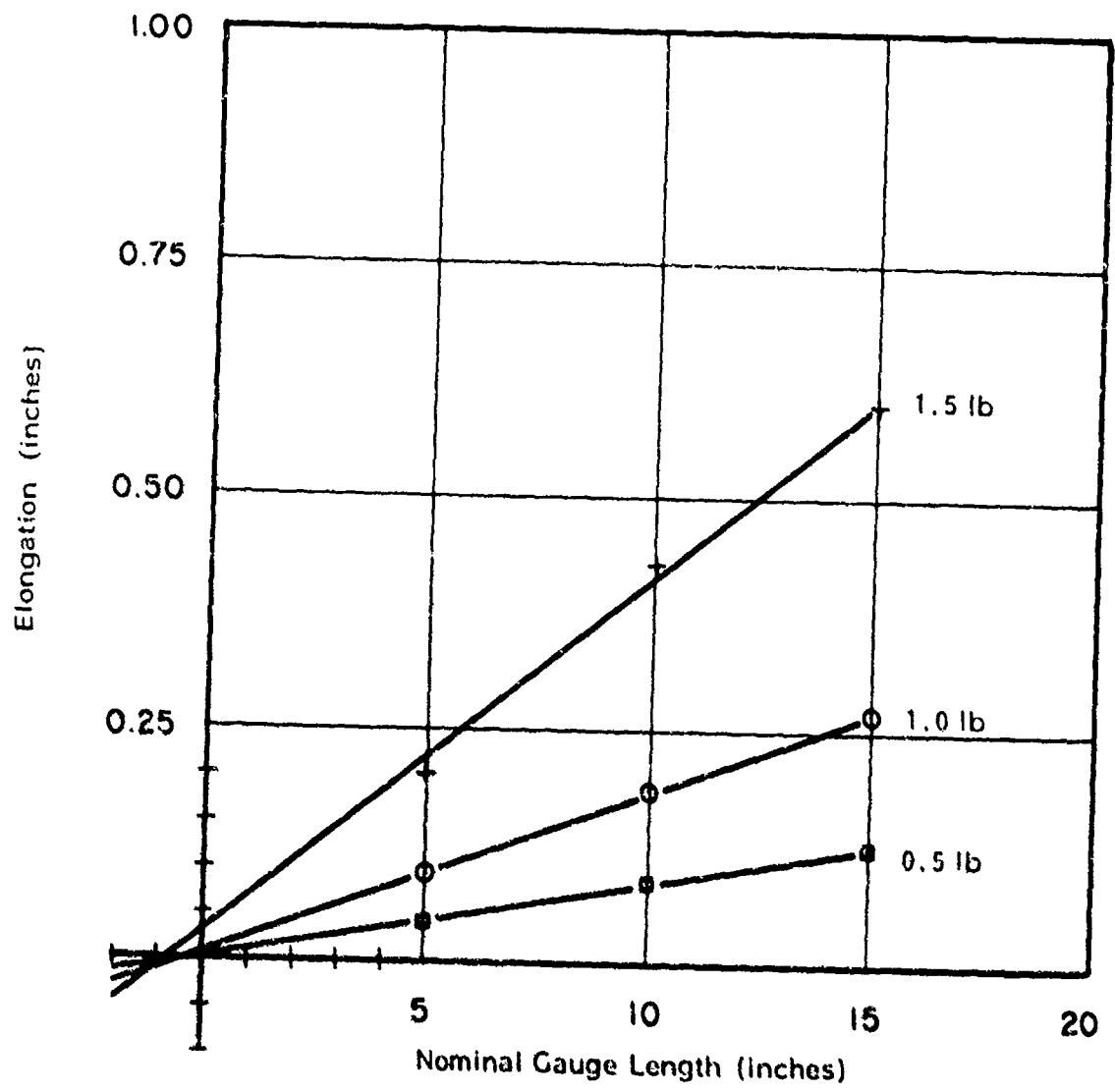
Figure 4. Gauge Length Correction for PBI Yarn
