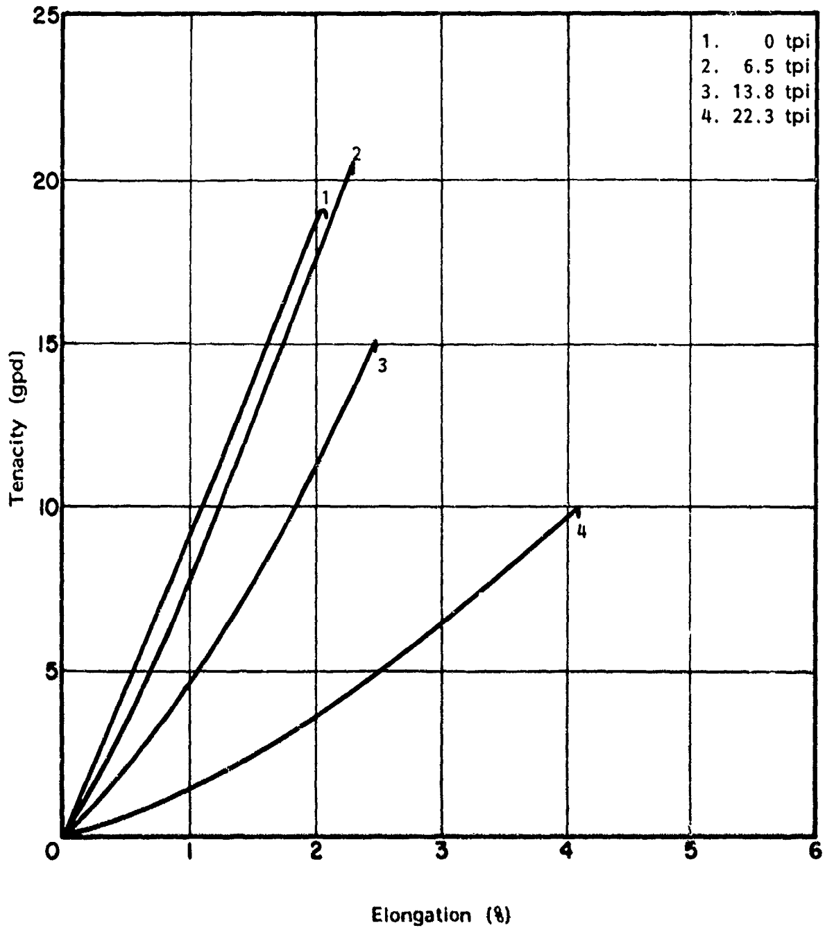
Figure 21. Typical Stress-Strain Diagrams of Kevlar 49 Twisted Yarn
