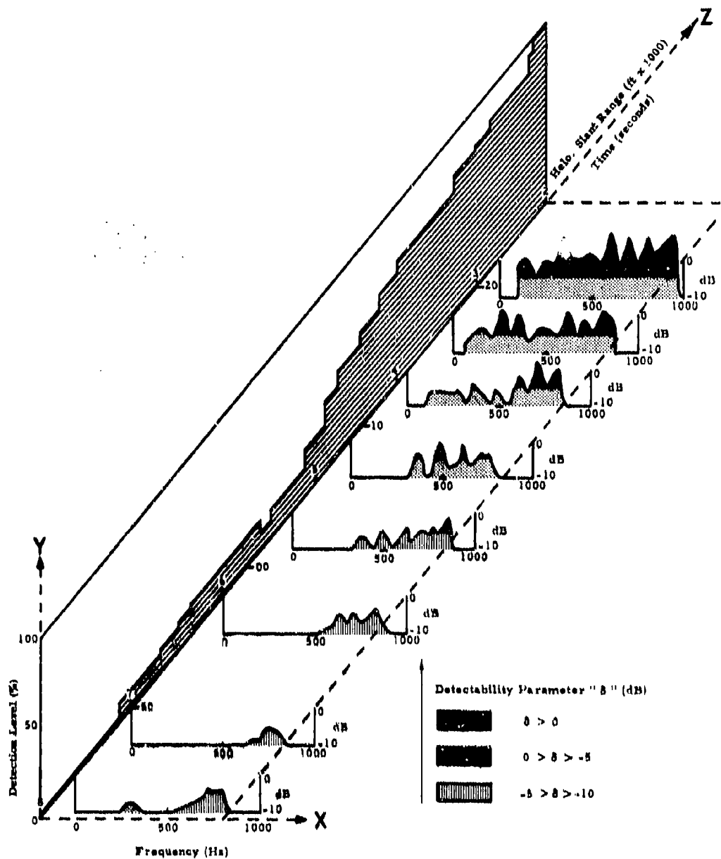
Figure 44. Summary of Measured Detection Data for Run 46 (2-Second Average).
