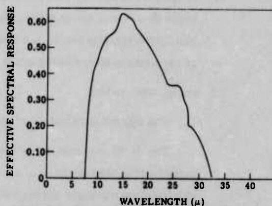
(d) Channel 4. Does not include constant value over 7- to 35-μ region of RRS-5 lens.
