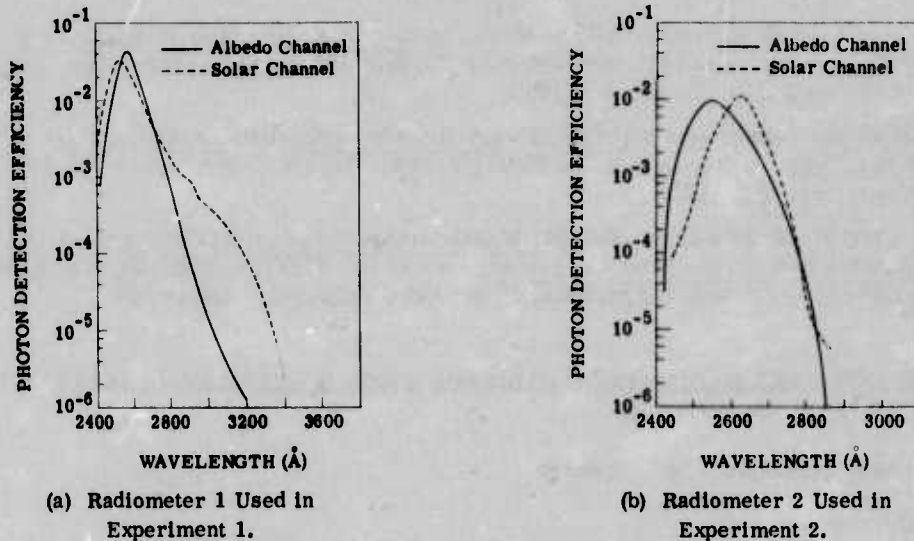
FIGURE 14. SPECTRAL RESPONSES OF AEROSPACE ULTRAVIOLET RADIOMETERS Unclassified
