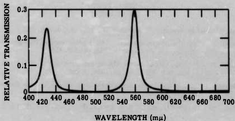
FIGURE 42. TRANSMISSION CURVES FOR INTERFERENCE FILTERS USED IN EARLY PHOTOELECTRIC MEASUREMENTS OF SKY BRIGHTNESS. Miley, 1953.
