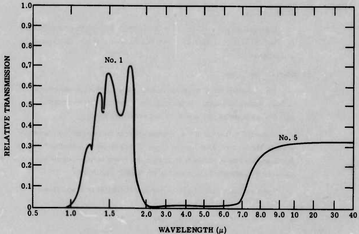
FIGURE 32. TRANSMISSION CURVES FOR INFRARED FILTERS 1 AND 5 OF THE RADIOMETER FILTER WHEEL USED IN STUDYING THE HORIZON AT 15 \mu AND THE THERMAL REGION Unclassified
