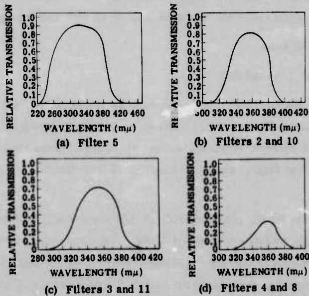
FIGURE 7. INDIVIDUAL TRANSMISSION CURVES FOR FILTERS IN THE FILTER WHEEL OF THE ULTRAVIOLET RADIOMETER. D. G. Murcra, 1959. Unclassified
