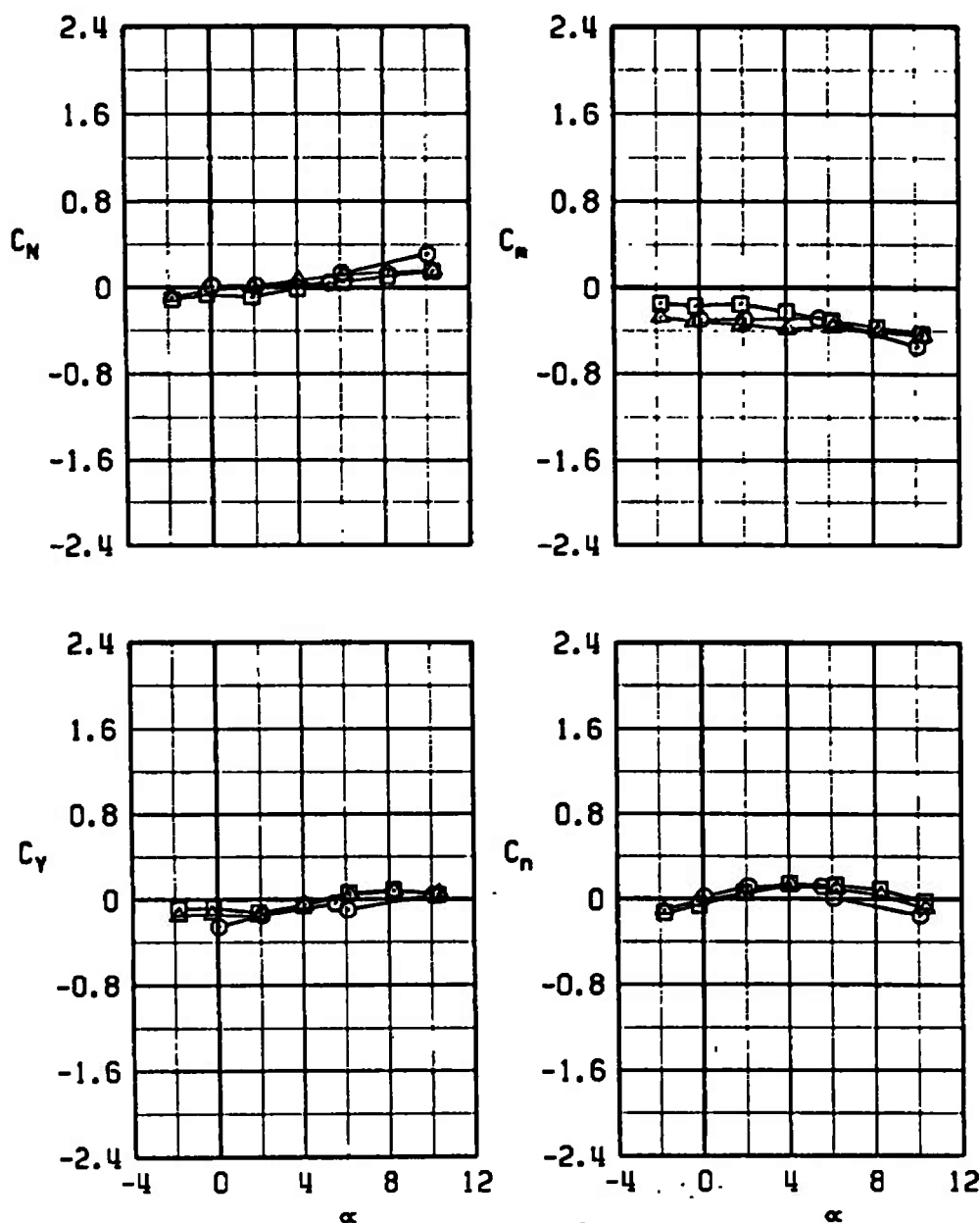
b. M_\infty = 0.90 Figure 38. Continued.
