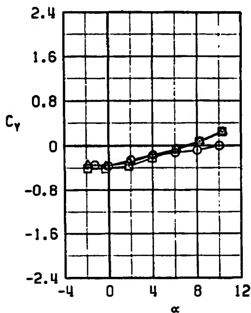
b. M_\infty = 0.90 Figure 41. Continued.
