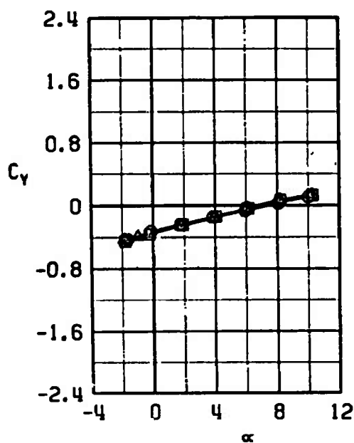
c. M_\infty = 1.05 Figure 42. Concluded.
