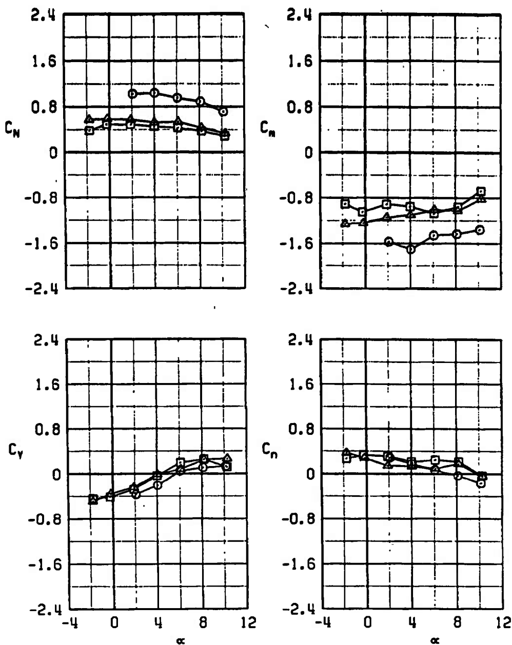
c. M_\infty = 1.05 Figure 38. Concluded.
