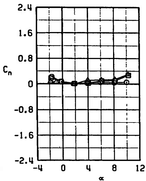
c. M_\infty = 1.05 Figure 42. Concluded.
