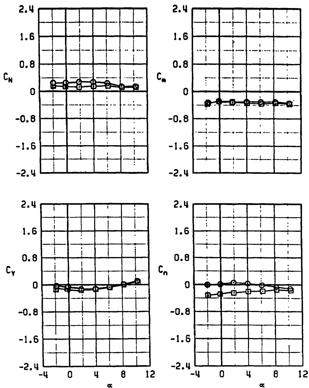
Figure 22. Comparison of basic M-117 carriage-position aerodynamic coefficients with and without the presence of the 0.2-in.-diam dummy sting, configuration 1R.
