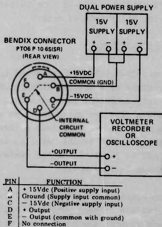
FIGURE 32. POWER/OUTPUT SCHEMATIC
