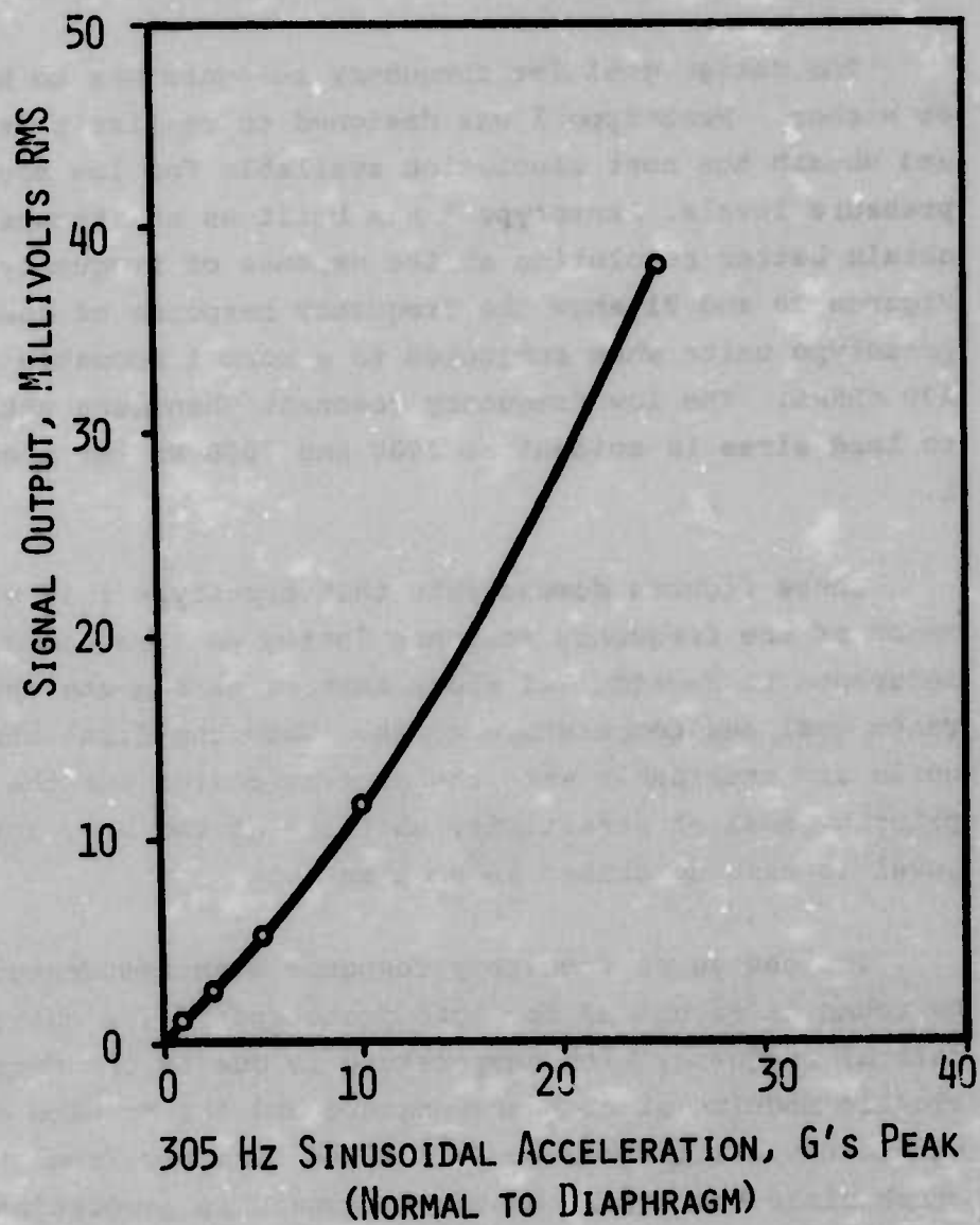
FIGURE 19. ACCELERATION RESPONSE OF PROTOTYPE NO. 2
