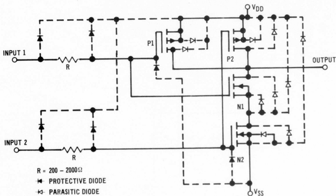
FIGURE 3 4011 CIRCUIT DIAGRAM SHOWING ALL PN JUNCTIONS (Parasitic and Protective Junctions Indicated by Dashed Lines)
