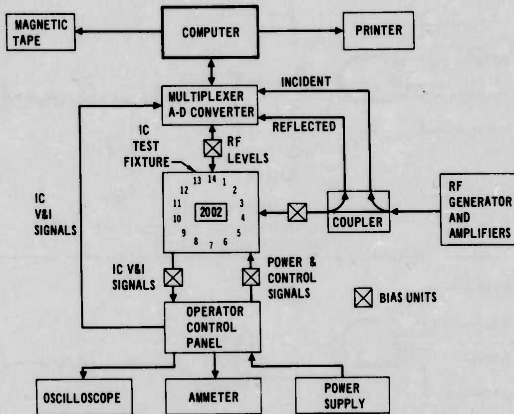
FIGURE 16 SCHEMATIC DIAGRAM FOR 2002 AUTOMATED MEASUREMENT SYSTEM
