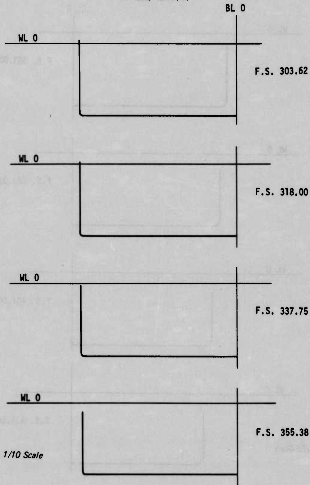
Figure 39: Cross Sections — Conformal Carriage Gun Installation (continued)
