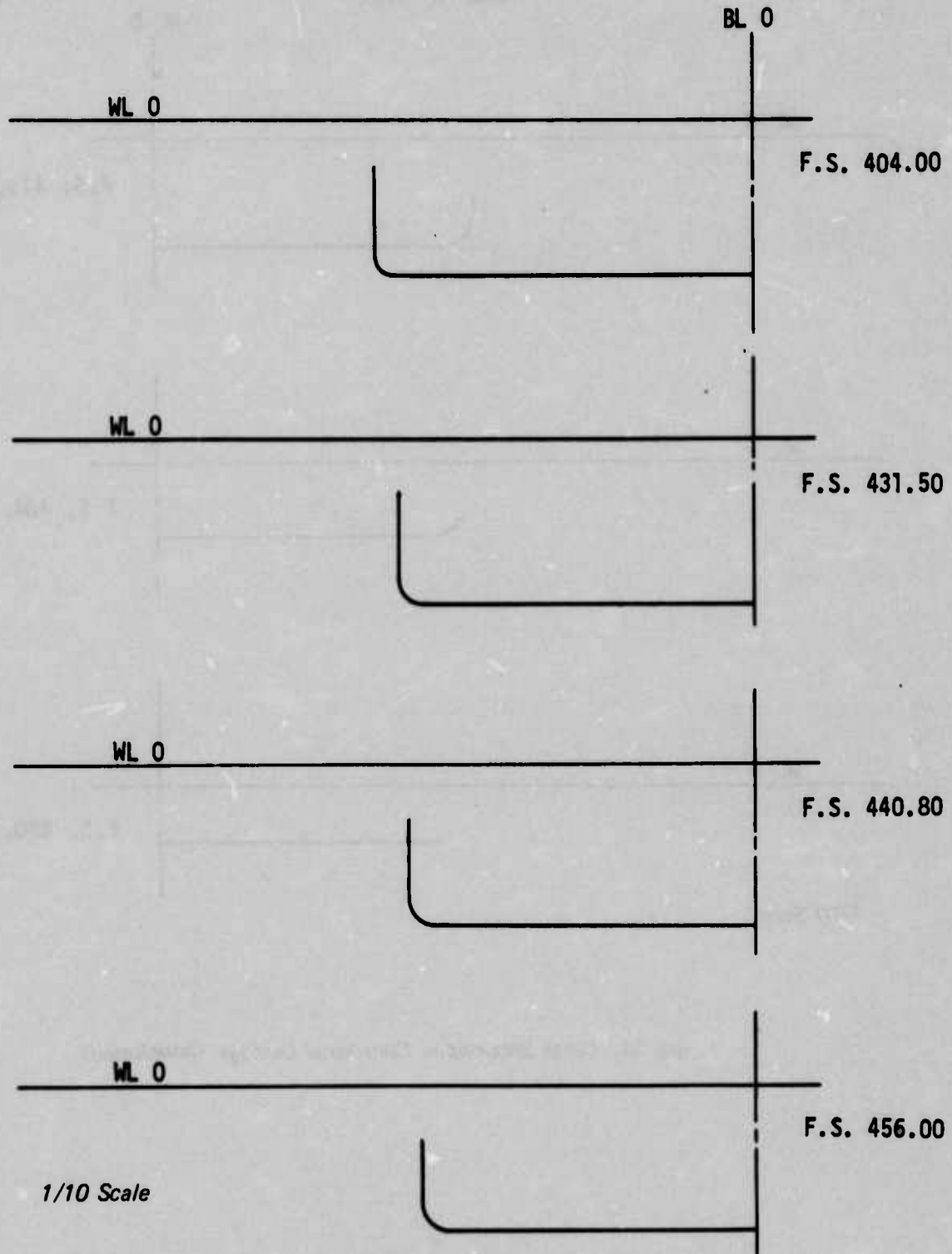
Figure 40: Cross Sections — Ccnformal Carriage (continued)
