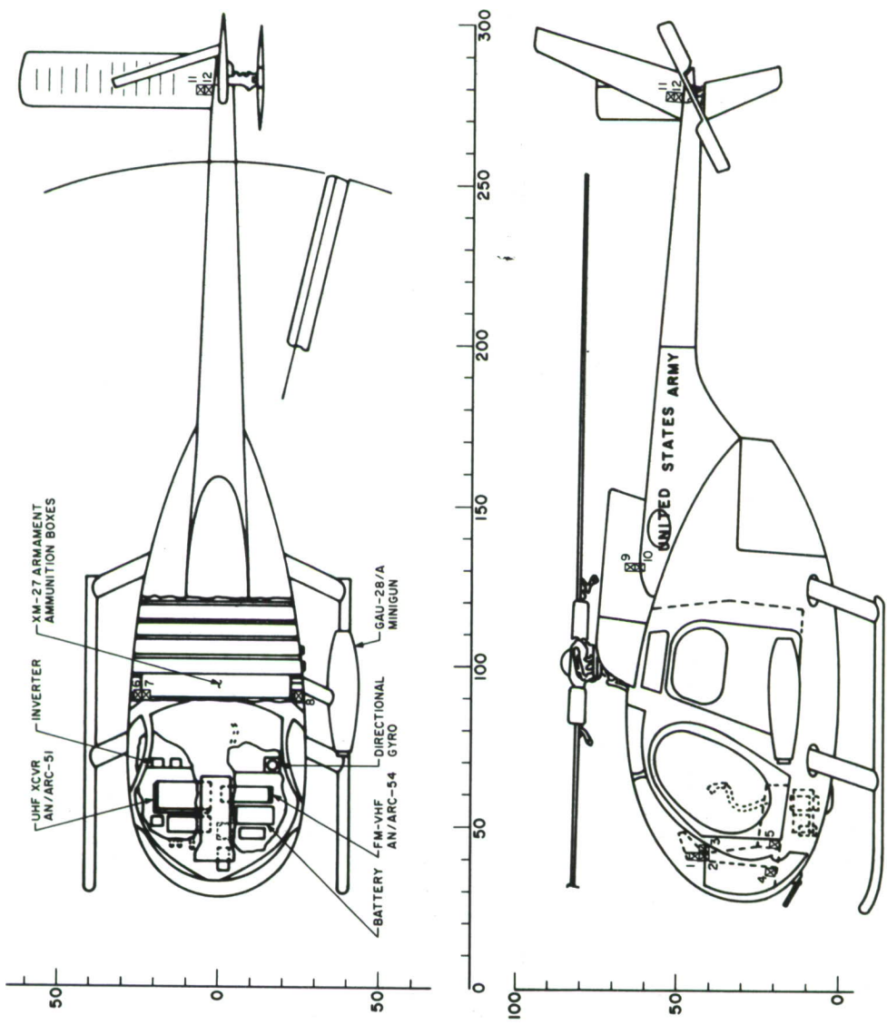
Figure 5. Low Frequency Accelerometer Locations
