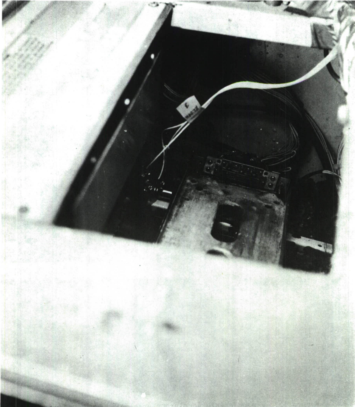
Figure 11. Piezoelectric Accelerometers, Left Side, AN/ARC-54, Sta. 58, PUID's 20, 21, 22
