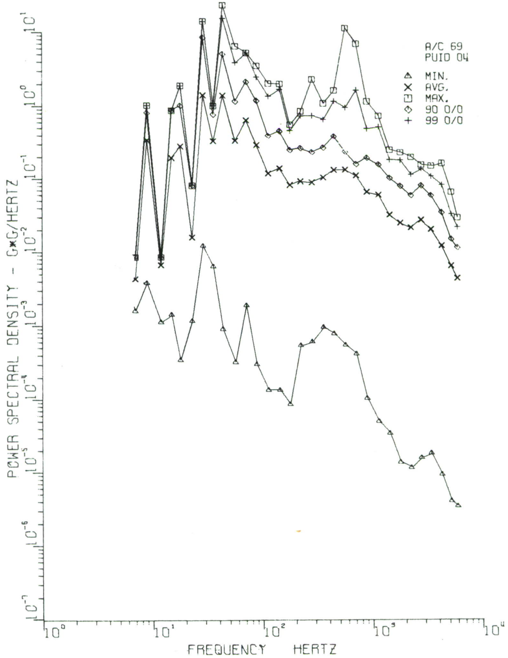
Figure 153. Nose Section and Cockpit, with Gunfire
