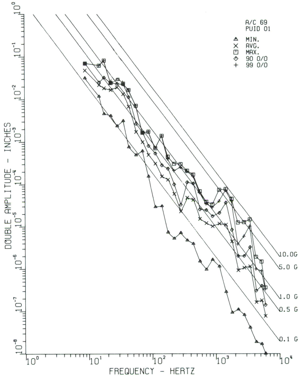
Figure 42. Vertical, Lateral, and Fore and Aft, Main Rotor Transmission Interface, Right Rear Support, Sta. 108, without Gunfire
