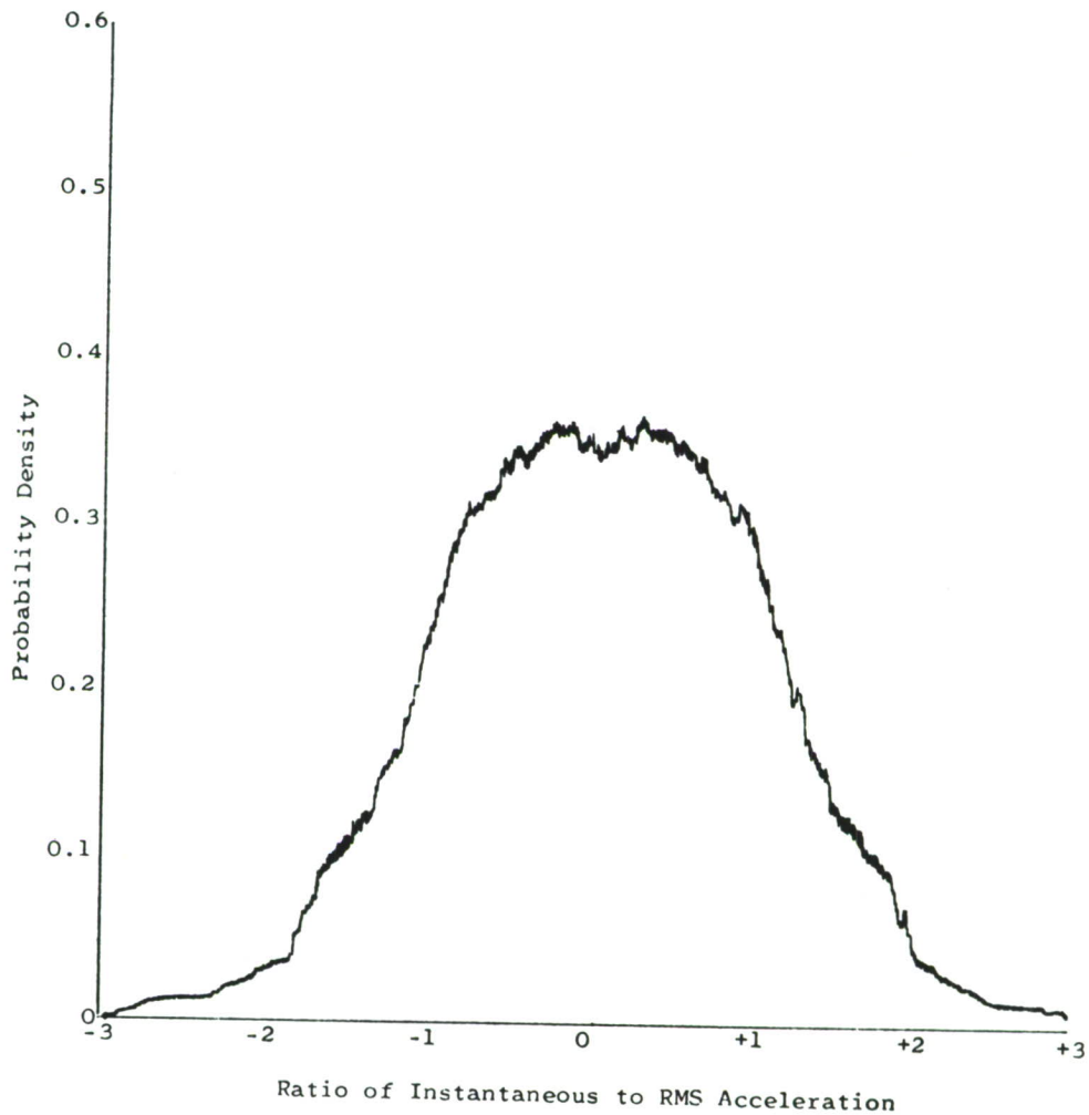
Figure 175. Acceleration APD in Electronics Compartment during Gunfire, Vertical, 700 Hz Band
