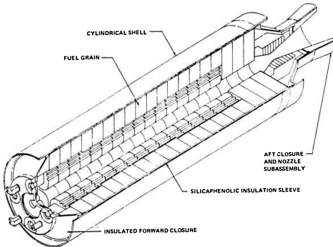
Figure 83. HAST Motor Case
