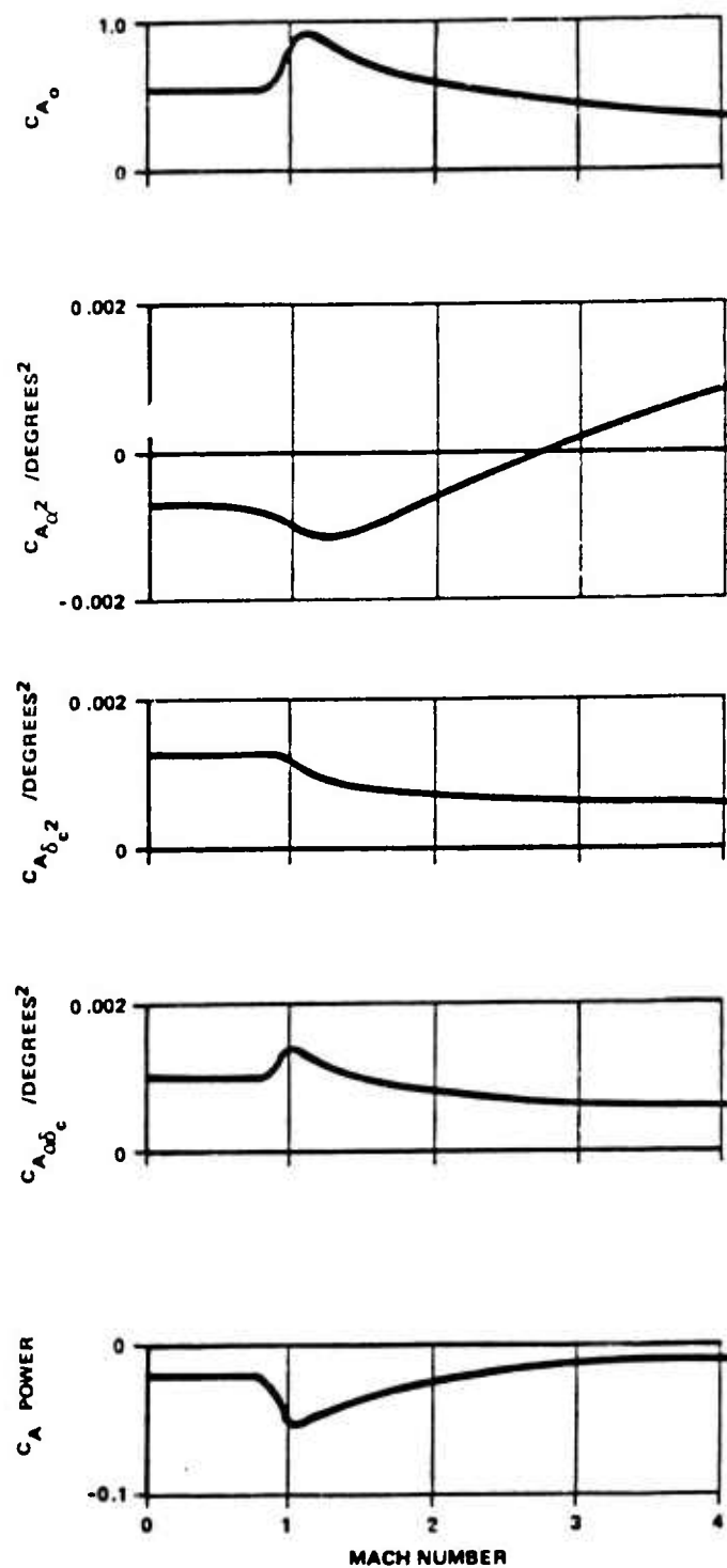
Figure 10. HAST Axial Force Coefficient
