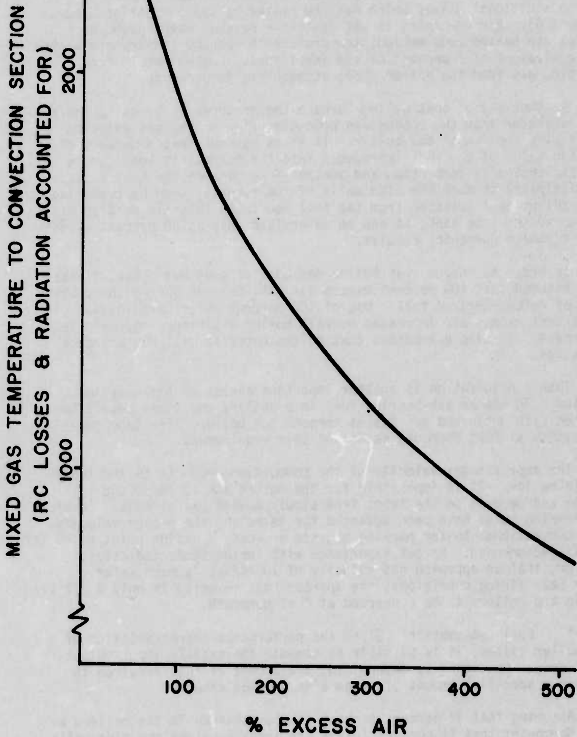
Figure 6. Furnace gas temperatures ( ^{\circ}\text{F} ) as a function of excess air.
