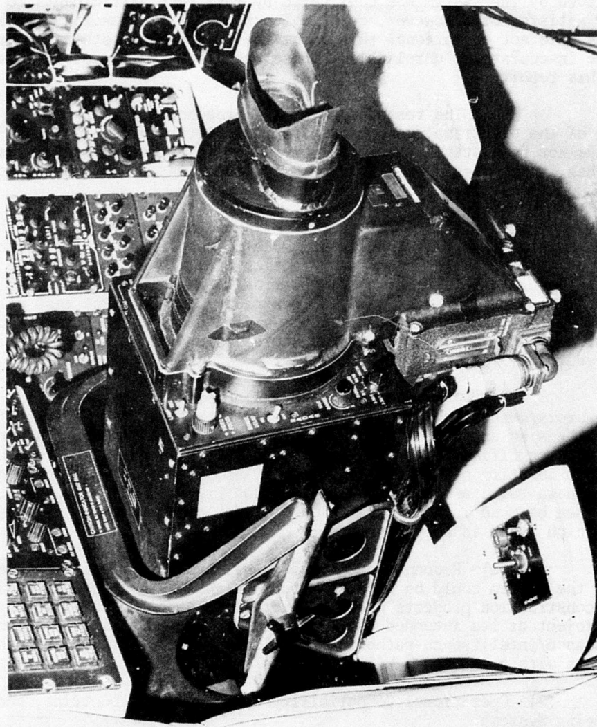
Figure 1. Radar Indicator and Camera/Periscope Assembly.
