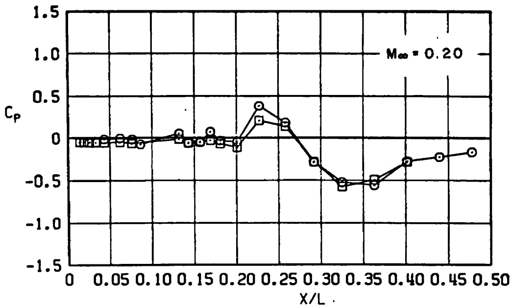
Figure 22. Variation of pressure coefficient along the two side rows of the radome-bomb body at -0.5 -deg beta angle.
