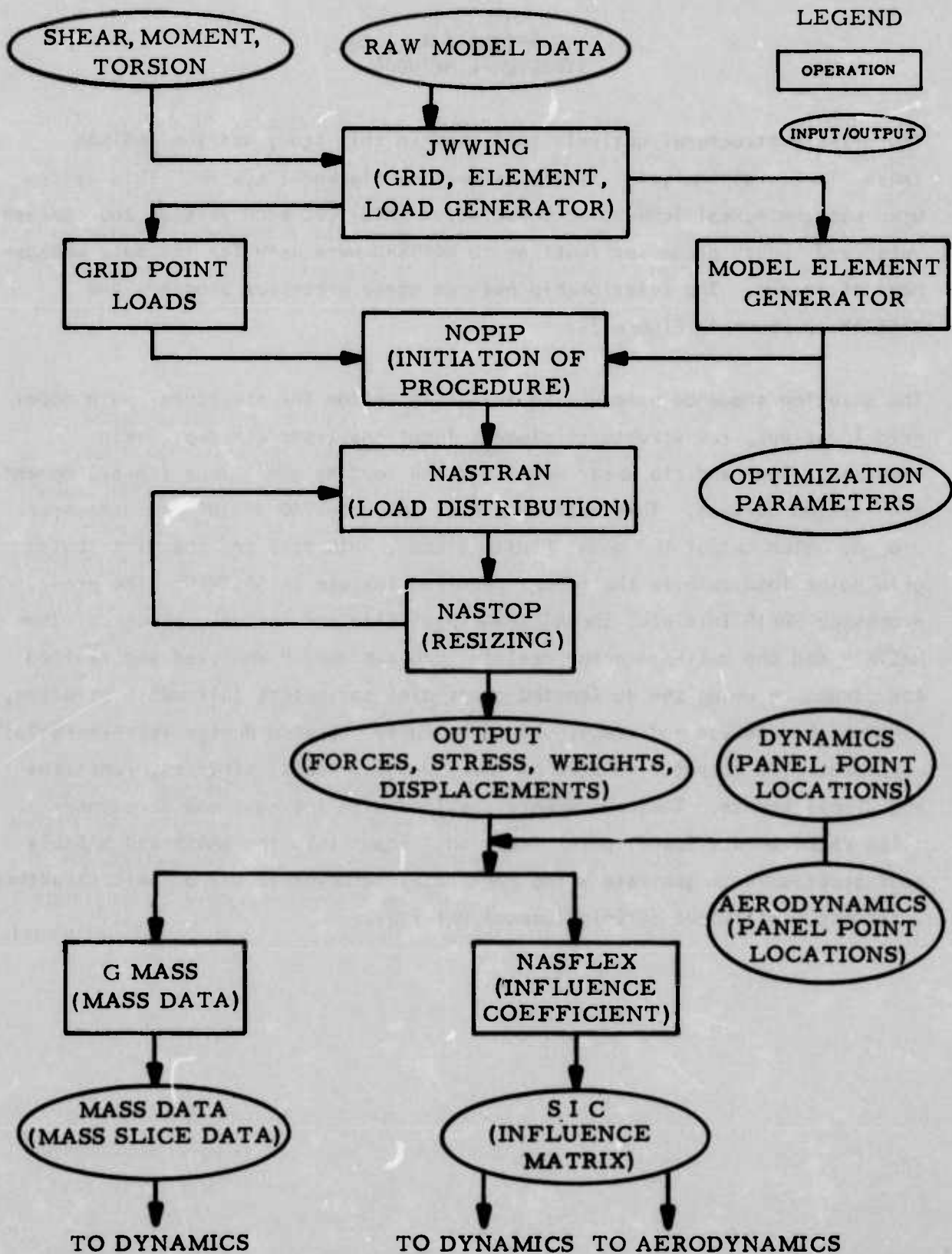
FIGURE 32: FLOW DIAGRAM FOR STRUCTURAL METHODS EMPLOYED IN CCS ANALYSIS
