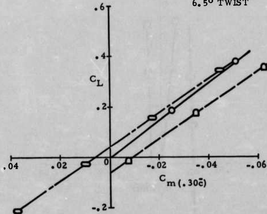
FIGURE 48: EFFECT OF COMBINED CAMBER AND TWIST ON LIFT AND PITCHING MOMENT M = 1.20
