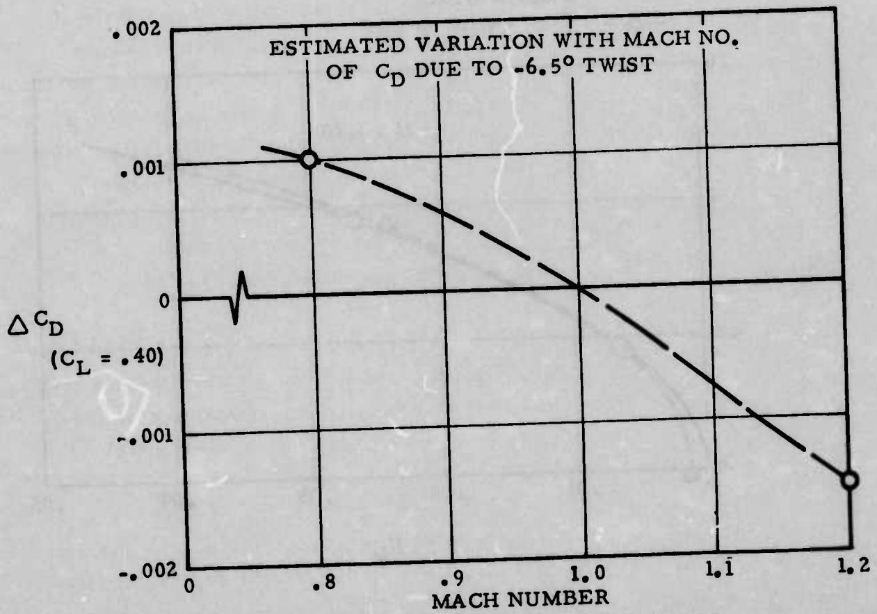
FIGURE 39: EFFECT OF TWIST ON DRAG VALUES
