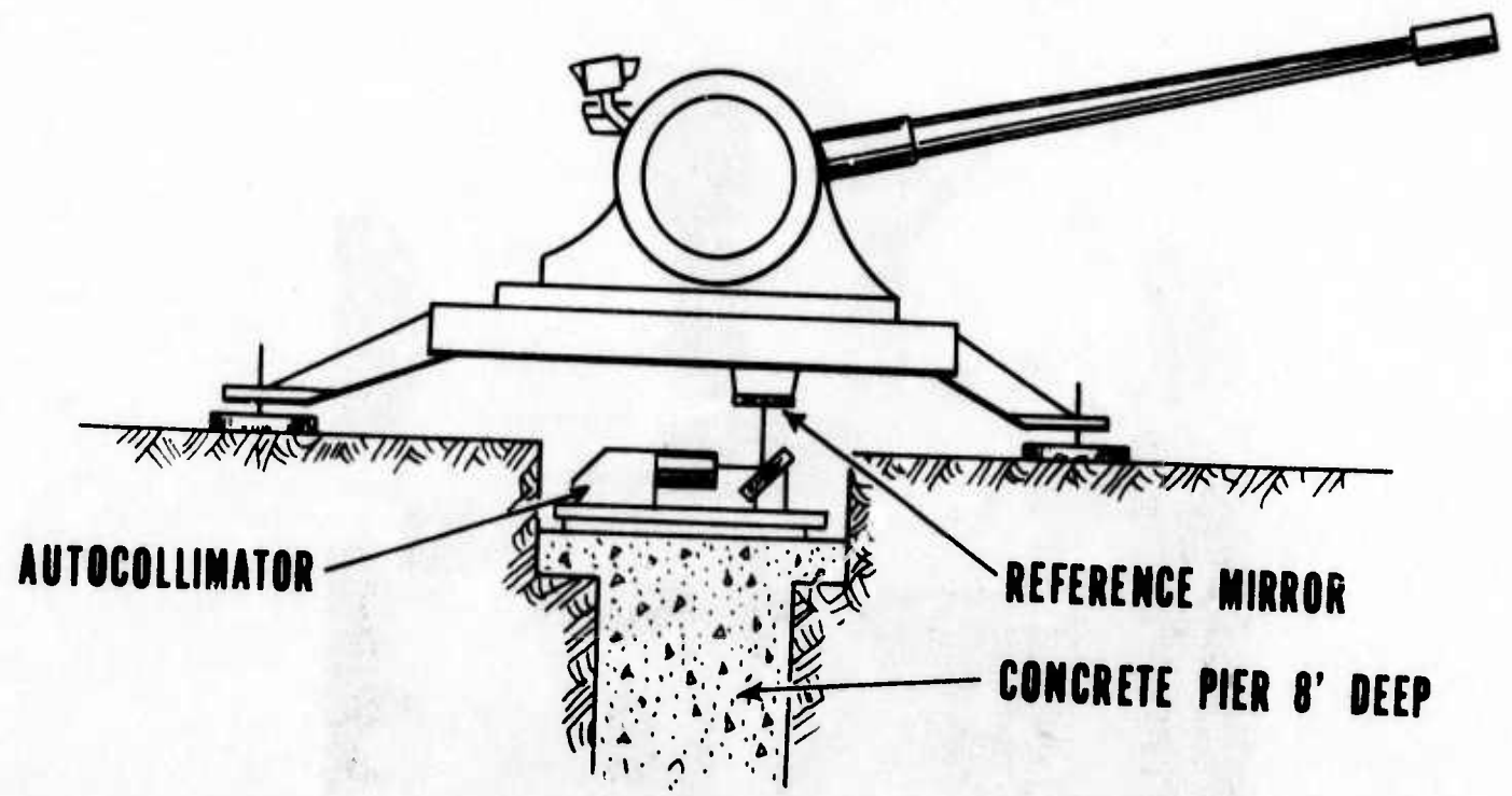
Figure 1-4. Drawing of Tilt Measurement System
