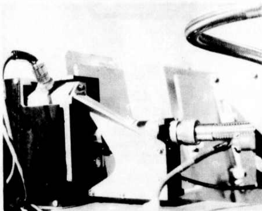
Figure 1-6. LOCAM Mounted on S-60 Gun
