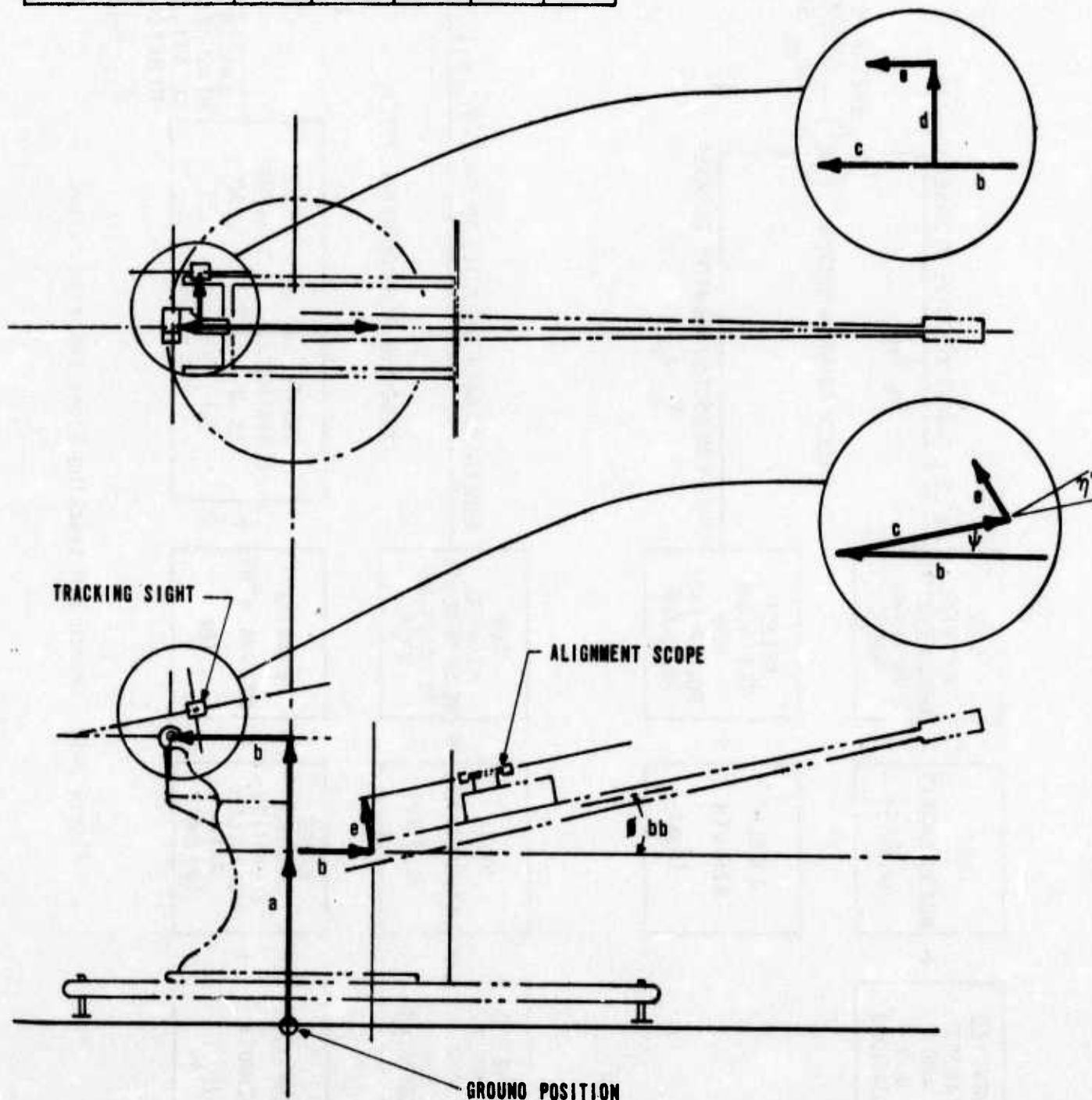
Figure 2-4. Physical Measurements on the S-60 Gun
