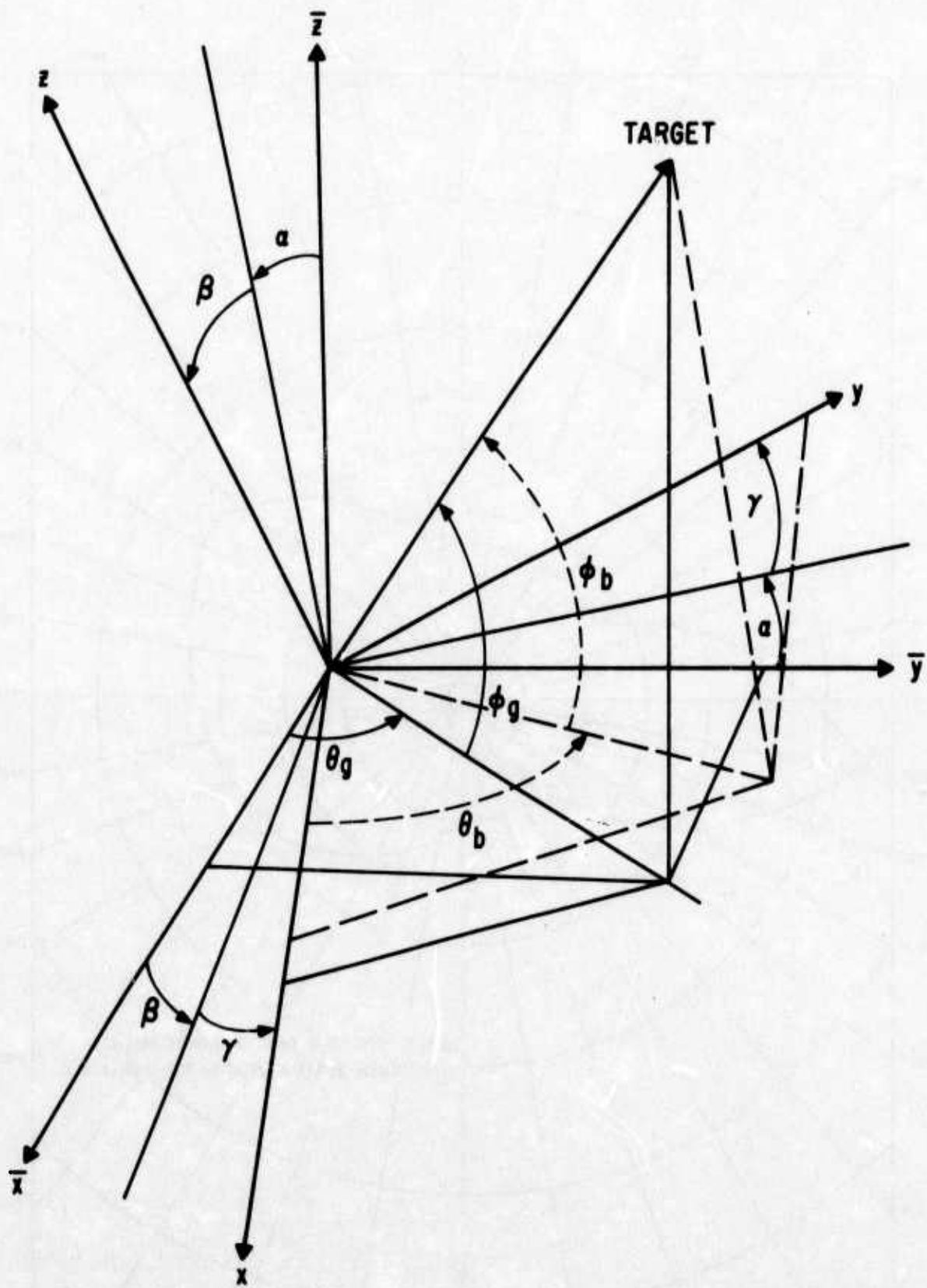
Figure 4-2. Transformation from Tilted to Untilted
