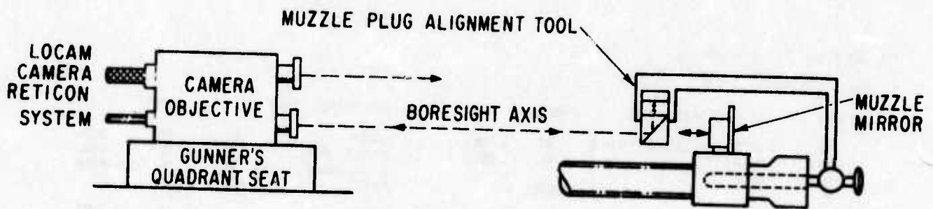
Figure 2-7. Alignment Concept
