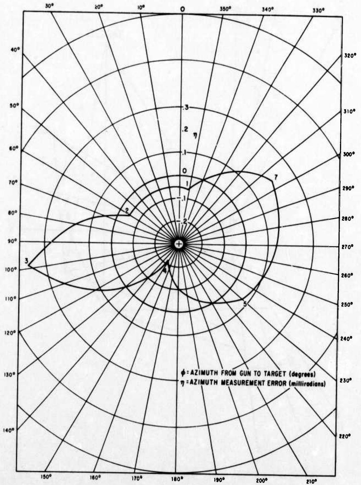
Figure 4-1. Azimuth Measurement Error versus Azimuth
