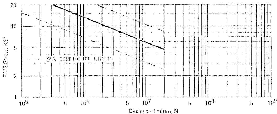
FIGURE 6.6.1-12 S-N DATA FOR 7075-T6 RIB FLANGES - BOX STRUCTURE SONIC FATIGUE TEST SPECIMENS
