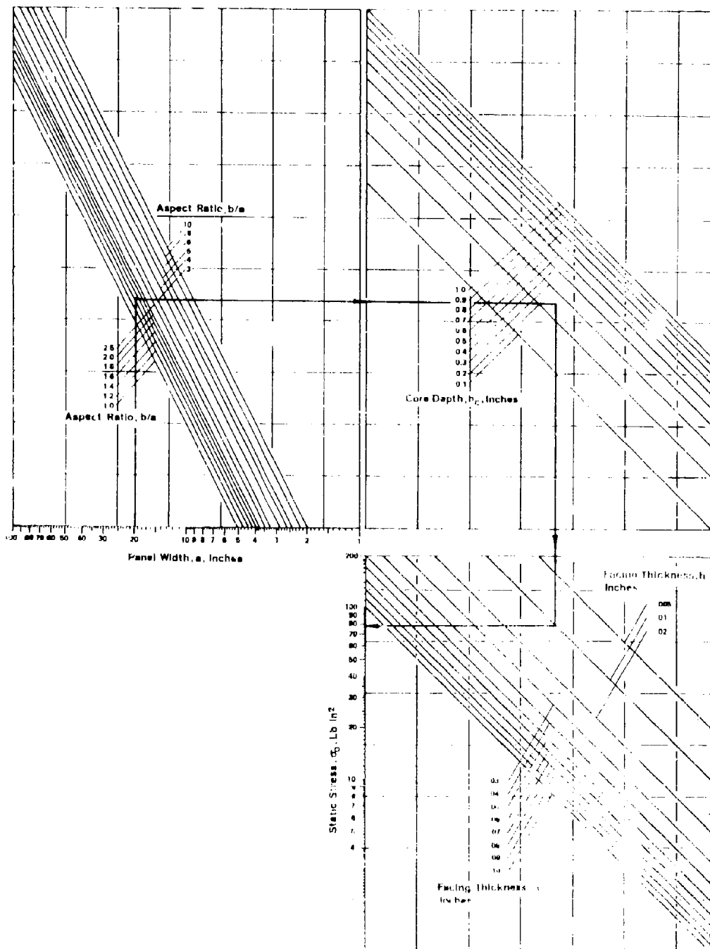
FIG. 3.4-5 STATIC EDGE STRESS RESPONSE DUE TO UNIFORM STATIC PRESSURE FOR DIFFUSION-BONDED TITANIUM HONEYCOMB PANELS (REF. 3)
