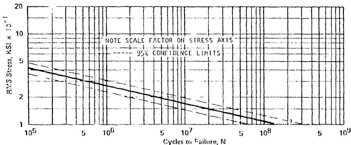
FIGURE 6.6.4-2 COUPON S-N DATA FOR SHARPLY NOTCHED RENE' 41 SHEET - 700^\circ\text{F}
