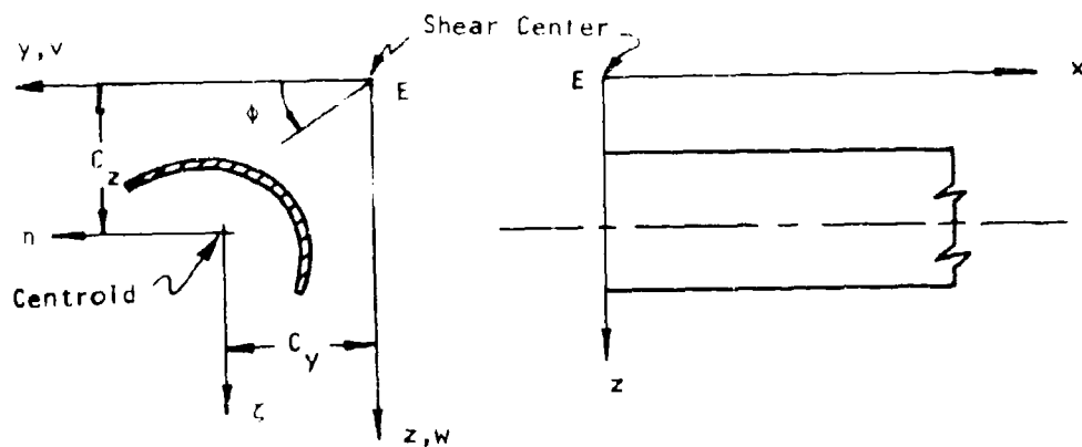
FIGURE B.1.1-5 AXIS SYSTEM, GEOMETRY, AND NOMENCLATURE FOR COUPLED BENDING-TORSION VIBRATION OF THIN-WALLED OPEN SECTION BEAMS
