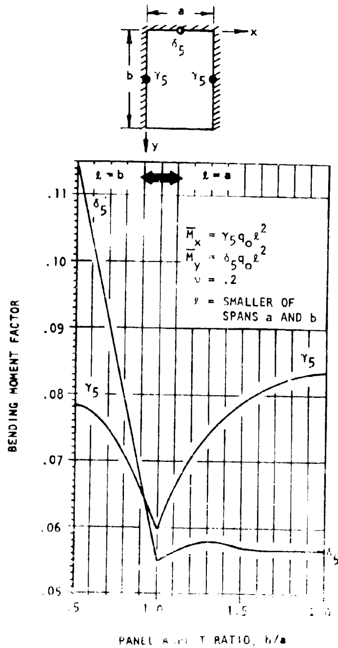
FIGURE 5.3.2-5 BENDING MOMENT FACTOR (PART 4)
