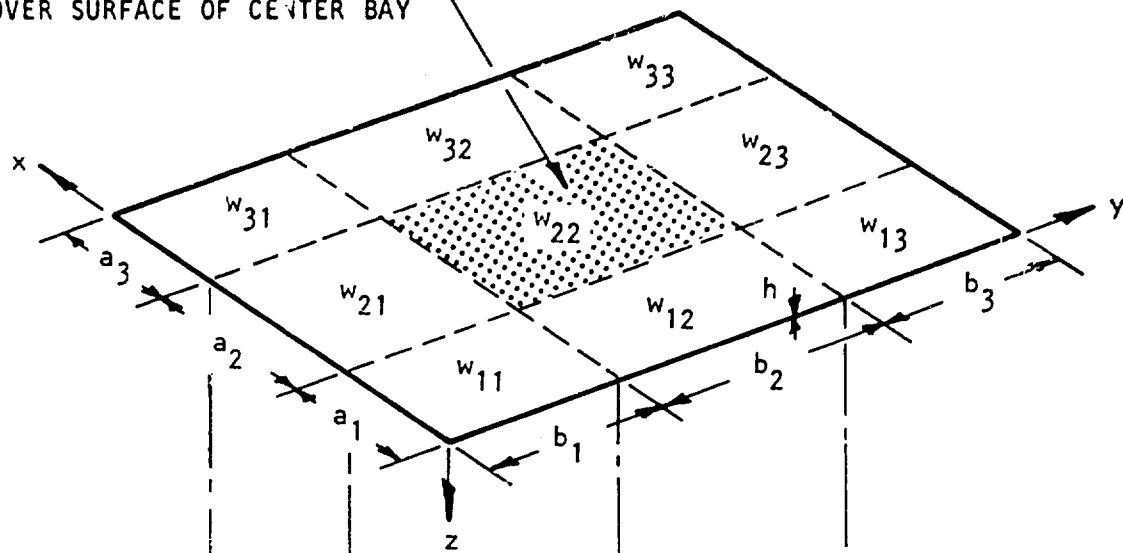
(a) PLATE GEOMETRY
