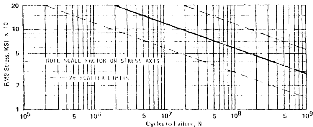
FIGURE 6.6.3-7 COUPON S-N DATA FOR COMMERCIALY PURE TITANIUM ALLOY WITH SPOT WELDED JOINTS
