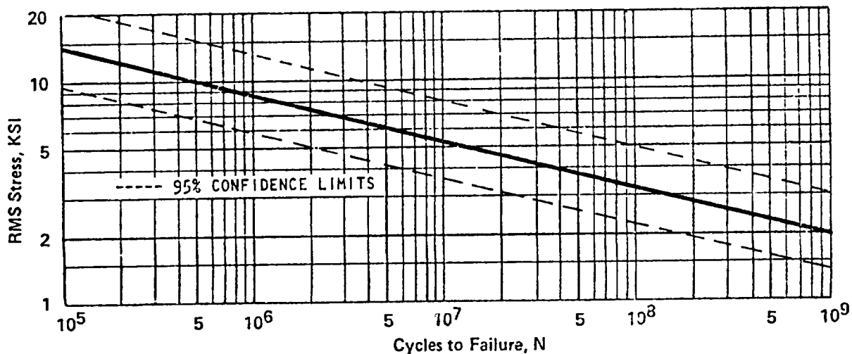
FIGURE 6.5.1-10 S-N DATA FOR 7075-T6 SHEET WITH CUT COUNTERSUNK RIVETED JOINTS - STIFFENED PANEL SONIC FATIGUE TEST SPECIMENS
