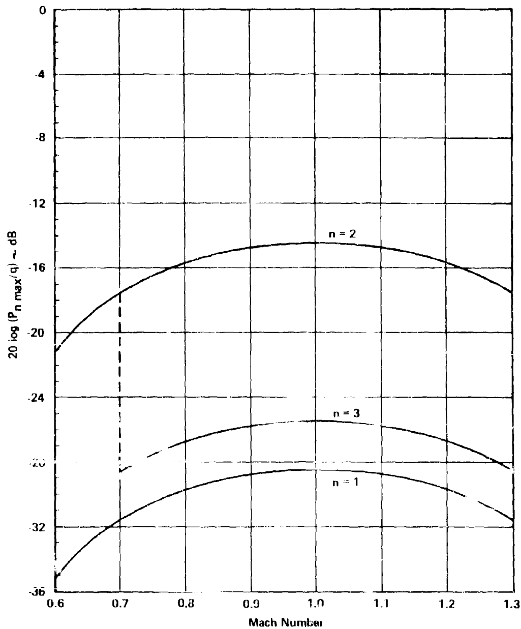
FIGURE 4.3.2-2 VARIATION OF MODAL PEAK AMPLIFICATION WITH MACH NUMBER FOR FIRST THREE MODES ( L_x/D = 4.0 )
