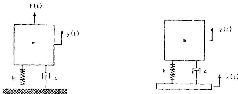
(a) Mechanical System with Force Input, (b) Mechanical System with Foundation Motion Input
